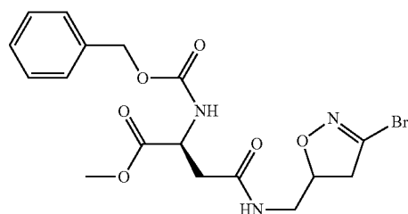
(S)-2-Benzyloxycarbonylamino-N-(3-bromo-4,5-dihydro-isoxazol-5-ylmethyl)-succinamic acid methyl ester
