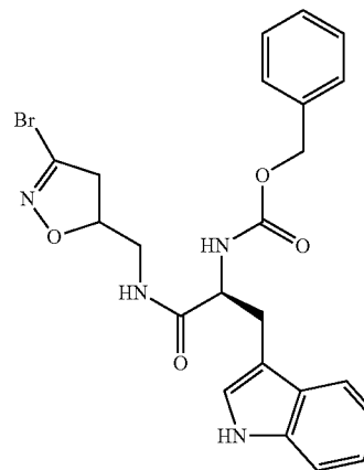
{(S)-1-[(3-Bromo-4,5-dihydro-isoxazol-5-ylmethyl)-carbamoyl]-2-(1H-indol-3-yl)-ethyl)-carbamamic acid benzyl ester
