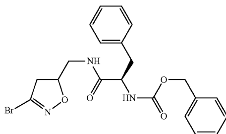
{(R)-1-[(3-Bromo-4,5-dihydro-isoxazol-5-ylmethyl)-carbamoyl]-2-phenyl-ethyl)-carbamamic acid benzyl ester
