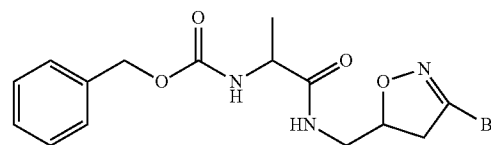
{(S)-1-[(3-Bromo-4,5-dihydro-isoxazol-5-ylmethyl)-carbamoyl]-ethyl}-carbamic acid benzyl ester
