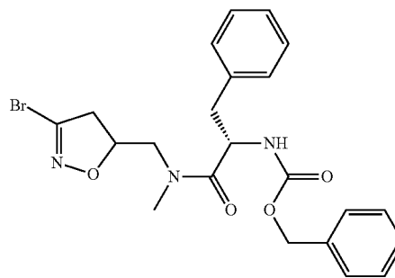
{(S)-1-[(3-Bromo-4,5-dihydro-isoxazol-5-ylmethyl)-methyl-carbamoyl]-2-(4-hydroxy-phenyl)-ethyl)-carbamamic acid benzyl ester
