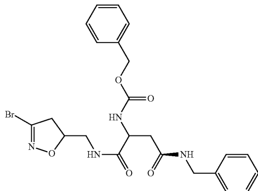
{(S)-2-Benzylcarbamoyl-1-[(3-Bromo-4,5-dihydro-isoxazol-5-ylmethyl)-carbamoyl]-ethyl)-carbamamic acid benzyl ester
