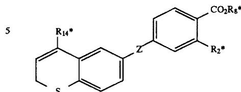
Formula 4
