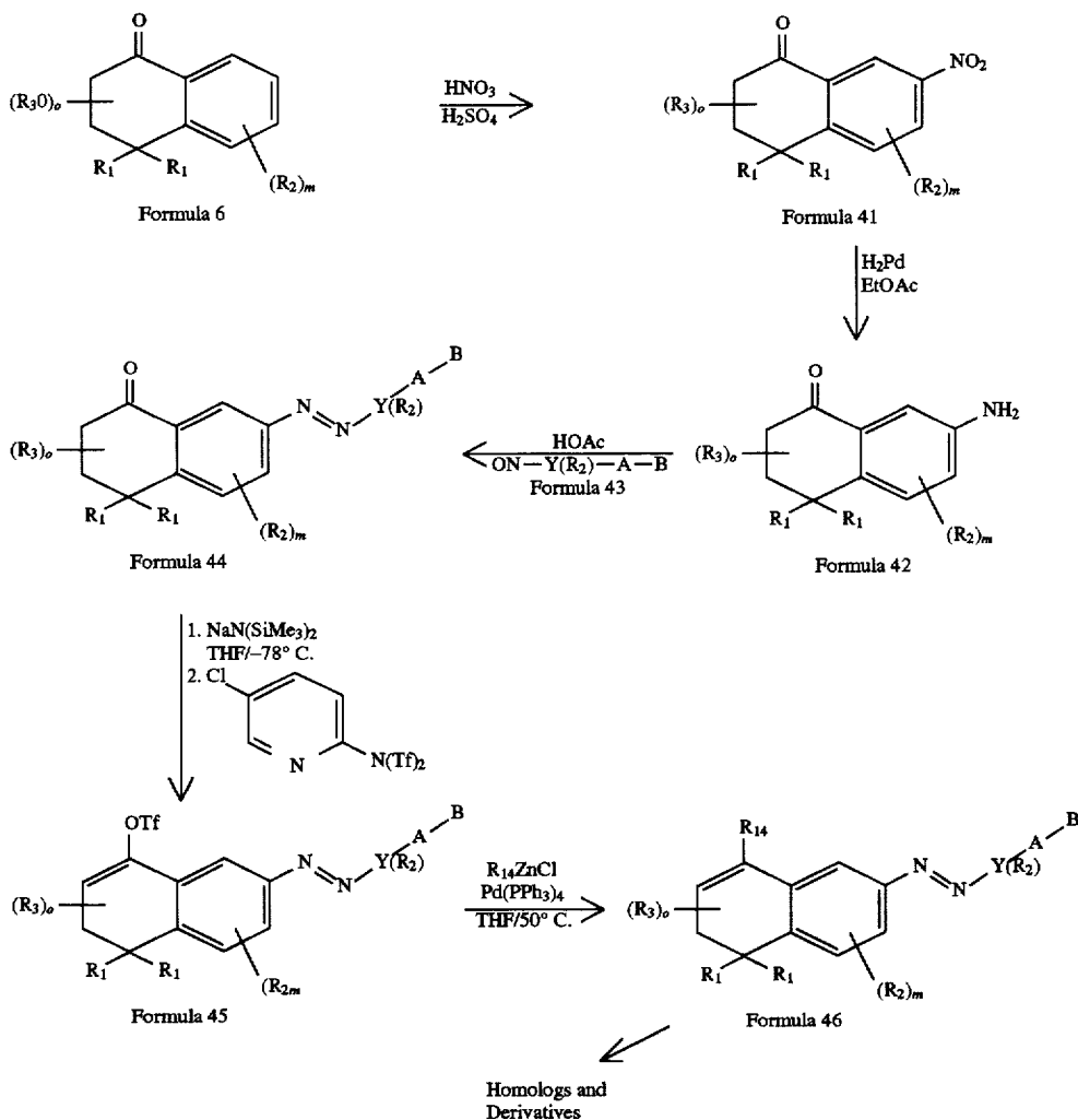
Reaction Scheme 5
