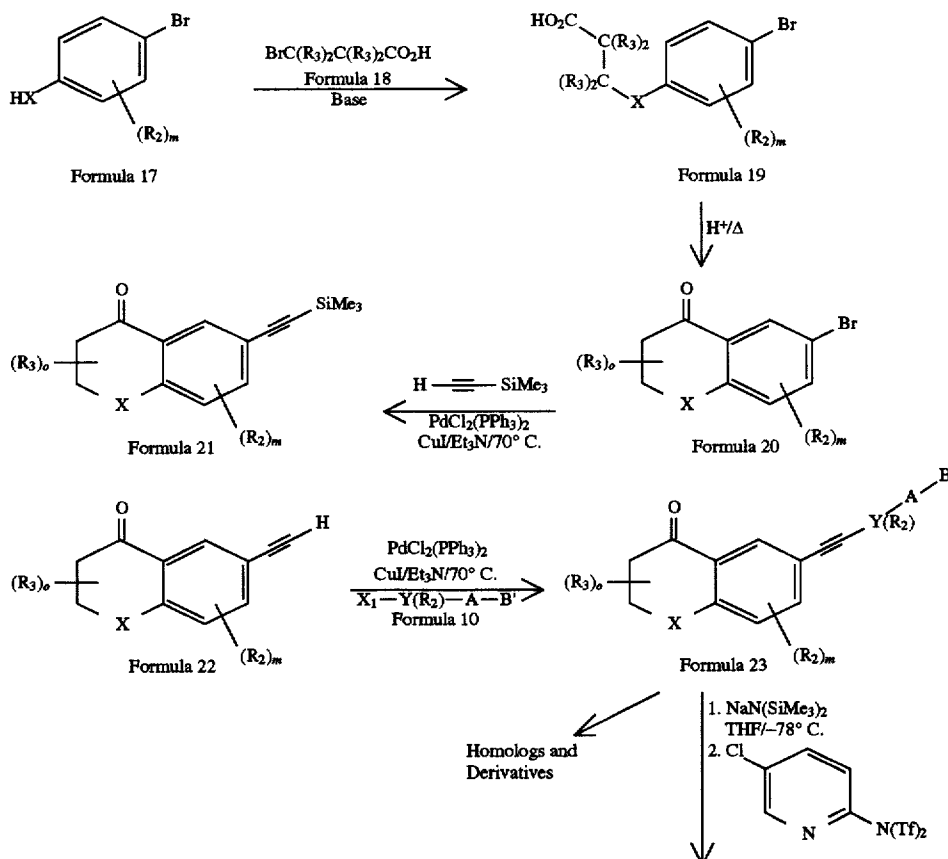
Reaction Scheme 2
