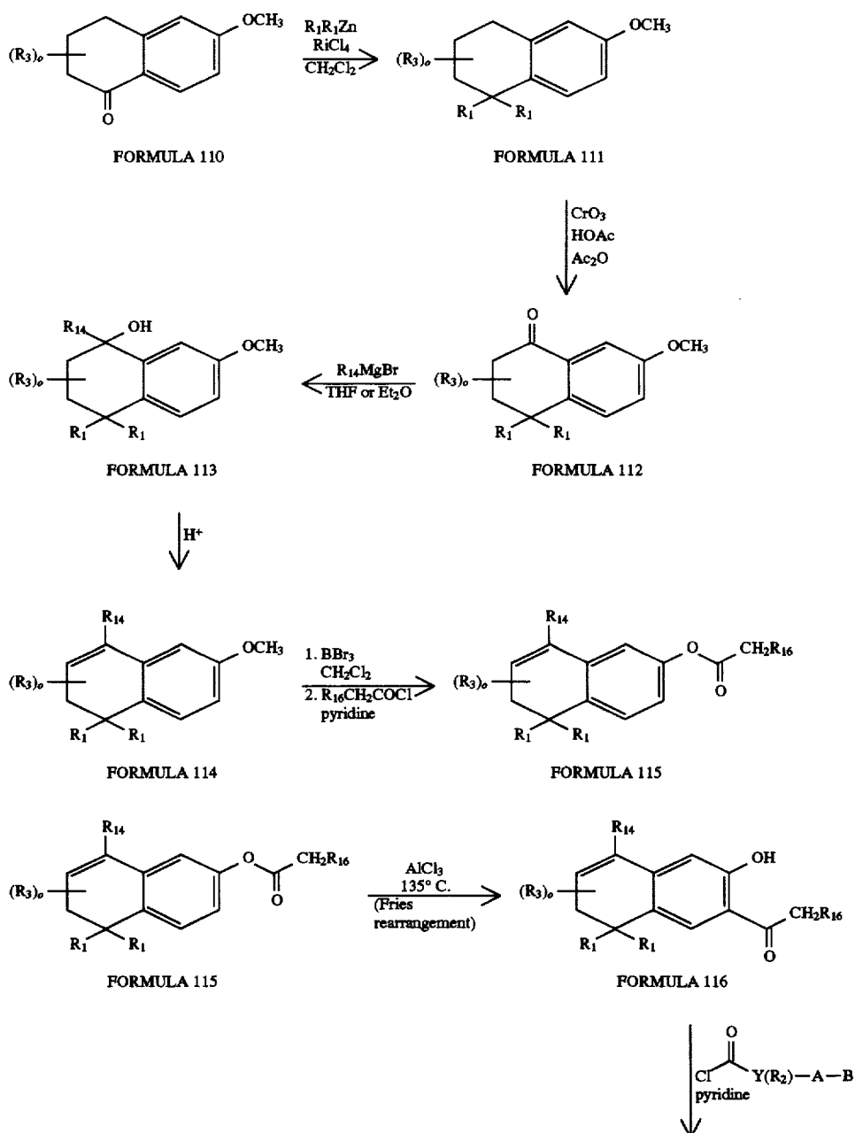
Reaction Scheme 102
