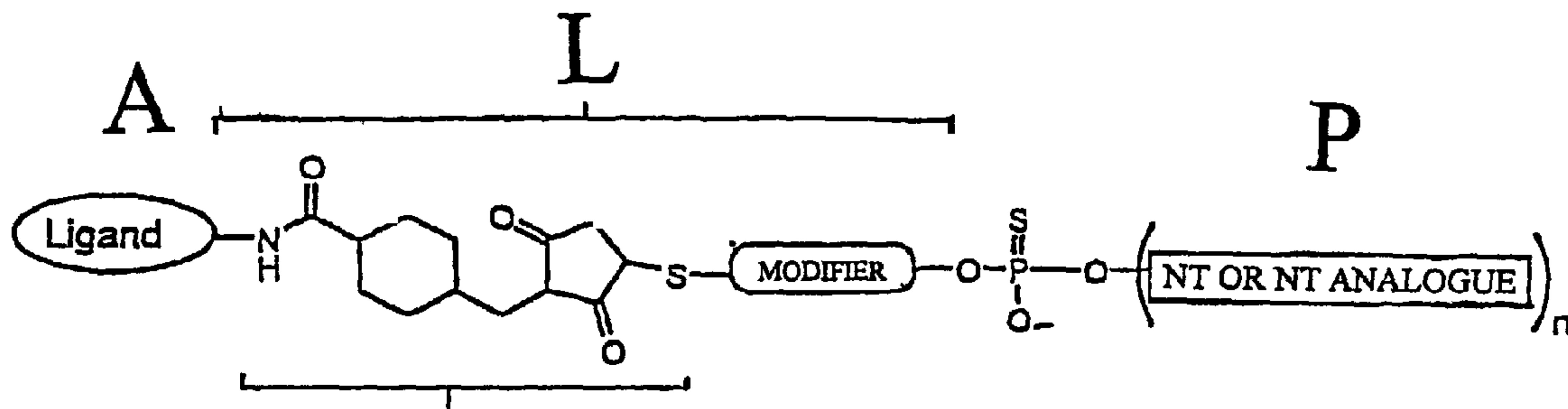
CROSS-LINKING REAGENT
