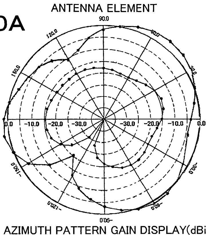
ANTENNA ELEMENT + PARASITIC ELEMENT FIG.10B
