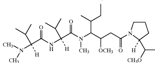
1a, Dolastatin 10 (Dov-Val-Dil-Dap-Doe)
