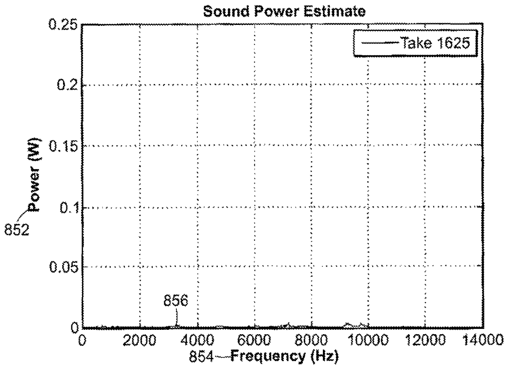
FIG. 8 (Prior Art)
