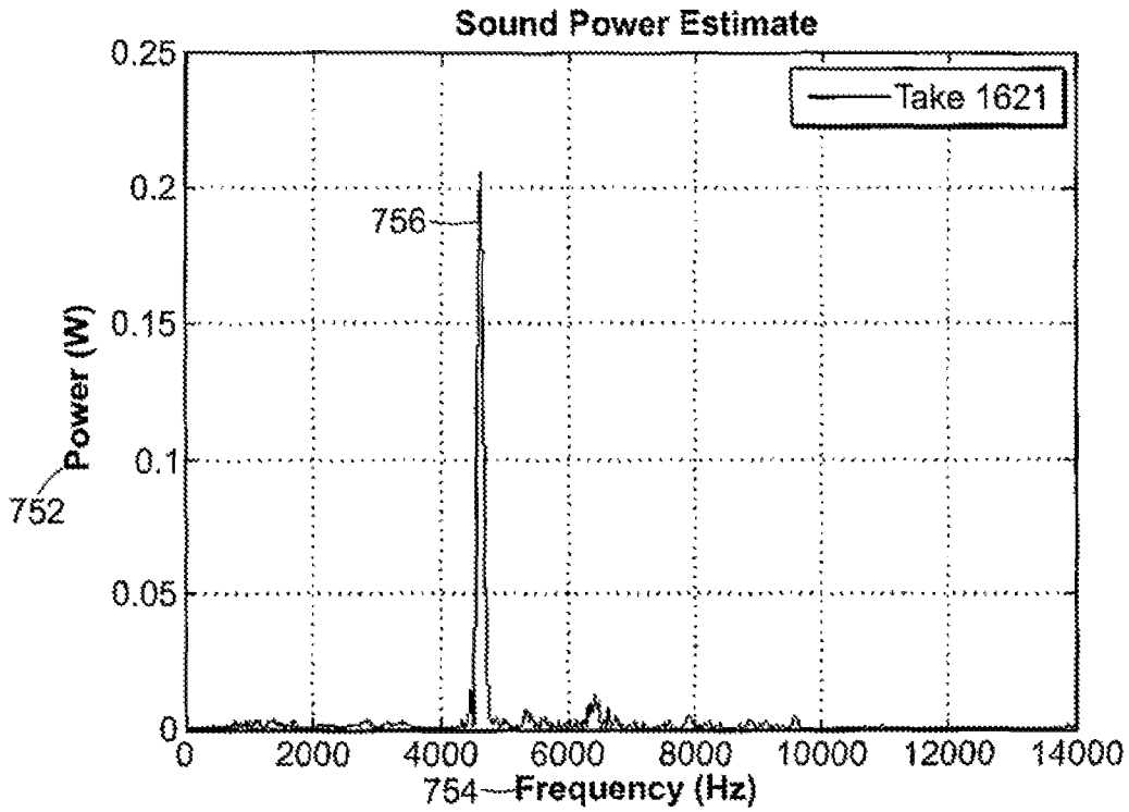
FIG. 7 (Prior Art)
