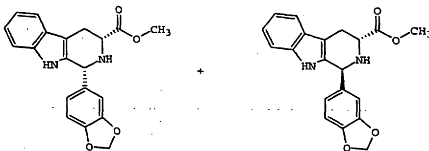
Compound (II) ( cis -isomer) (42% yield) (desired)
