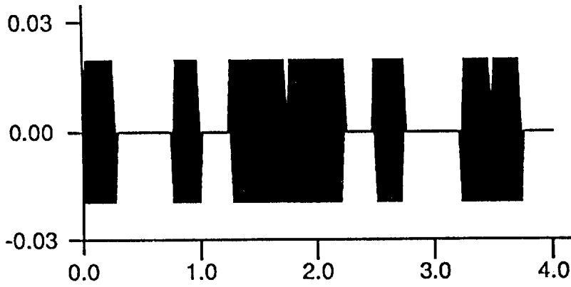
AMPLITUDE ON-OFF PLUS BIPHASE CARRIER MODULATION [1 + PN_1(t)] \cos[\omega_0 t + \pi/2 PN_2(t)]
