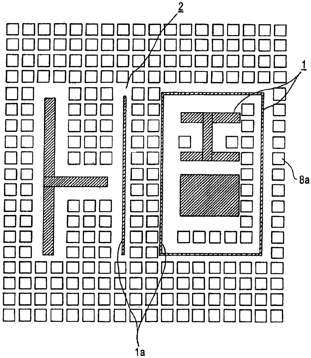
FIG. 12 (PRIOR ART)
