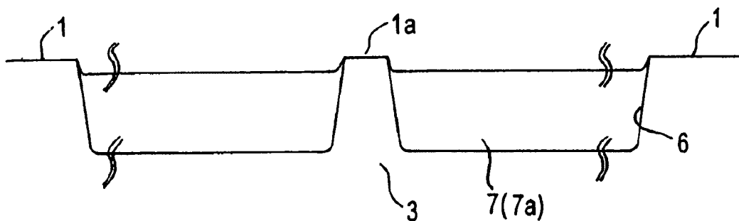
FIG. 11 (PRIOR ART)
