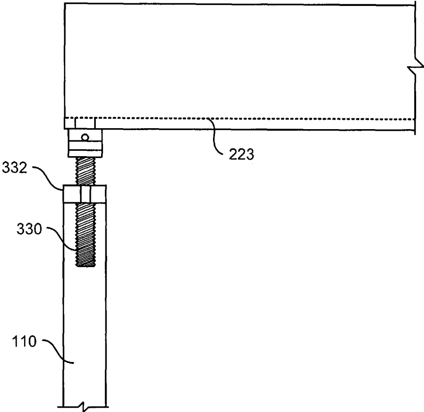
02 DETAIL S1 SCALE: 3/4" - 1'-0"
