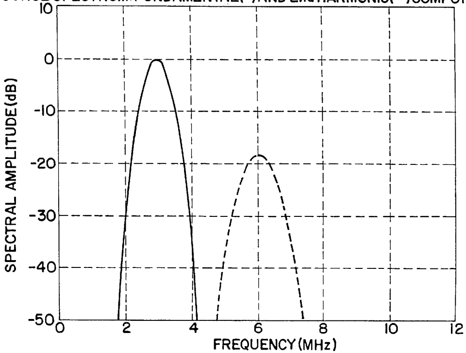
SOURCE SPECTRUM: FUNDAMENTAL(-) AND 2nd HARMONIC(-) COMPONENTS
