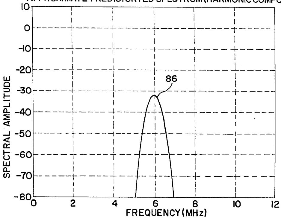
APPROXIMATE PREDISTORTED SPECTRUM (HARMONIC COMPONENT)
