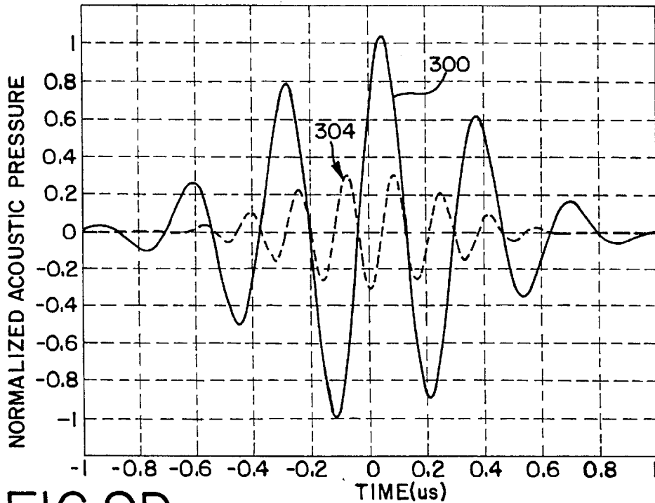
SOURCE WAVEFORM: FUNDAMENTAL (—) AND 2nd HARMONIC (---) COMPONENTS
