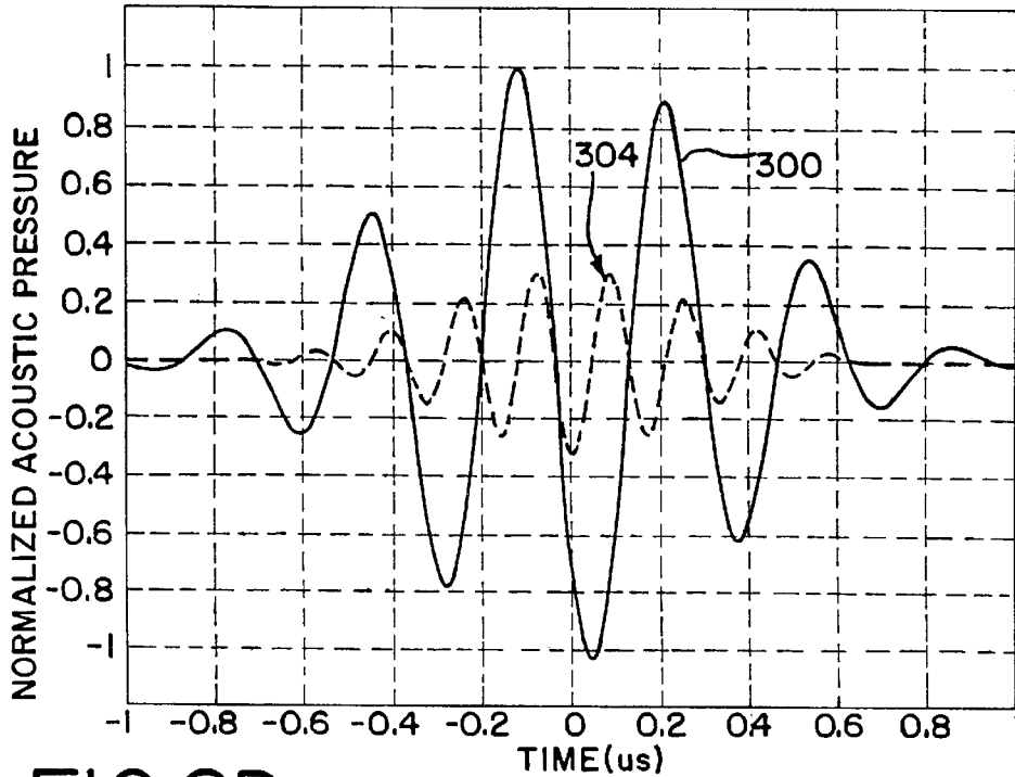
SOURCE WAVEFORM: FUNDAMENTAL(-) AND 2nd HARMONIC(-) COMPONENTS
