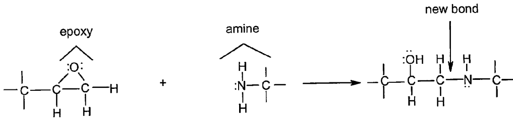
FIGURE 4: REACTIONS OF EPOXY GROUPS
