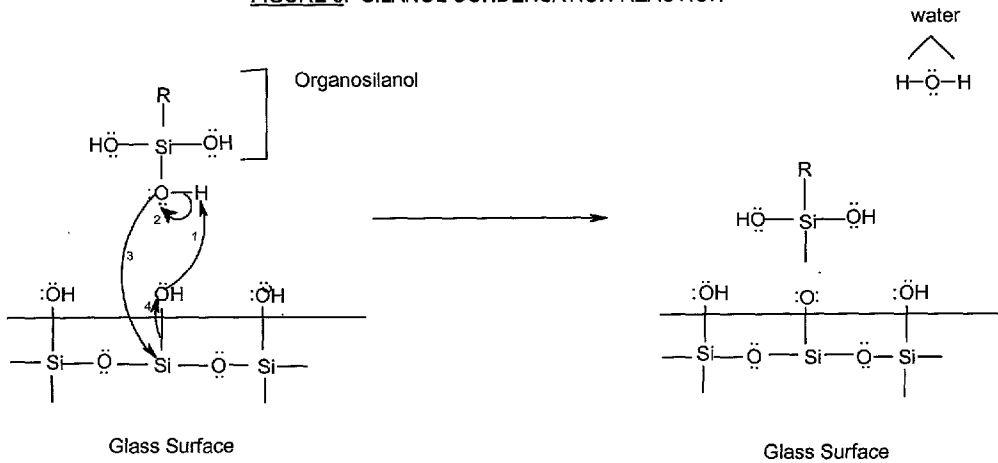
FIGURE 3: SILANOL CONDENSATION REACTION
