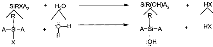
FIGURE 2: HYDROLYSIS OF AN ORGANOSILANE TO PRODUCE AN ORGANOSILANOL
