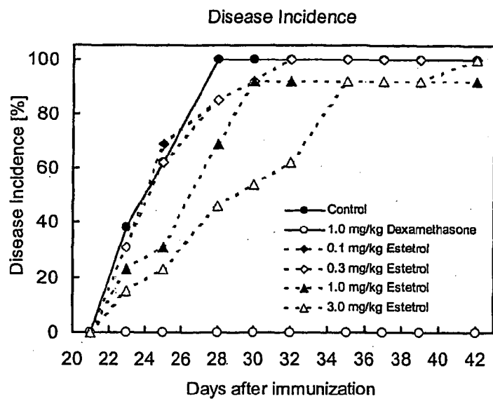
Figure 6: Effect of treatment with estetrol on disease incidence in mouse CIA., showing the incidence of disease for all studied treatment groups versus time. "Disease" was defined as a macroscopic arthritis score of > 0.
