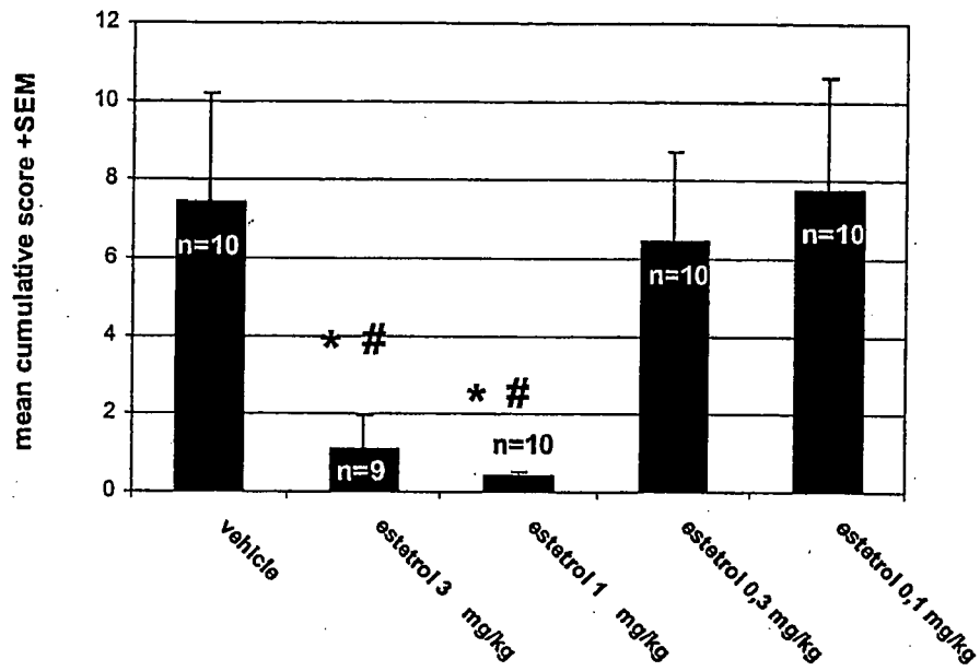
Figure 5: Effect of treatment with estetrol on the cumulative clinical EAE score in the relapsing phase (day 26-42) in SJL/J mice.
