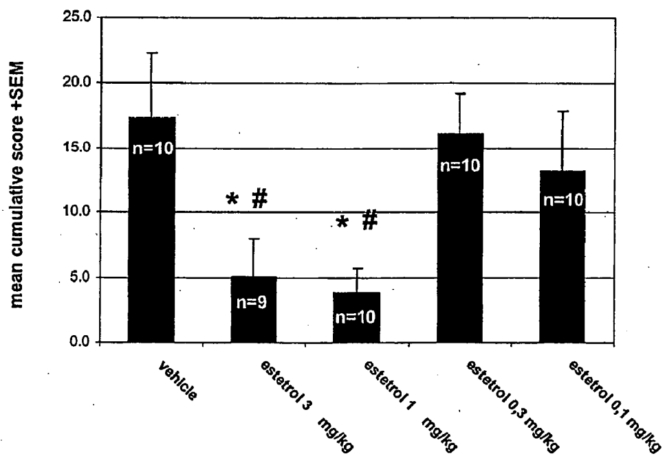
Figure 4: Effect of treatment with estetrol on the cumulative clinical EAE score (day 0-42) in SJL/J mice.
