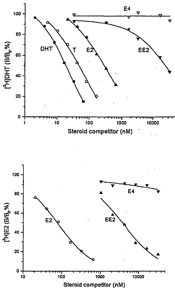
Figure 1: Competitive displacement of [ 3 H]DHT (panel A) and [ 3 H]estradiol (panel B) from the human sex hormone-binding globulin steroid binding site. The unlabeled steroid ligands used as competitors were as follows: estetrol (E4), 17 \alpha -ethinylestradiol (EE2), 17 \beta -estradiol (E2), testosterone (T) and 5 \alpha -dihydrotestosterone (DHT)
