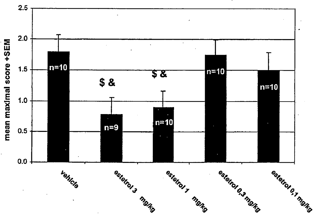
Figure 3: Effect of treatment with estetrol on the maximal EAE score in SJL/J mice.
