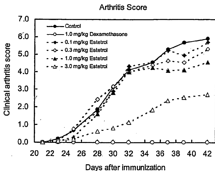
Figure 7: Effect of treatment with estetrol on macroscopical arthritis score in mouse CIA. Each point represents the group mean (n=13).
