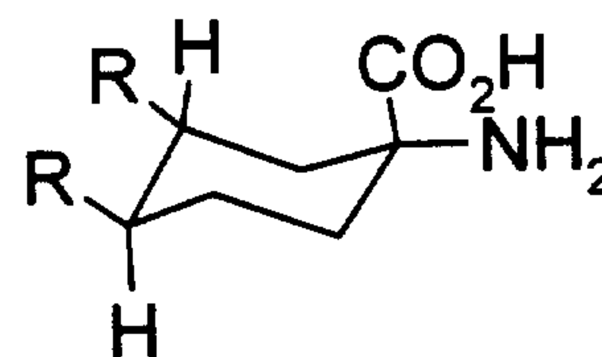
Strecker synthesis ( \alpha -isomer)
