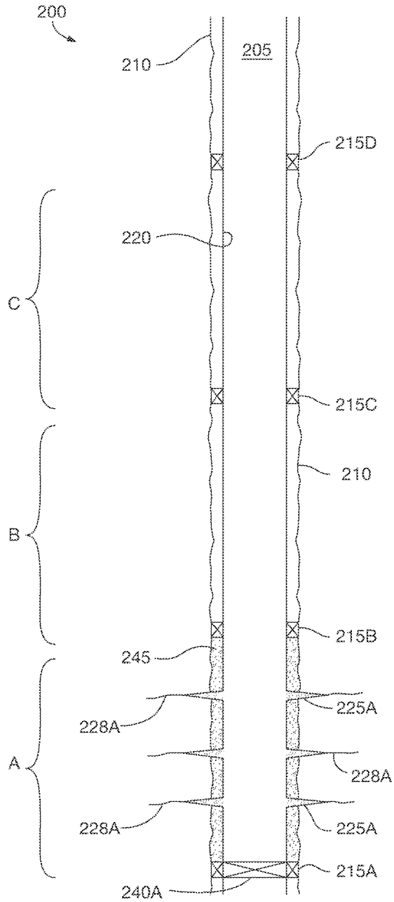
FIG. 2C Prior Art
