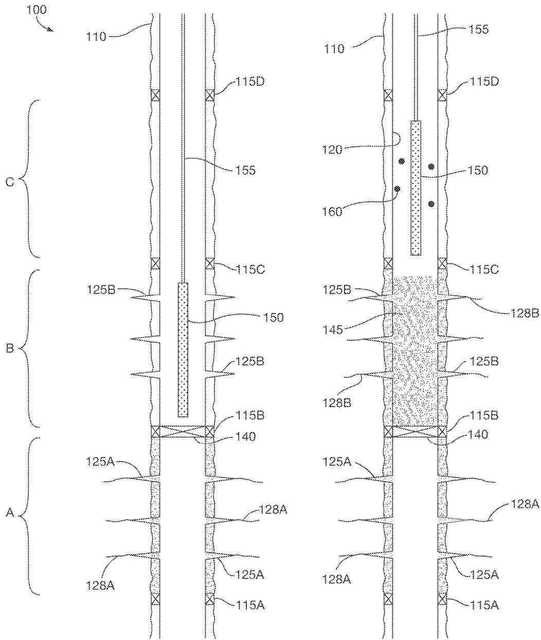
FIG. 1C Prior Art
