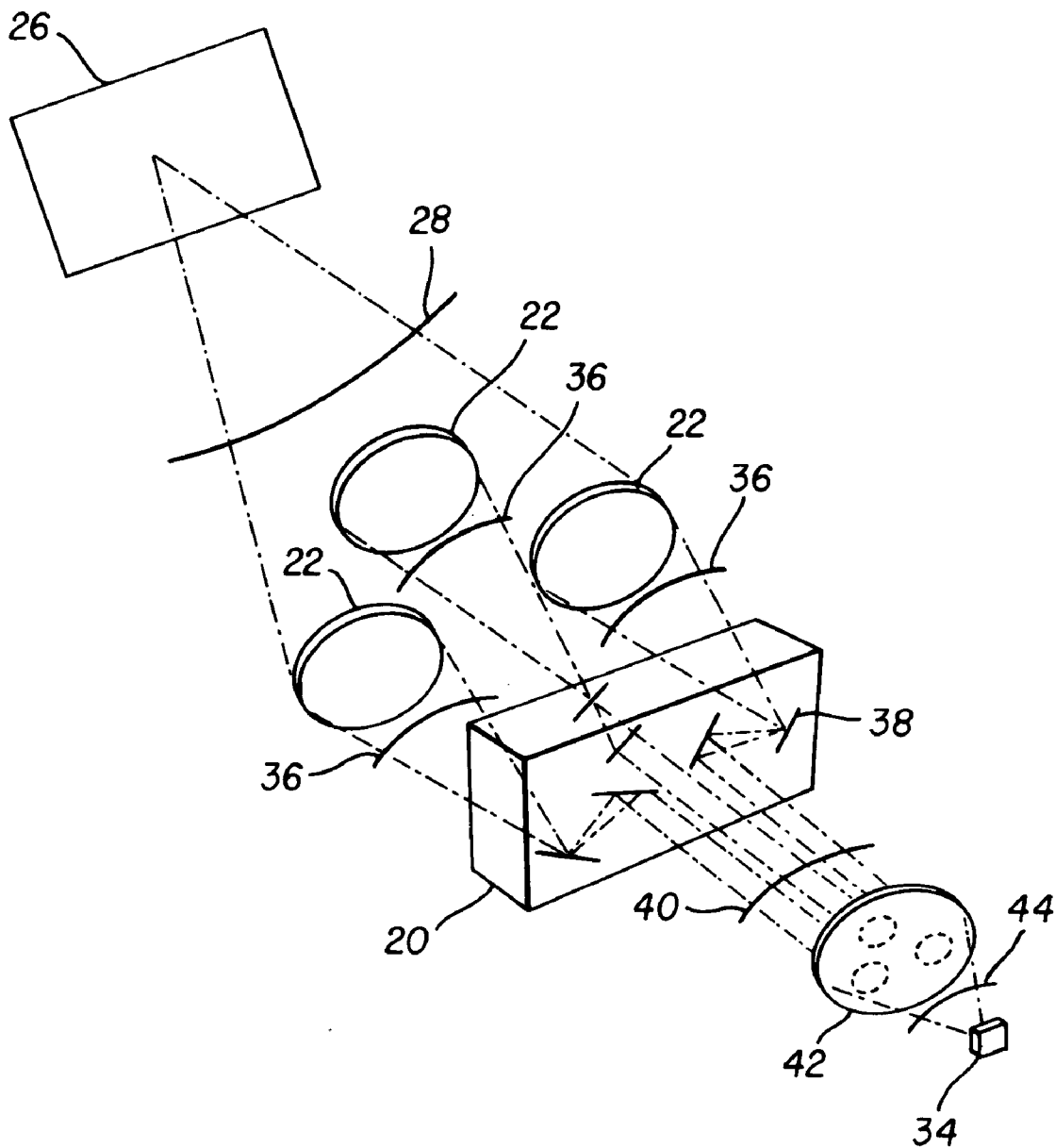
FIG. 4 (Prior Art)
