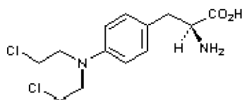
4-Bis(2-chloroethyl)amino-L-phenylalanine
