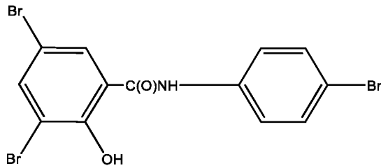
tribromosalalan
