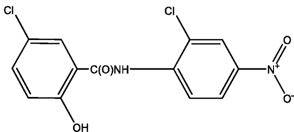
niclosamide
