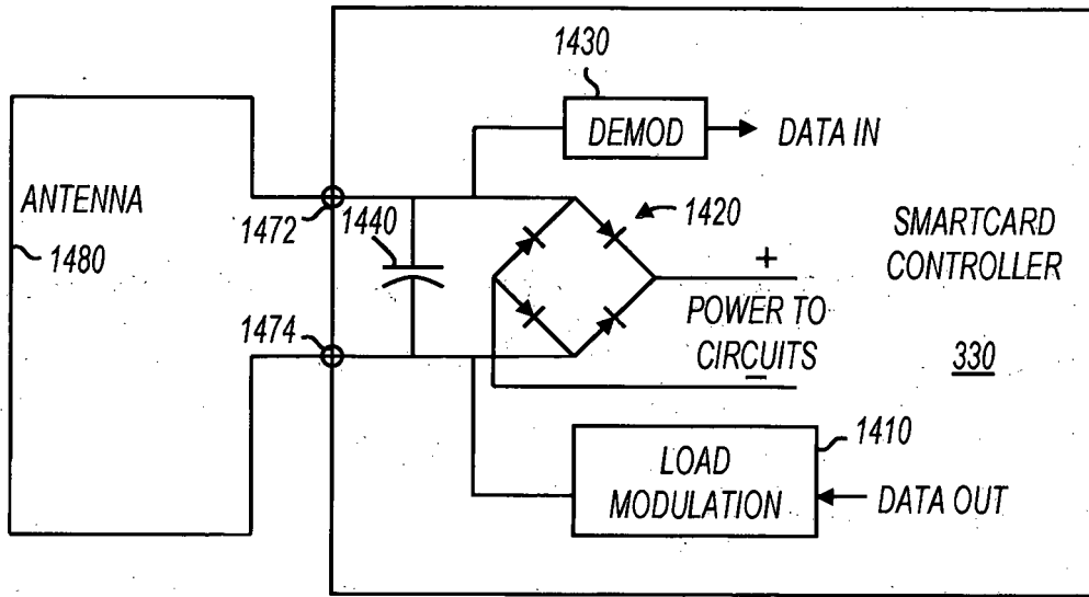
FIG. 14 (PRIOR ART)
