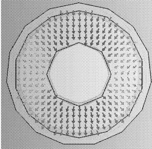
HE11, Horizontal Polarization
