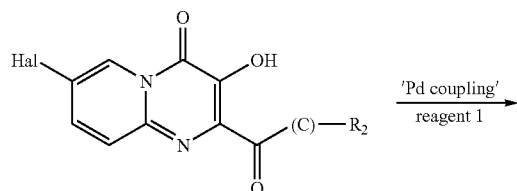
Further reactions: Scheme 4
