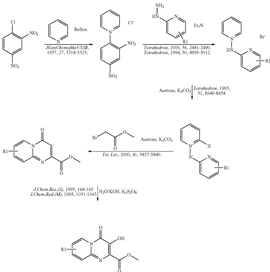
General Scheme 2: Alternate Synthesis 1
