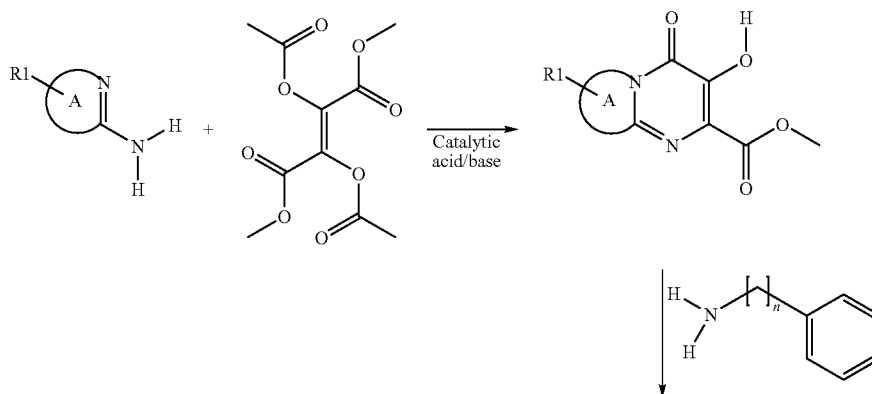
General Scheme 1: Synthesis
