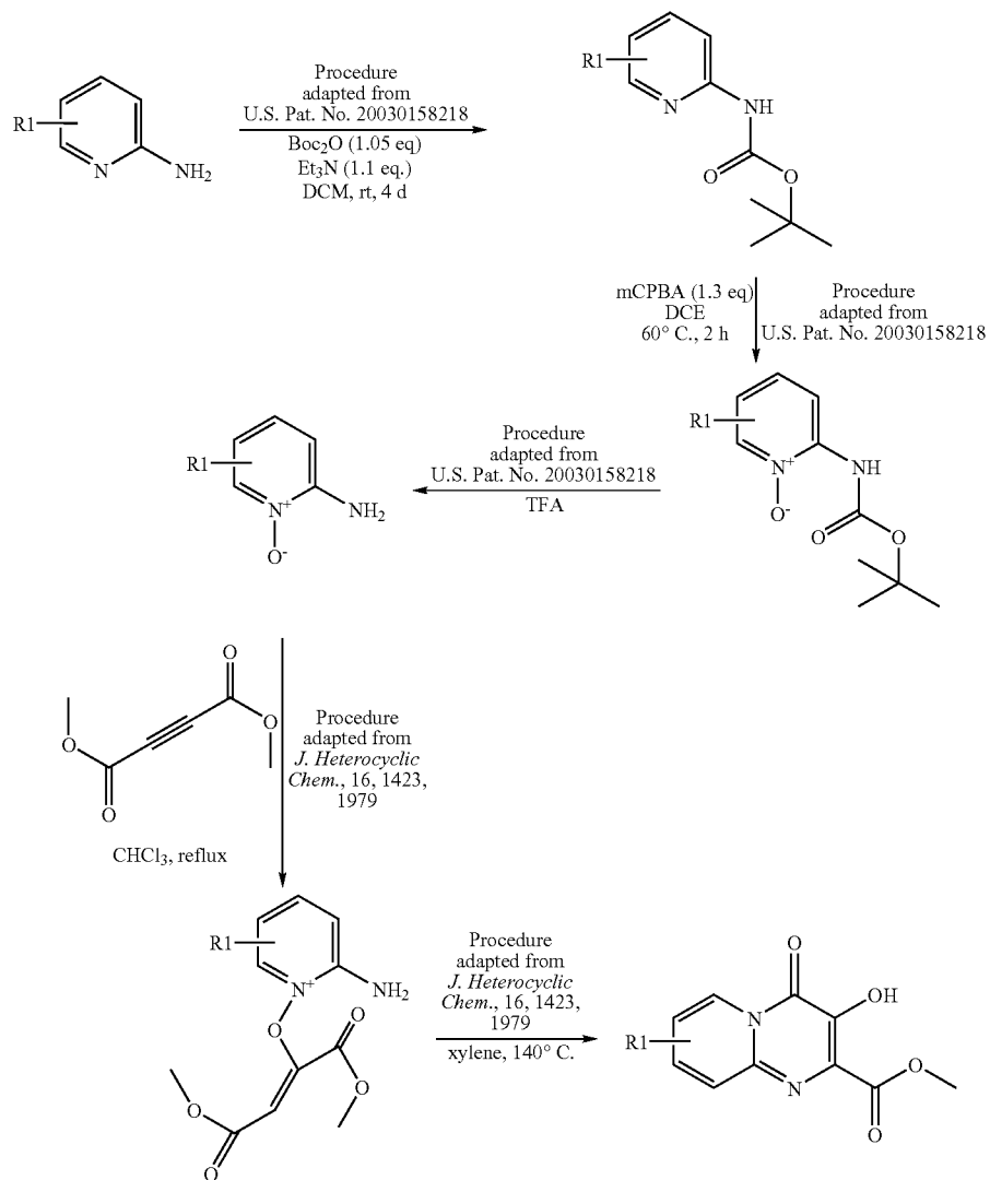
General Scheme 3: Alternate Synthesis 2
