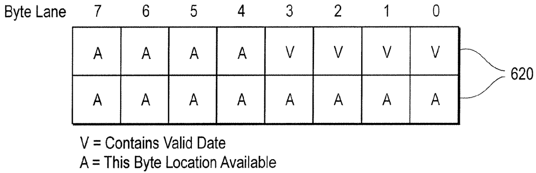
FIG. 5B Cell Buffer before Host Read
