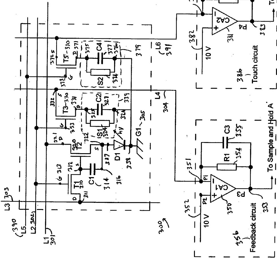
Charge Amp Transimpedance amplifiers
