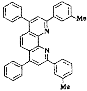
Compound No. 30
