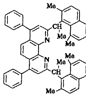
Compound No. 166
