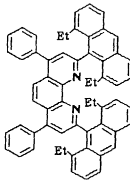
Compound No.130
