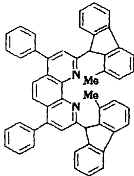
Compound No. 135
