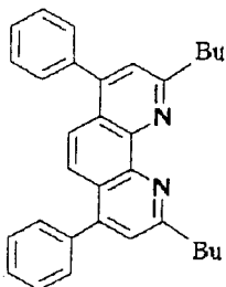
Compound No. 4
