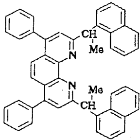
Compound No. 163
