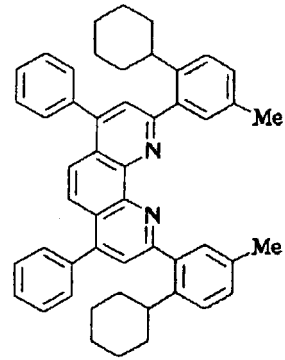
Compound No. 80
