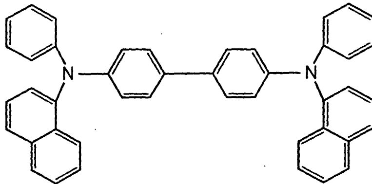
STRUCTURAL FORMULA OF \alpha -NAPHTHYLPHENYLDIAMINE ( \alpha -NPD)
