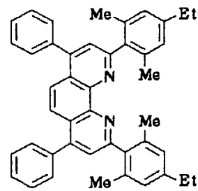
Compound No. 71
