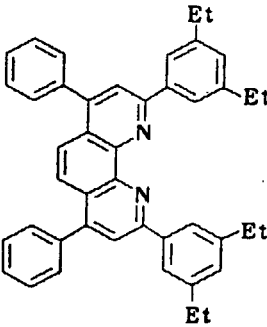
Compound No. 47
