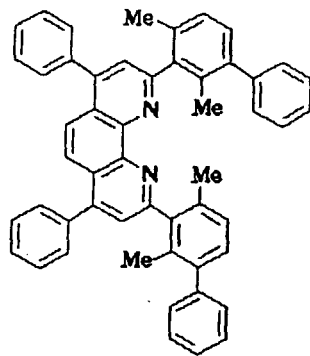
Compound No. 109
