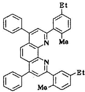
Compound No. 69
