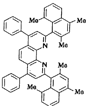
Compound No.119
