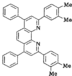
Compound No. 35
