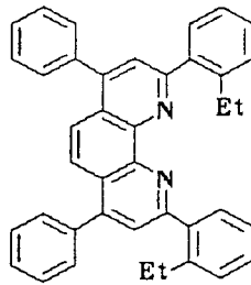
Compound No. 41
