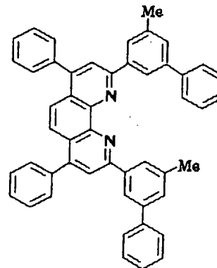
Compound No. 108
