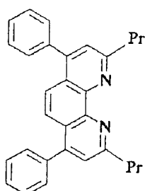
Compound No. 2
