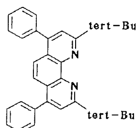
Compound No. 6
