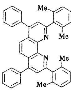
Compound No. 32
