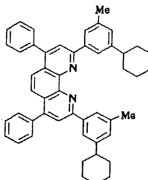
Compound No. 88
