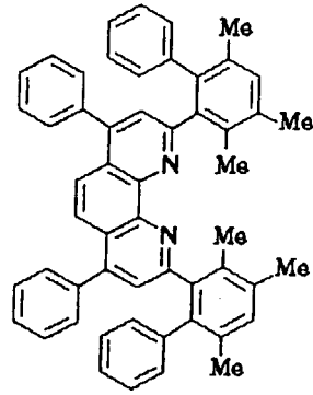
Compound No. 104
