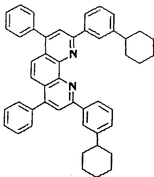
Compound No. 85
