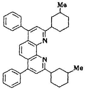
Compound No. 16
