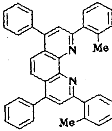
Compound No. 29
