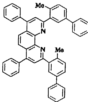
Compound No. 107
