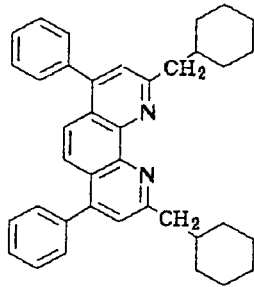
Compound No. 171
