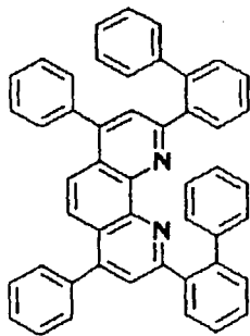
Compound No. 95
