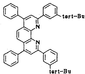
Compound No. 54
