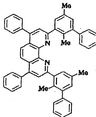
Compound No. 112
