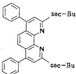
Compound No. 5
