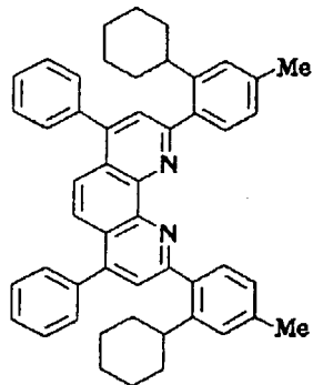
Compound No. 79
