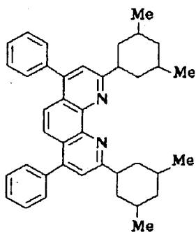
Compound No. 23
