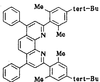
Compound No. 74
