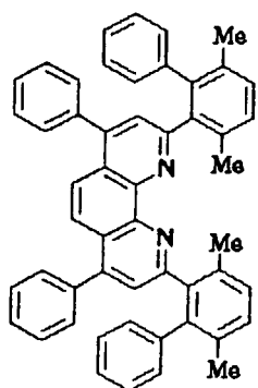
Compound No. 101
