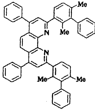
Compound No. 113
