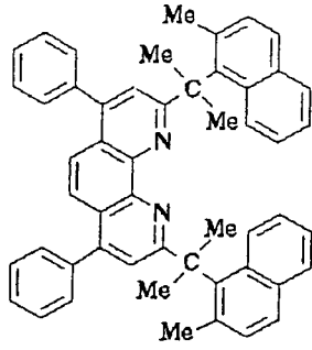
Compound No. 169
