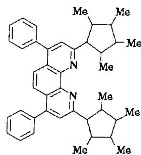
Compound No. 12
