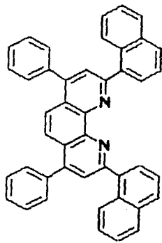
Compound No. 115
