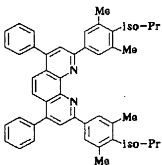
Compound No. 77
