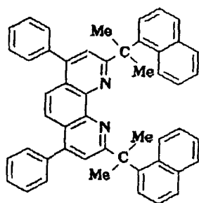
Compound No. 167
