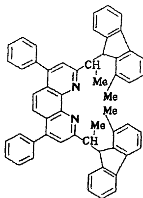
Compound No. 177
