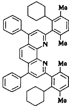
Compound No. 81
