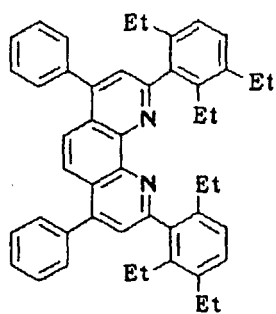
Compound No. 49
