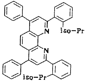
Compound No. 57
