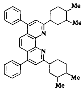
Compound No. 24
