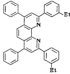
Compound No. 42
