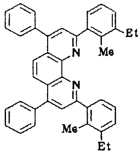
Compound No. 67
