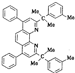
Compound No. 157
