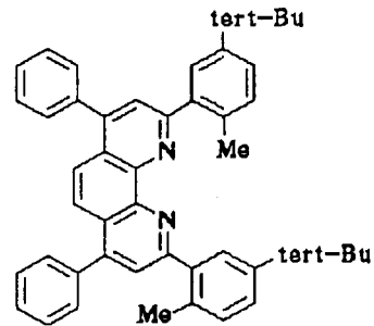
Compound No. 72
