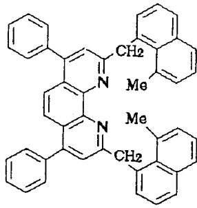
Compound No. 161
