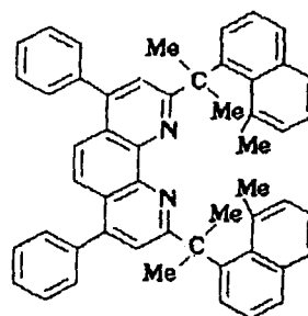
Compound No. 168
