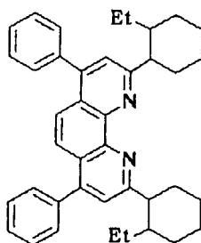
Compound No. 20
