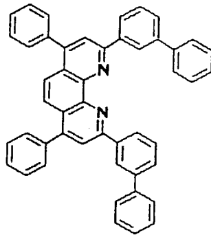
Compound No. 105
