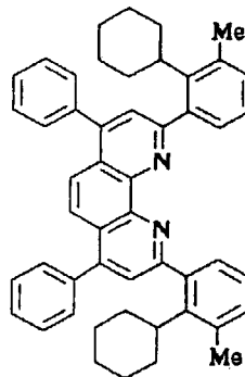
Compound No. 80
