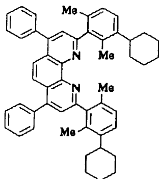
Compound No. 89
