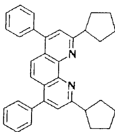
Compound No. 8
