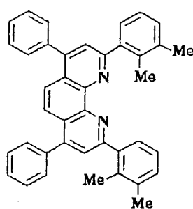
Compound No. 36
