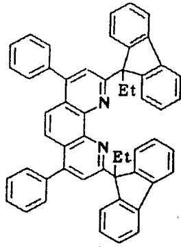
Compound No. 137
