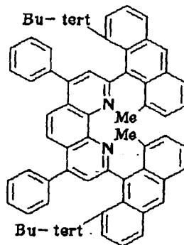
Compound No.132
