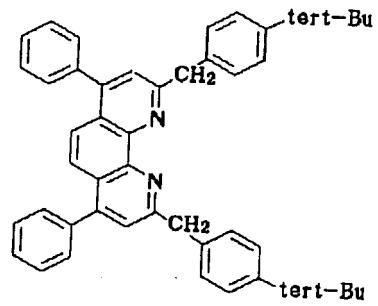
Compound No. 148
