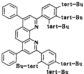
Compound No. 65
