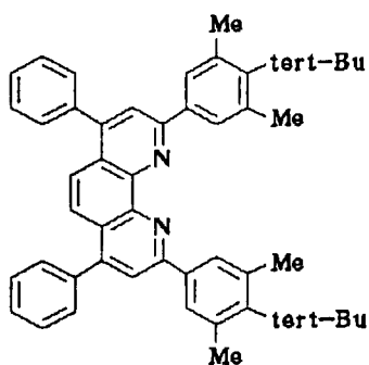
Compound No. 75
