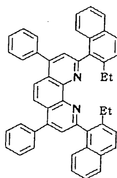
Compound No.120
