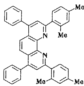
Compound No. 33
