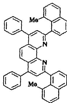
Compound No. 116
