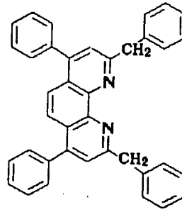
Compound No. 138
