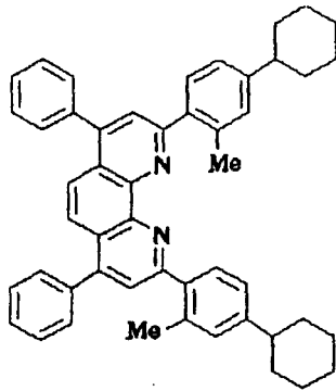
Compound No. 91
