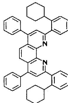
Compound No. 78
