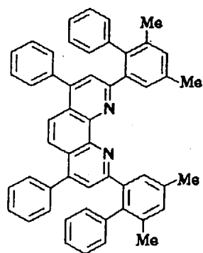
Compound No. 102
