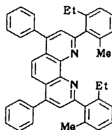
Compound No. 66
