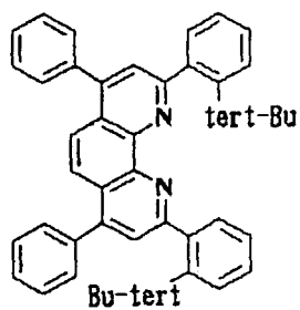
Compound No. 53
