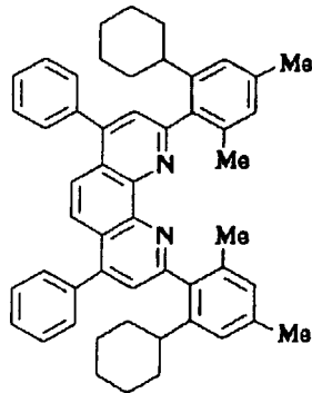
Compound No. 82
