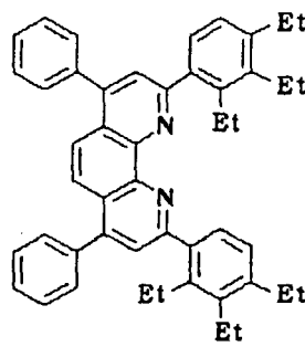
Compound No. 50
