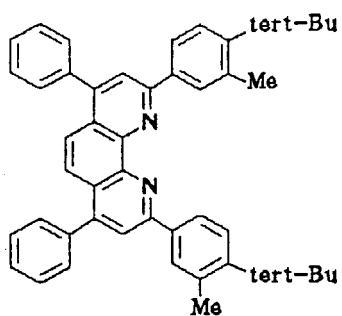
Compound No. 73
