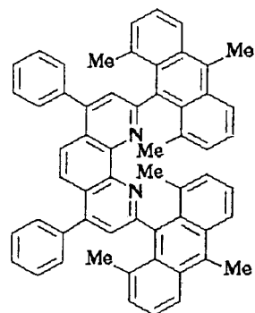
Compound No. 128
