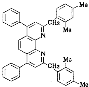
Compound No. 144
