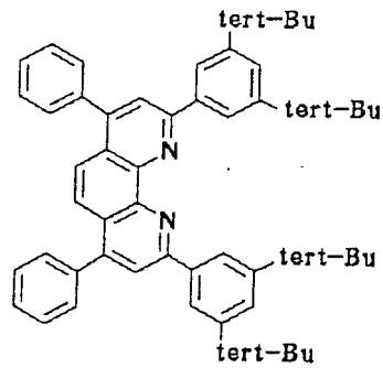
Compound No. 60
