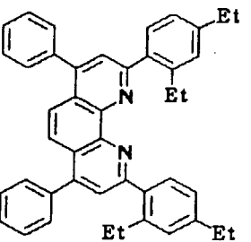
Compound No. 46
