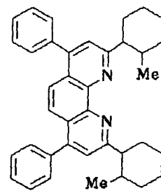
Compound No. 15
