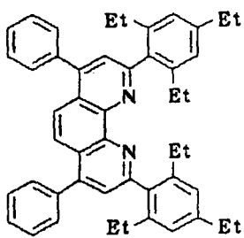
Compound No. 51
