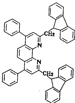
Compound No. 173
