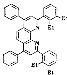
Compound No. 45
