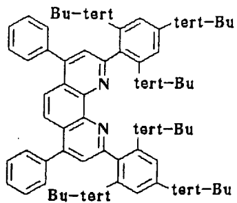
Compound No. 62
