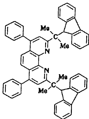
Compound No. 175
