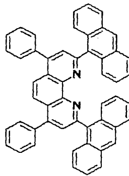
Compound No. 124
