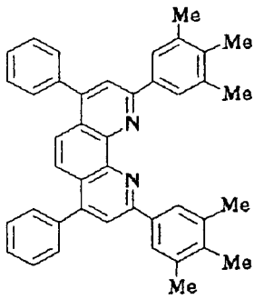
Compound No. 40
