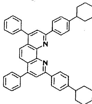
Compound No. 88
