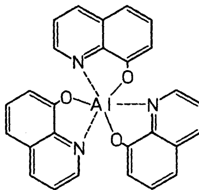
STRUCTURAL FORMULA OF Alq 3
