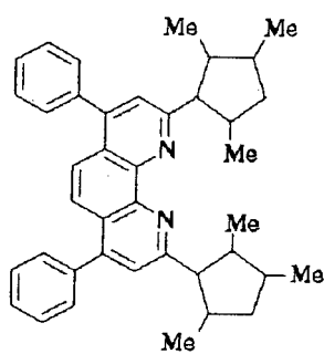
Compound No. 11
