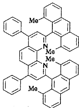
Compound No. 127
