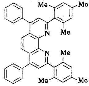
Compound No. 39
