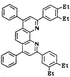
Compound No. 48
