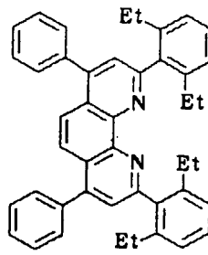
Compound No. 44
