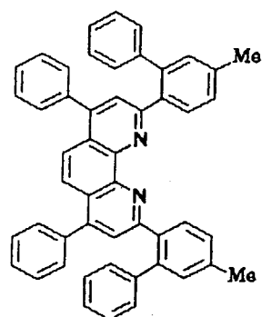
Compound No. 100
