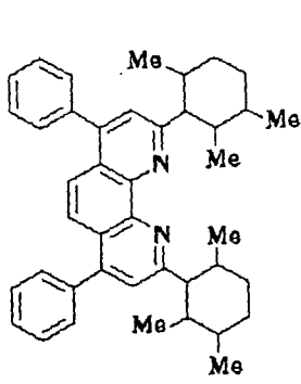
Compound No. 25
