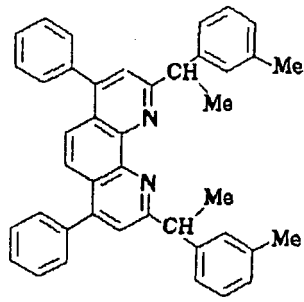
Compound No. 149
