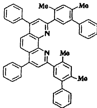
Compound No. 111
