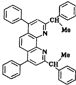
Compound No. 139
