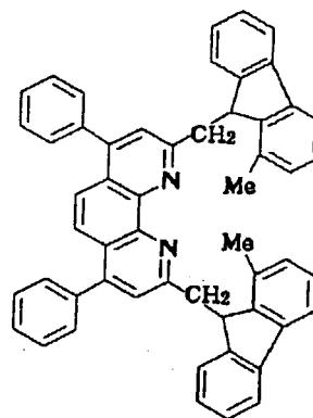
Compound No. 176
