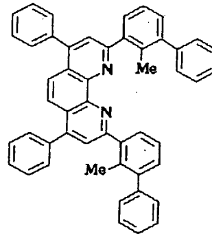
Compound No. 106
