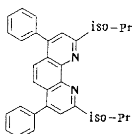
Compound No. 3
