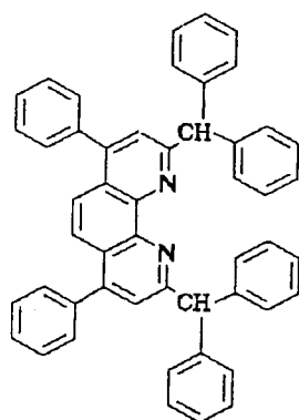
Compound No. 159
