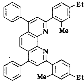
Compound No. 68
