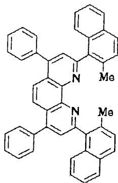
Compound No.117
