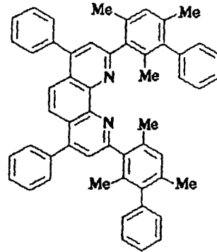
Compound No. 114
