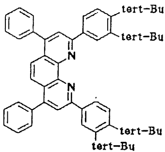
Compound No. 61
