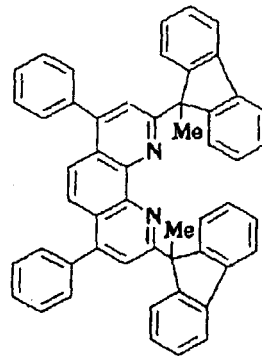
Compound No. 134
