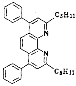
Compound No. 13
