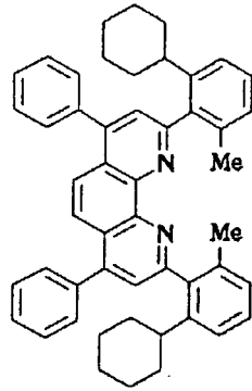
Compound No. 79
