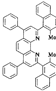
Compound No. 126
