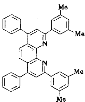
Compound No. 34
