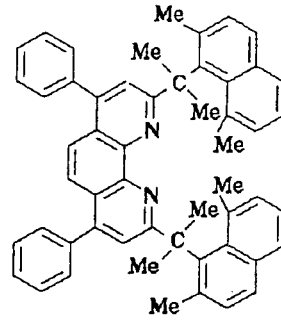
Compound No. 170
