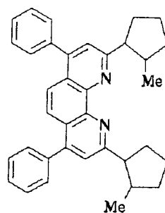
Compound No. 9
