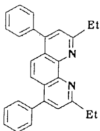
Compound No. 1
