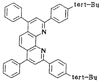
Compound No. 55
