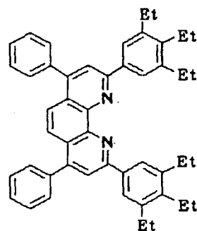
Compound No. 52
