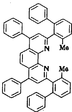
Compound No. 97
