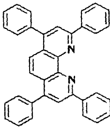
Compound No. 28
