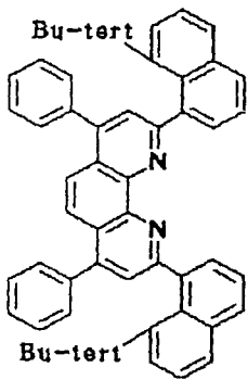
Compound No. 123
