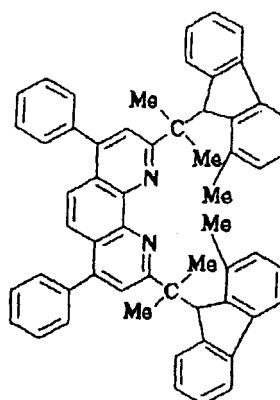
Compound No. 178
