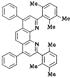
Compound No. 37
