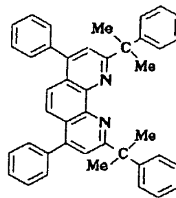
Compound No. 140
