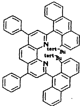
Compound No.131
