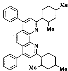
Compound No. 21
