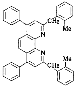
Compound No. 141
