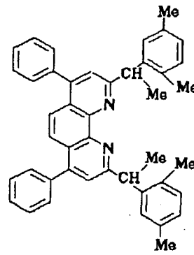
Compound No. 152
