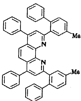
Compound No. 99
