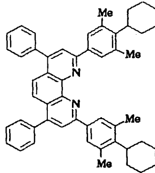
Compound No. 94
