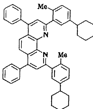
Compound No. 86
