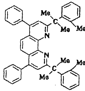
Compound No. 156
