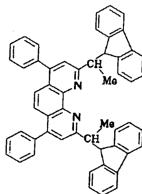
Compound No. 174
