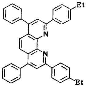
Compound No. 43
