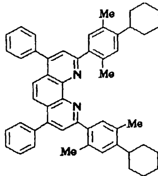
Compound No. 93
