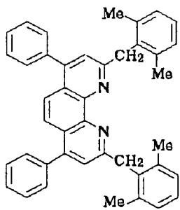
Compound No. 143
