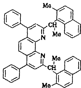
Compound No. 165
