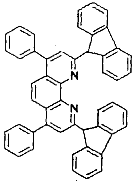
Compound No. 133
