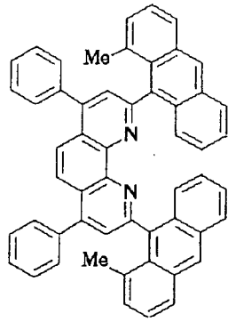
Compound No. 125
