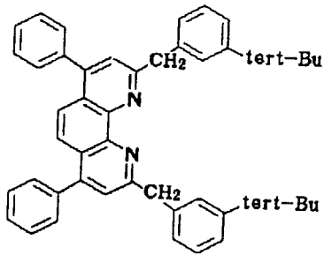
Compound No. 147
