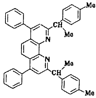
Compound No. 150
