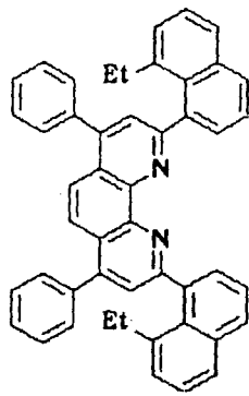
Compound No. 121
