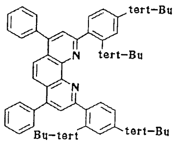
Compound No. 59
