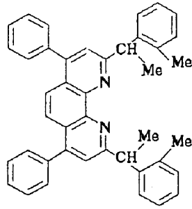
Compound No. 142
