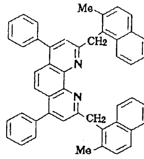
Compound No. 162
