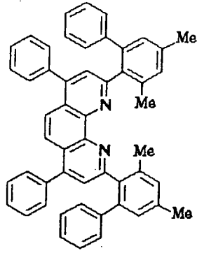
Compound No. 103
