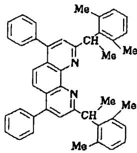
Compound No. 151
