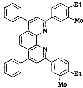
Compound No. 70
