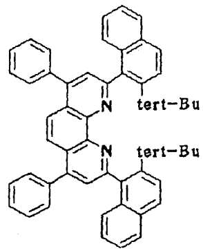
Compound No. 122
