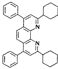
Compound No. 14
