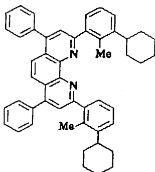
Compound No. 87
