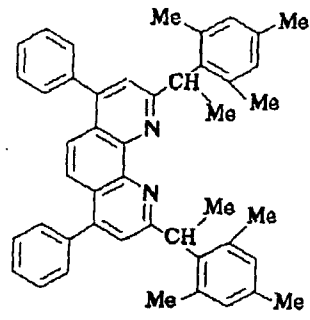
Compound No. 154
