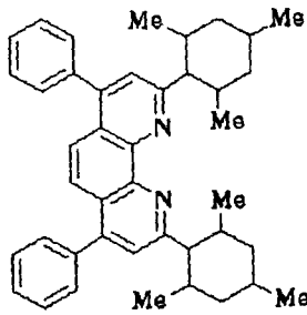
Compound No. 26
