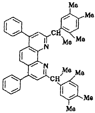
Compound No. 155
