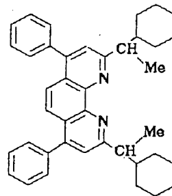
Compound No. 172
