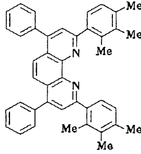
Compound No. 38
