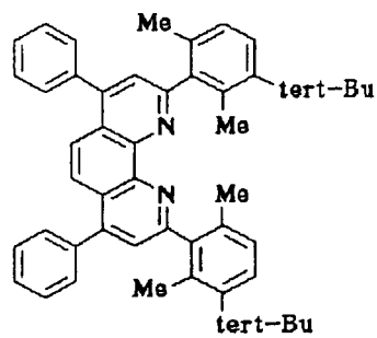
Compound No. 76
