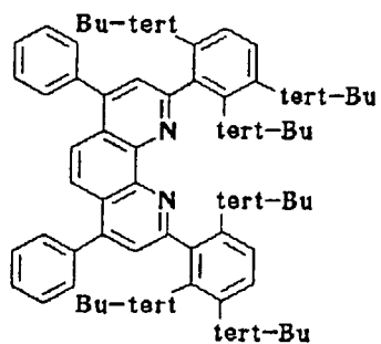
Compound No. 64
