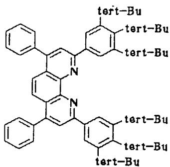
Compound No. 63
