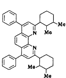
Compound No. 22
