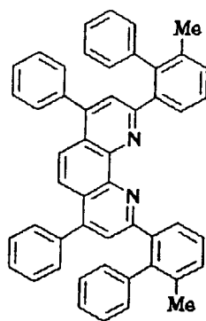
Compound No. 98
