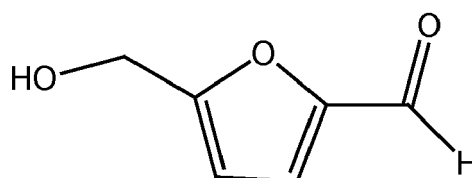
30 Hydroxymethylfurfural
