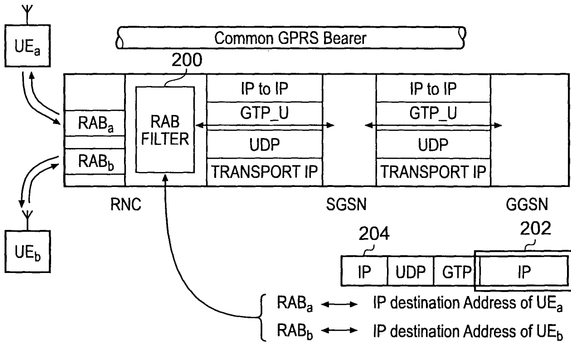
Fig. 15: Common PDP Context Shared GTP_U
