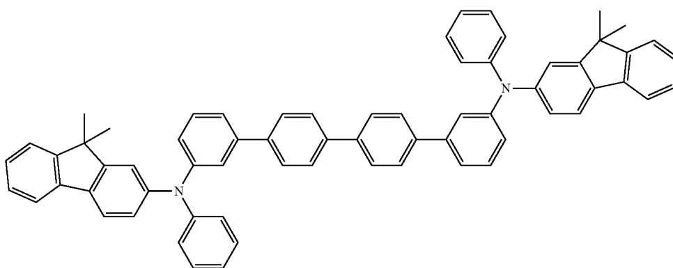
Compound 3
