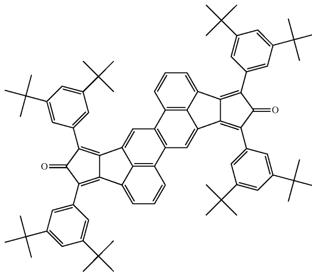
Compound 1-8
