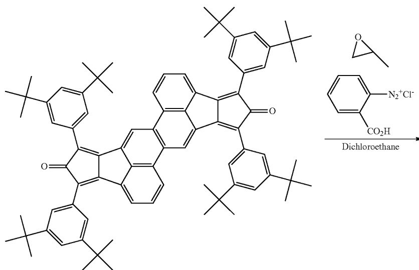
Compound 1-8
