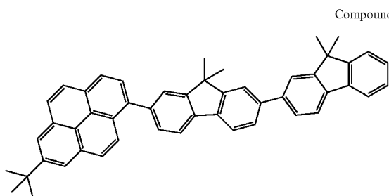
Compound 3
