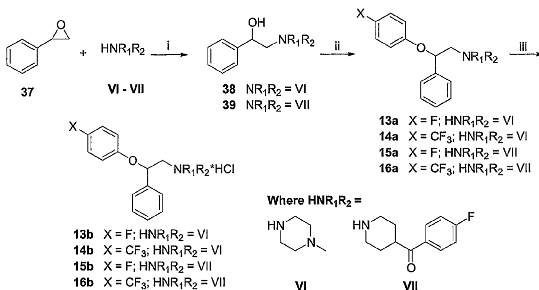
Scheme 4. Synthesis of Homologues Type I – Compounds 13 to 16.
