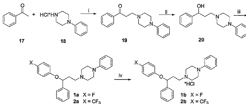
Scheme 1. Synthesis of Homologues Type II – Compounds 1 and 2.
