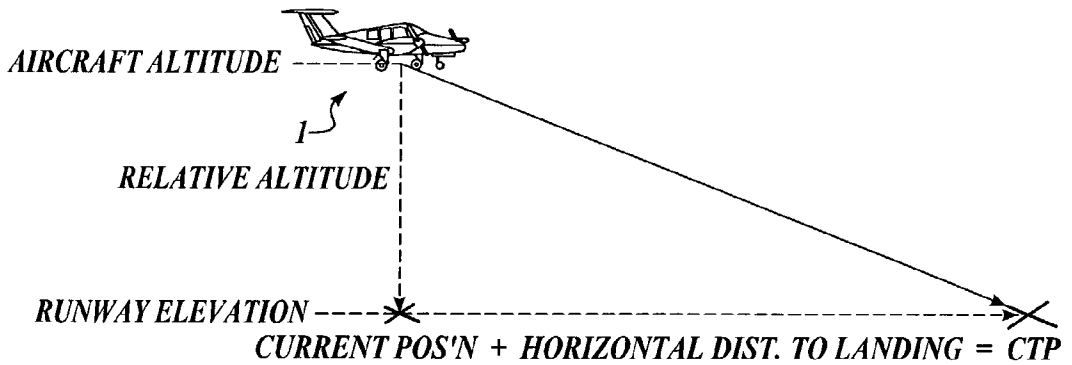
Fig. 10. (PRIOR ART)
