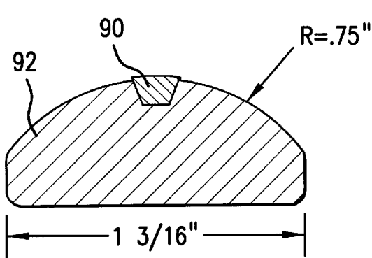
CATHODE FIG. 7C
