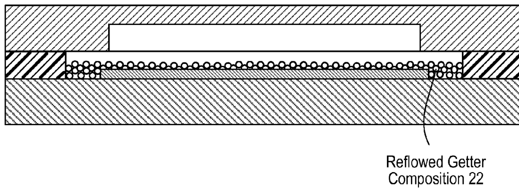
Encapsulated Device Before Reflow Of Getter 20
