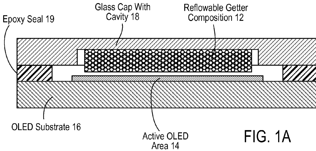
Encapsulated Device Before Reflow Of Getter 10
