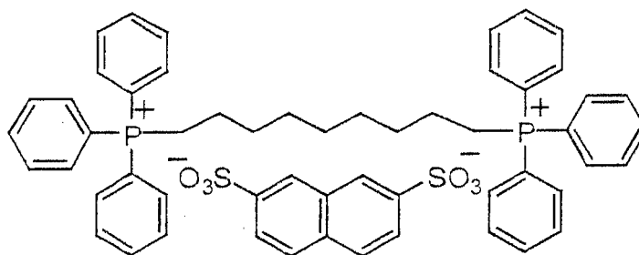
Phosphonium compound (1)
