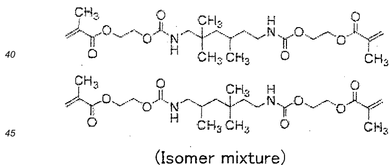
Polymerizable compound (1)
