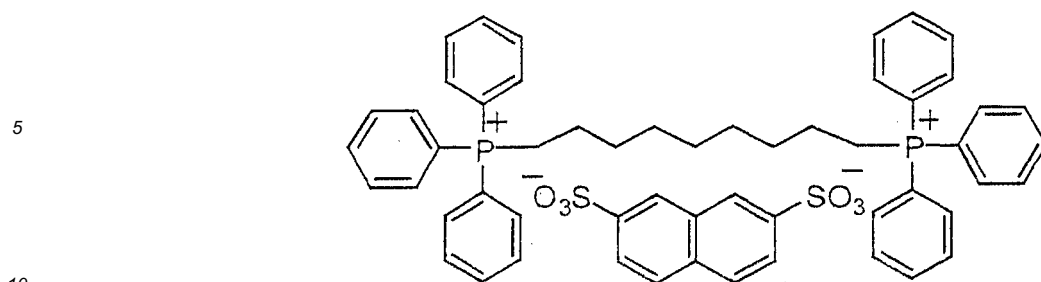
Phosphonium compound (1)
