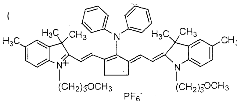
Infrared absorber (1)
