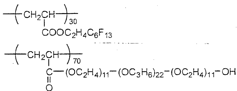
Fluorosurfactant (1)
