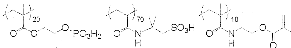
Undercoating compound (1)
