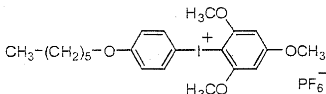
Polymerization initiator (1)
