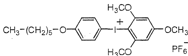
Polymerization initiator (1)
