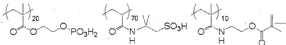
Undercoating compound (1)
