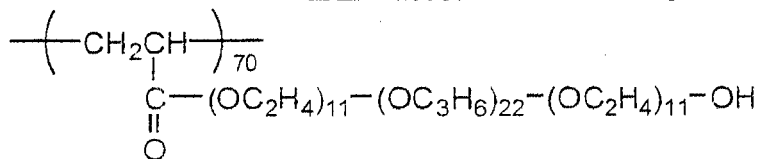
Fluorosurfactant (1)
