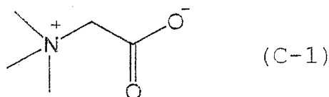
Low-molecular-weight hydrophilic compound (1)
