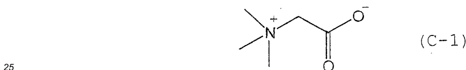
Low-molecular-weight hydrophilic compound (1)
