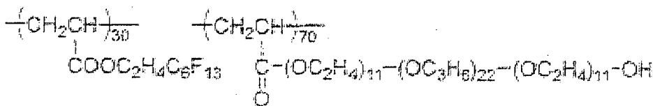
Fluorosurfactant (1)
