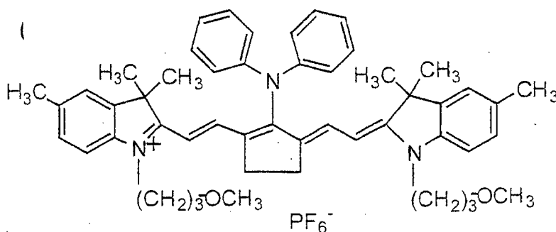
Infrared absorber (1)
