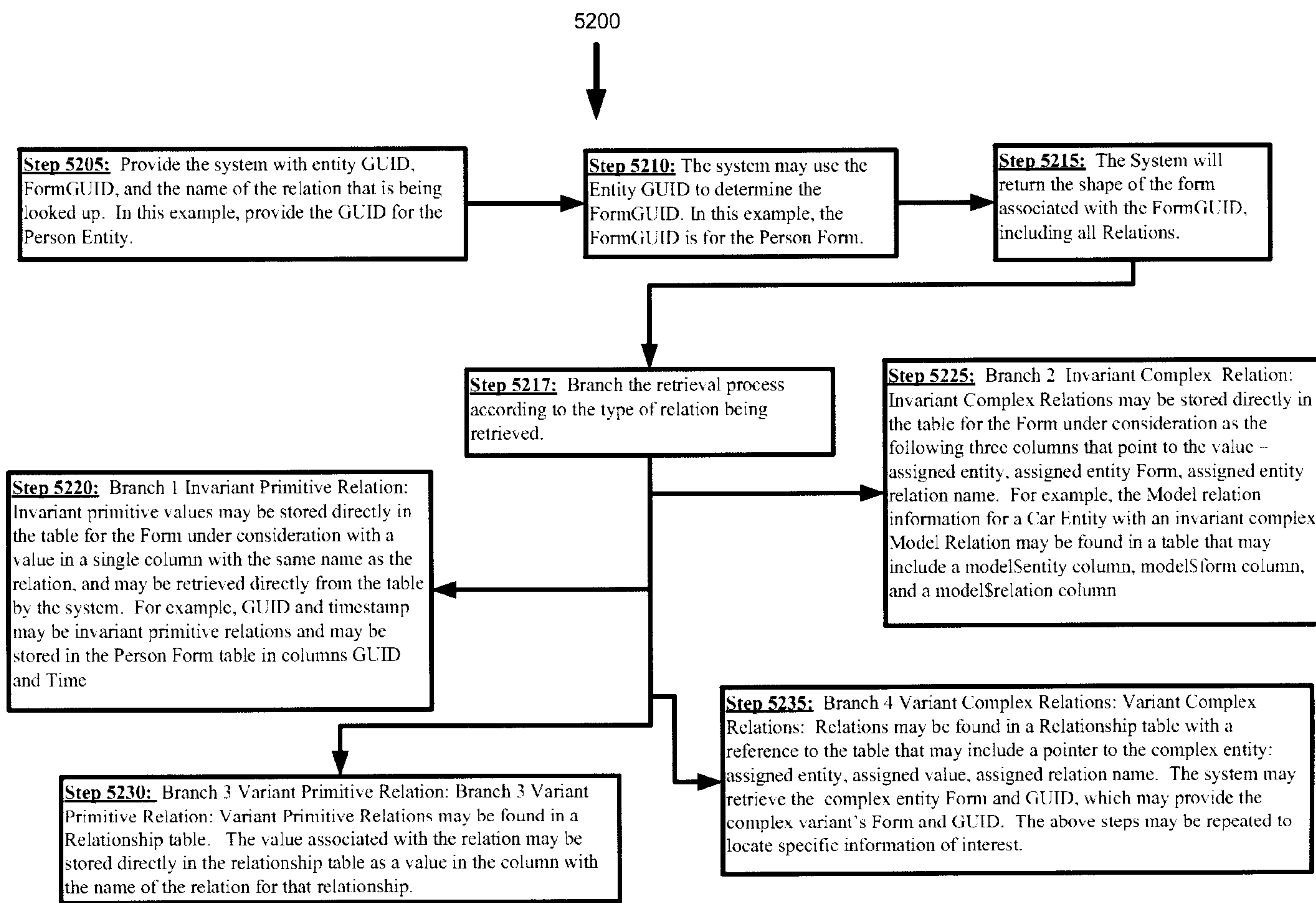
Figure 52. Example Process Flow for Retrieving Entity State
