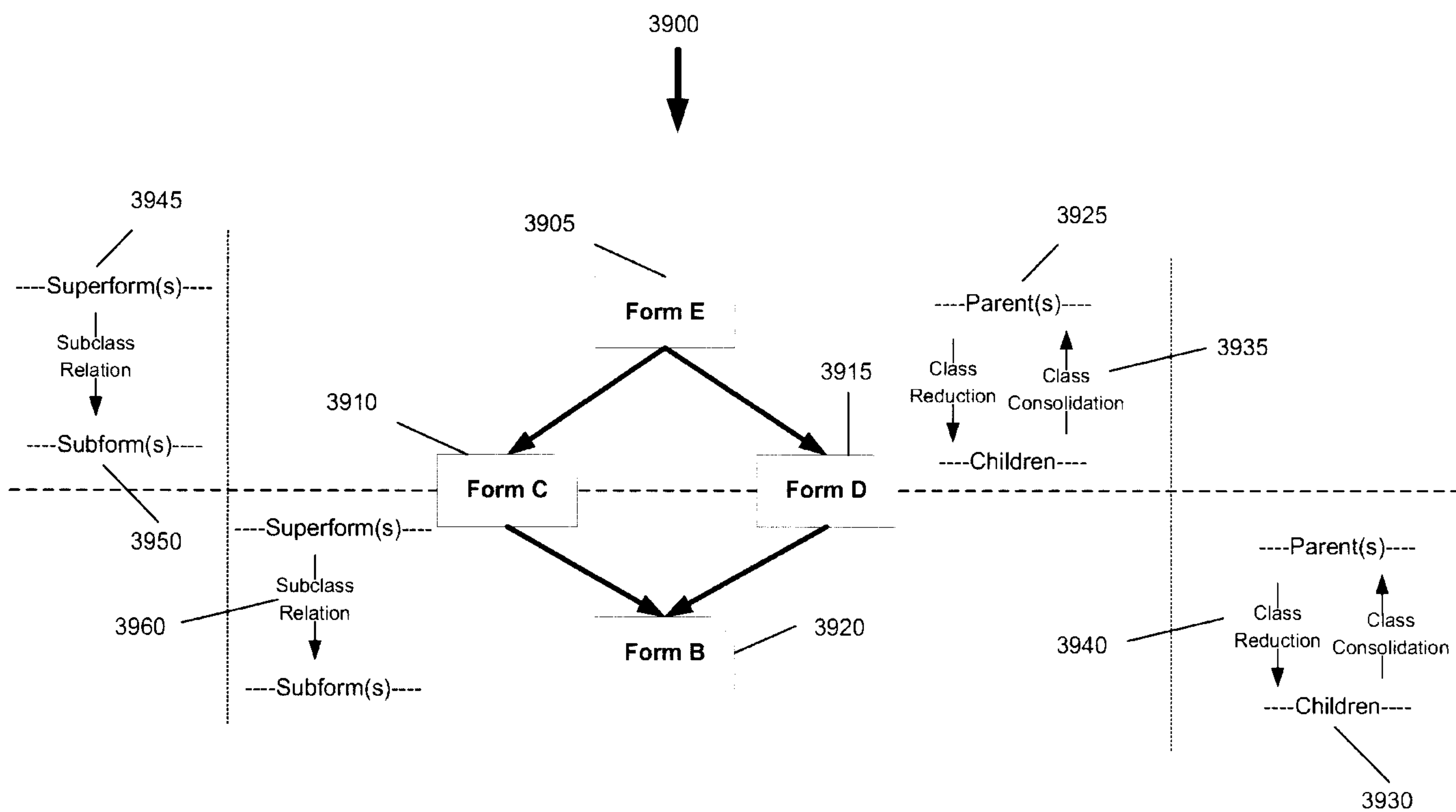
Figure 39. Subclassing Forms and Relations
