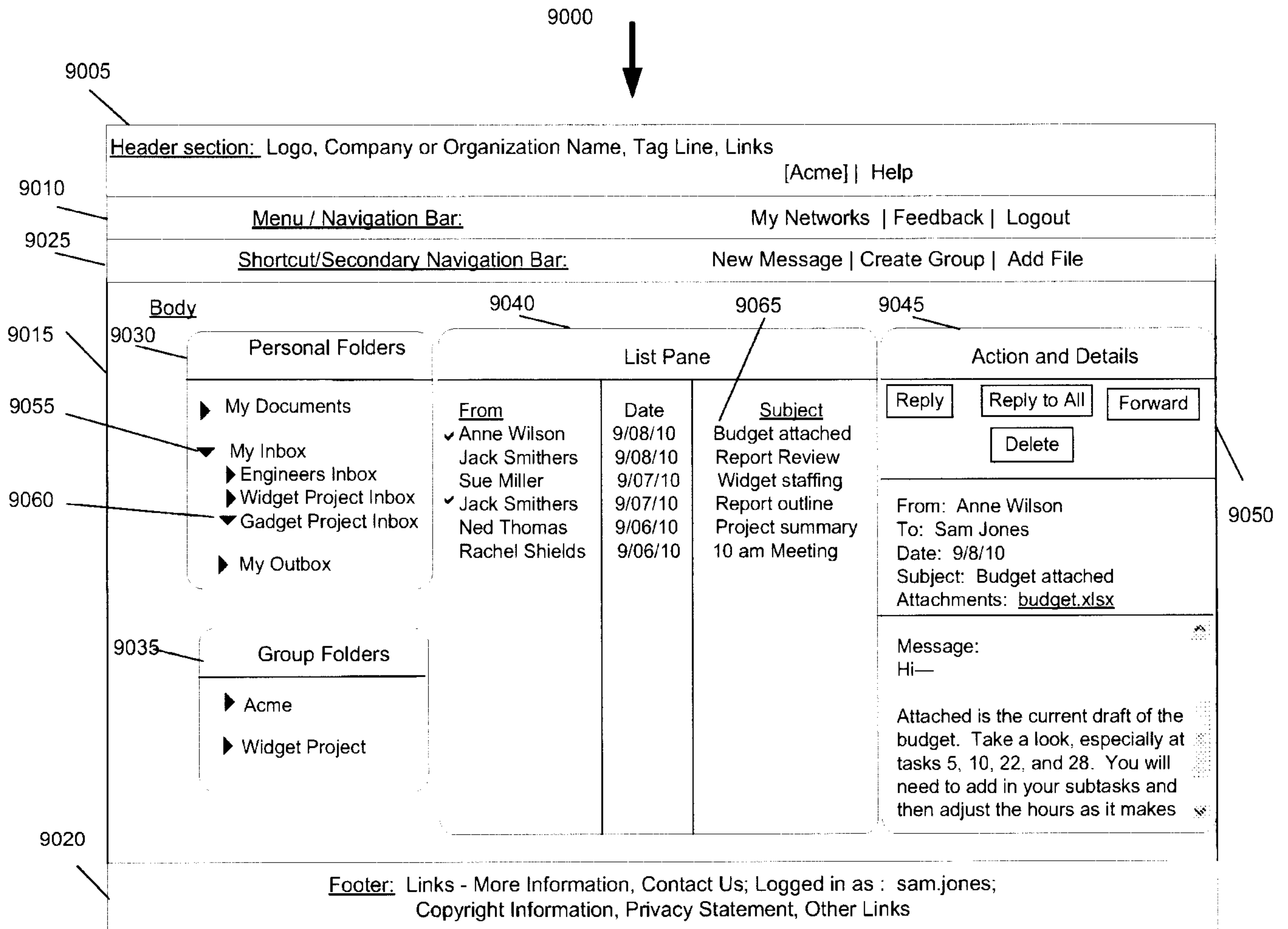
Figure 90. View Messages and Details
