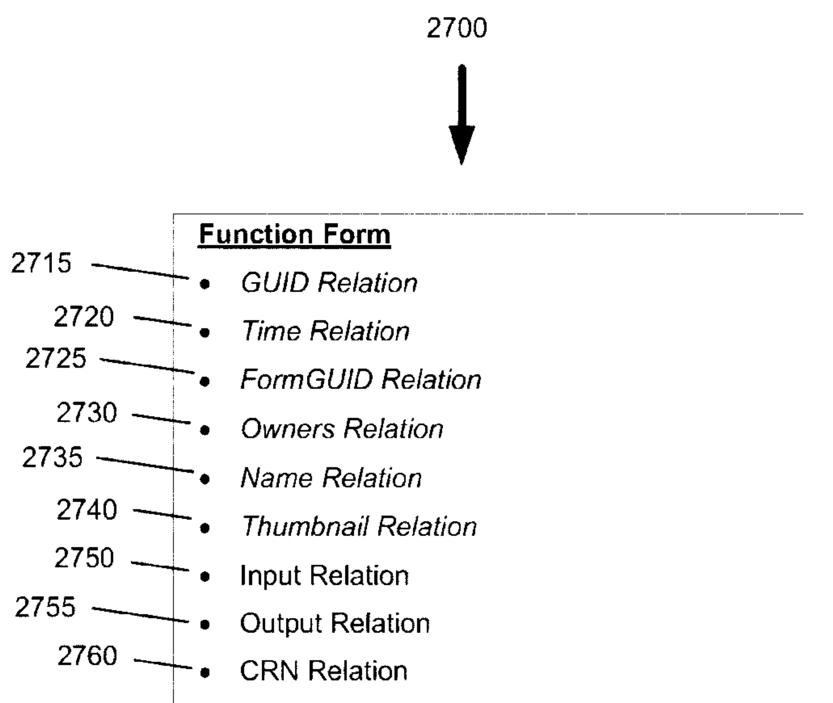
Figure 27. Example Function Form
