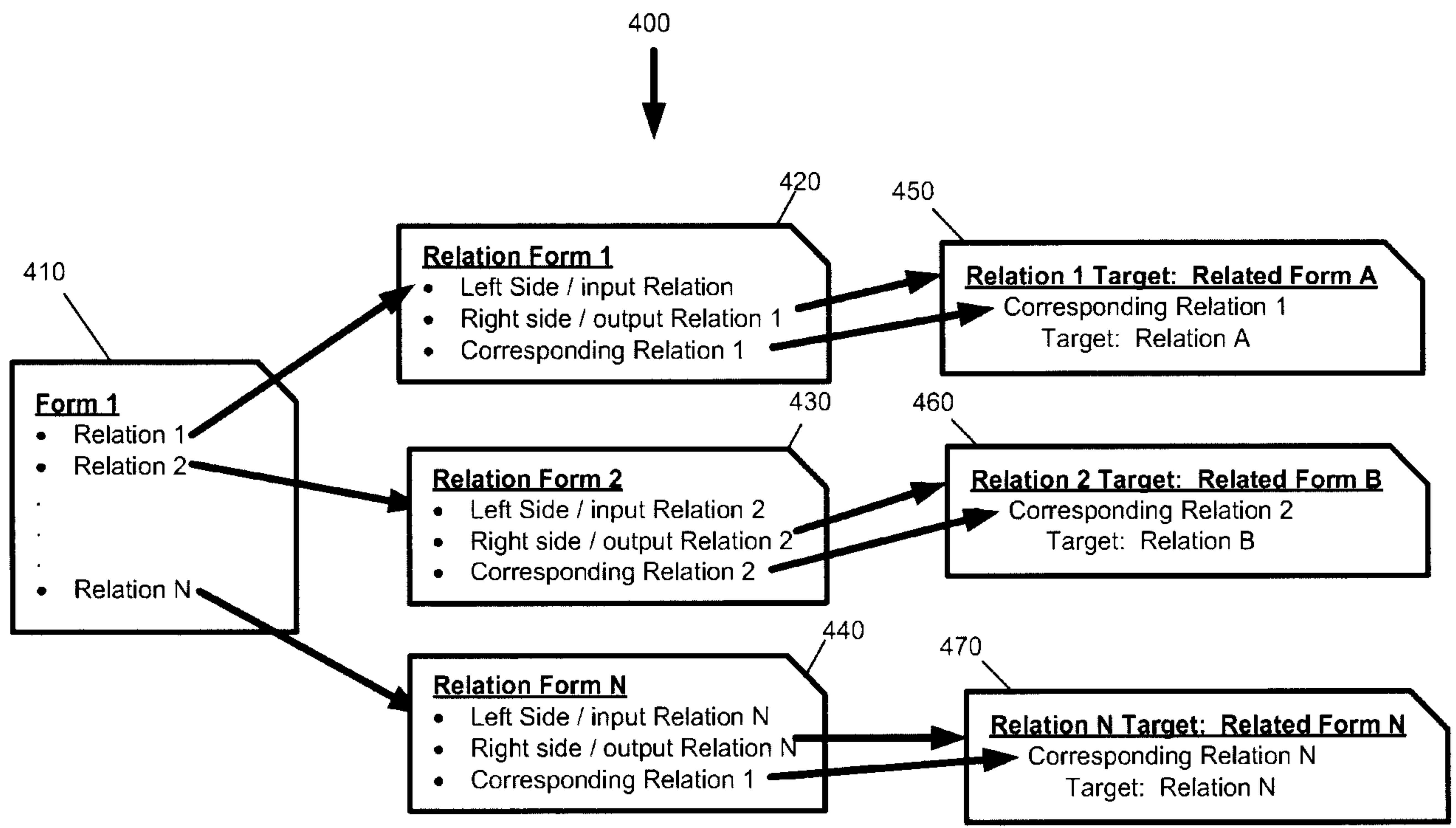
Figure 4. Forms, Relations, and Corresponding Relations
