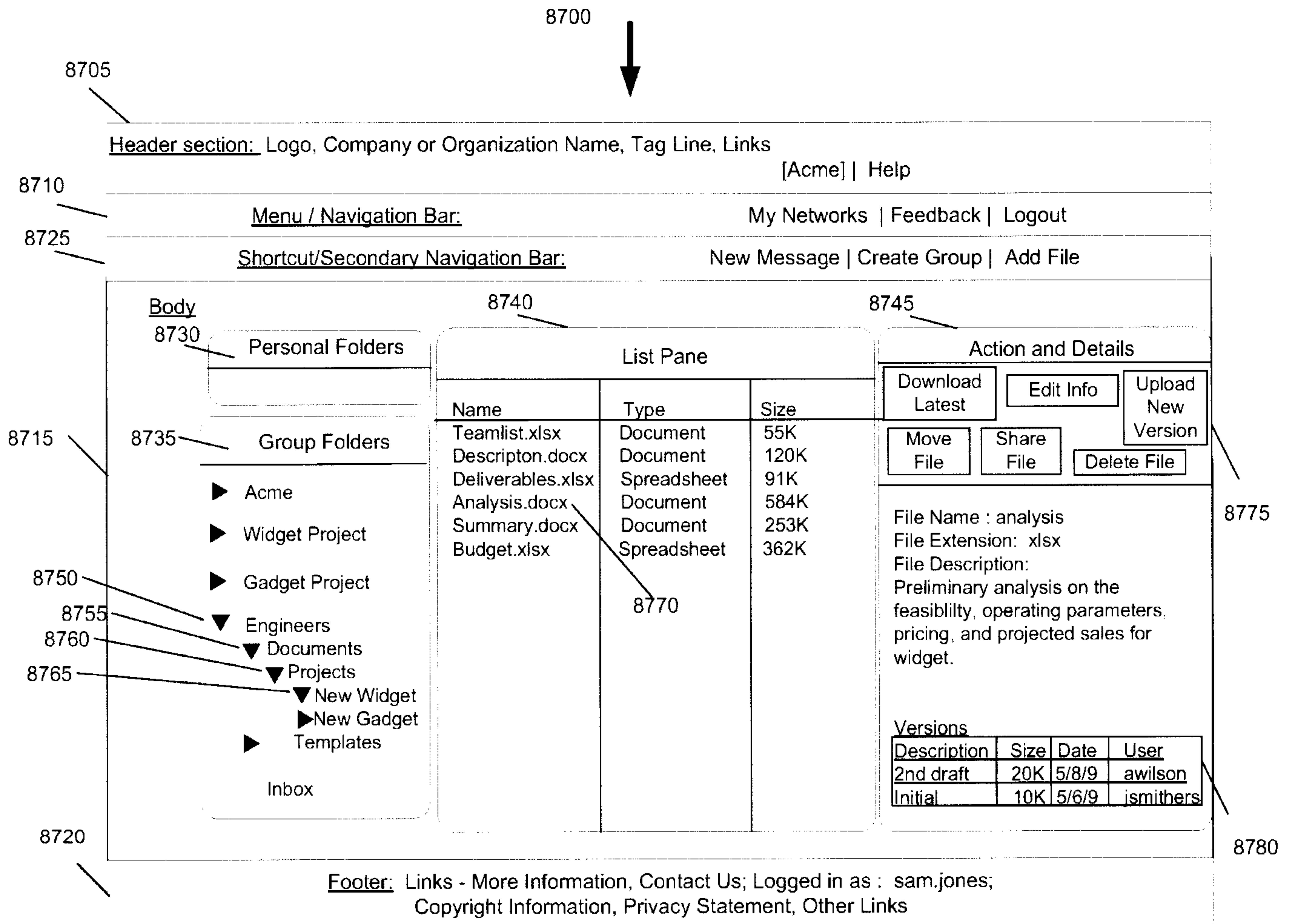
Figure 87. File Detail View
