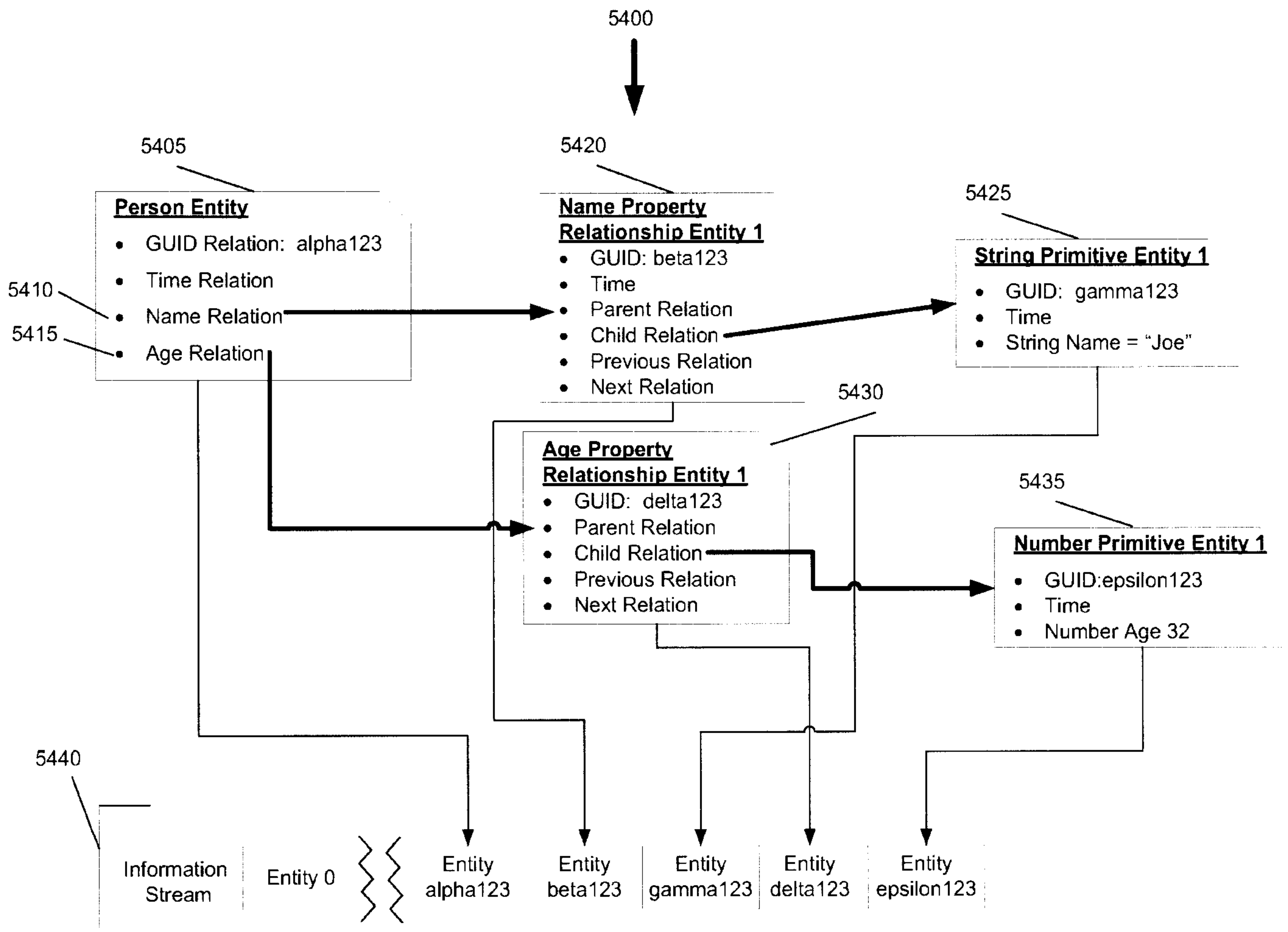
Figure 54. Simplified Conceptual View of Writing Person Entity and Related Entities to an Information Stream
