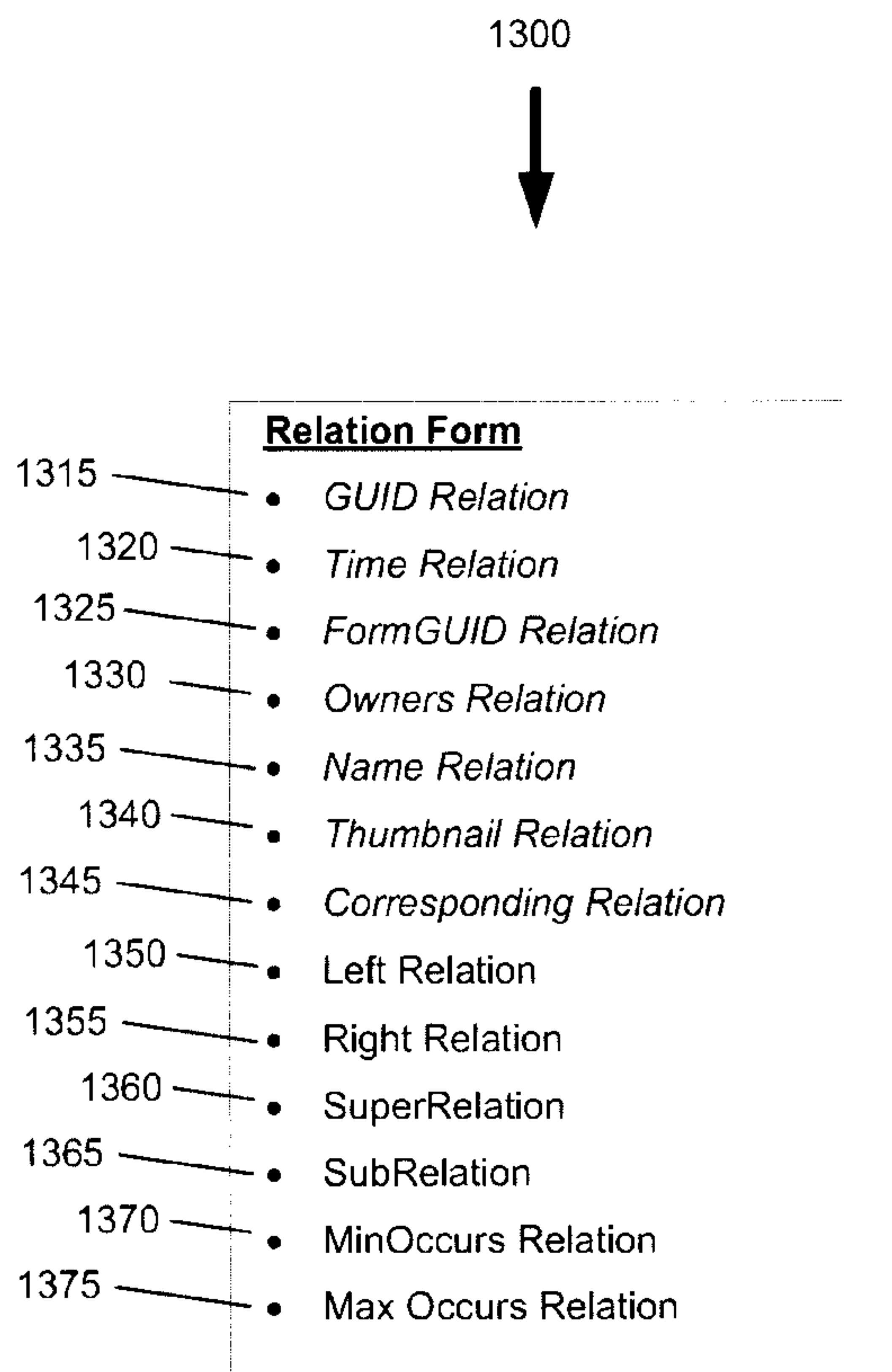
Figure 13. Example Relation Form
