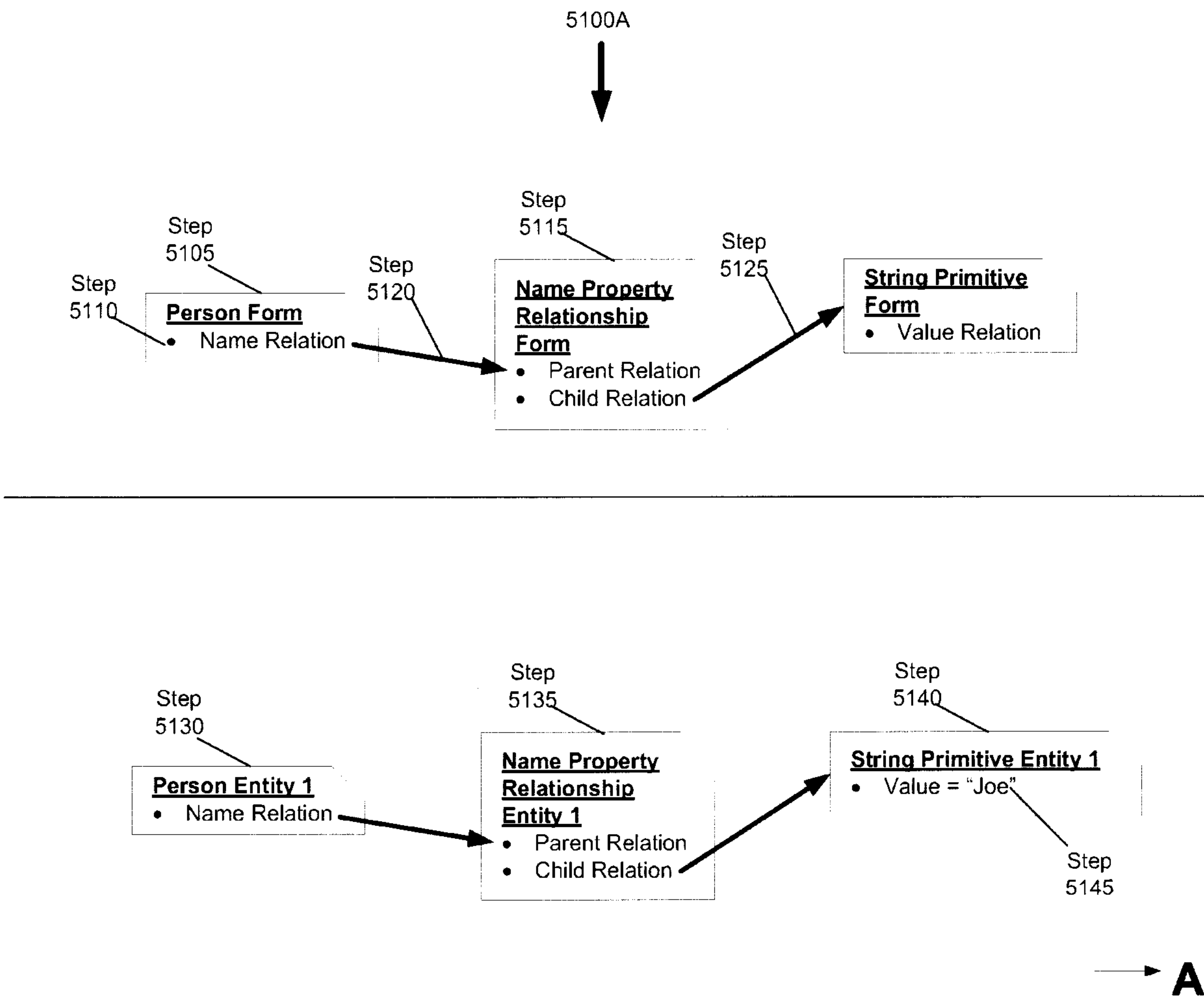
Figure 51A. Substitution Process Flow Example: Step 5105 through – Step 5145
