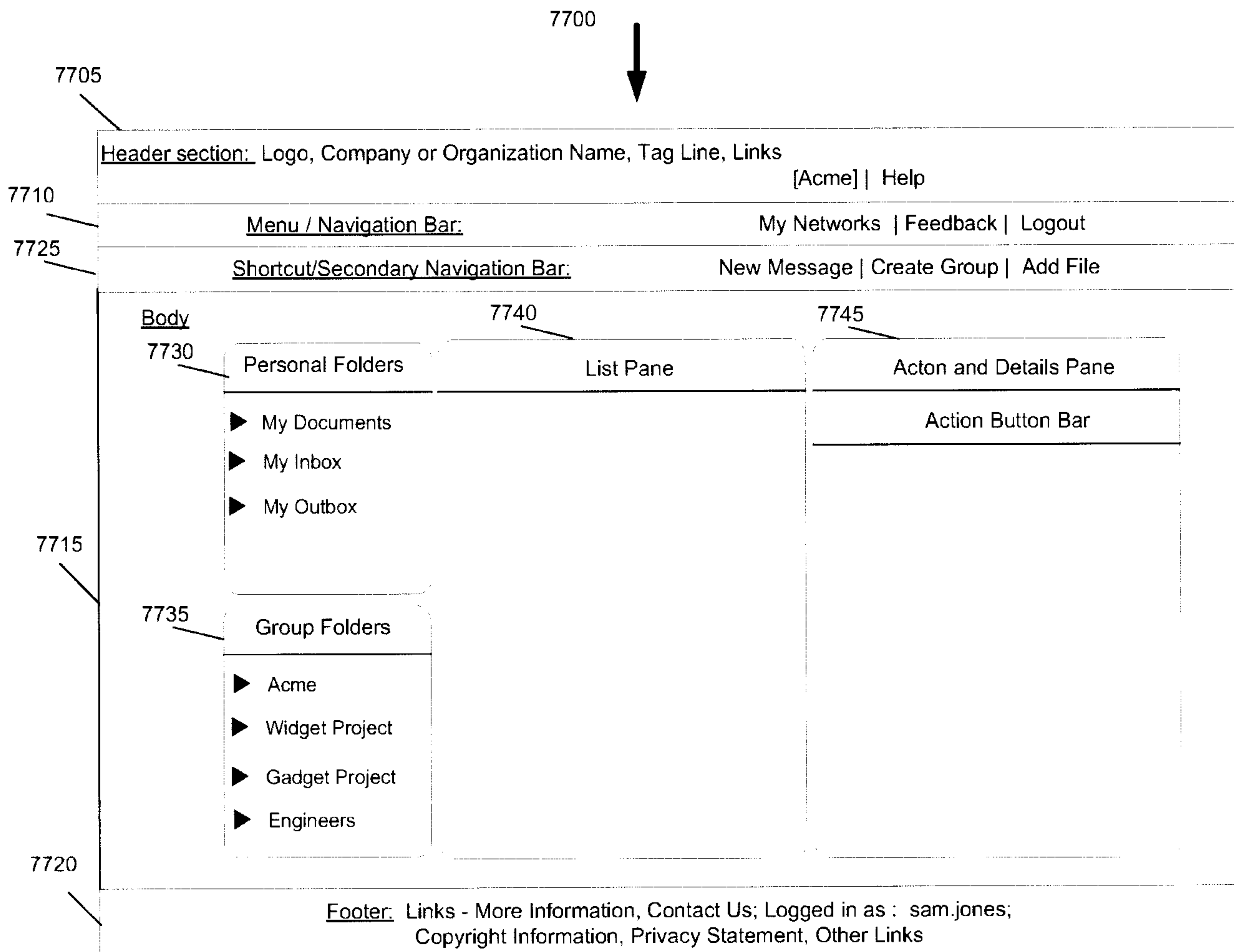
Figure 77. Network Home Page
