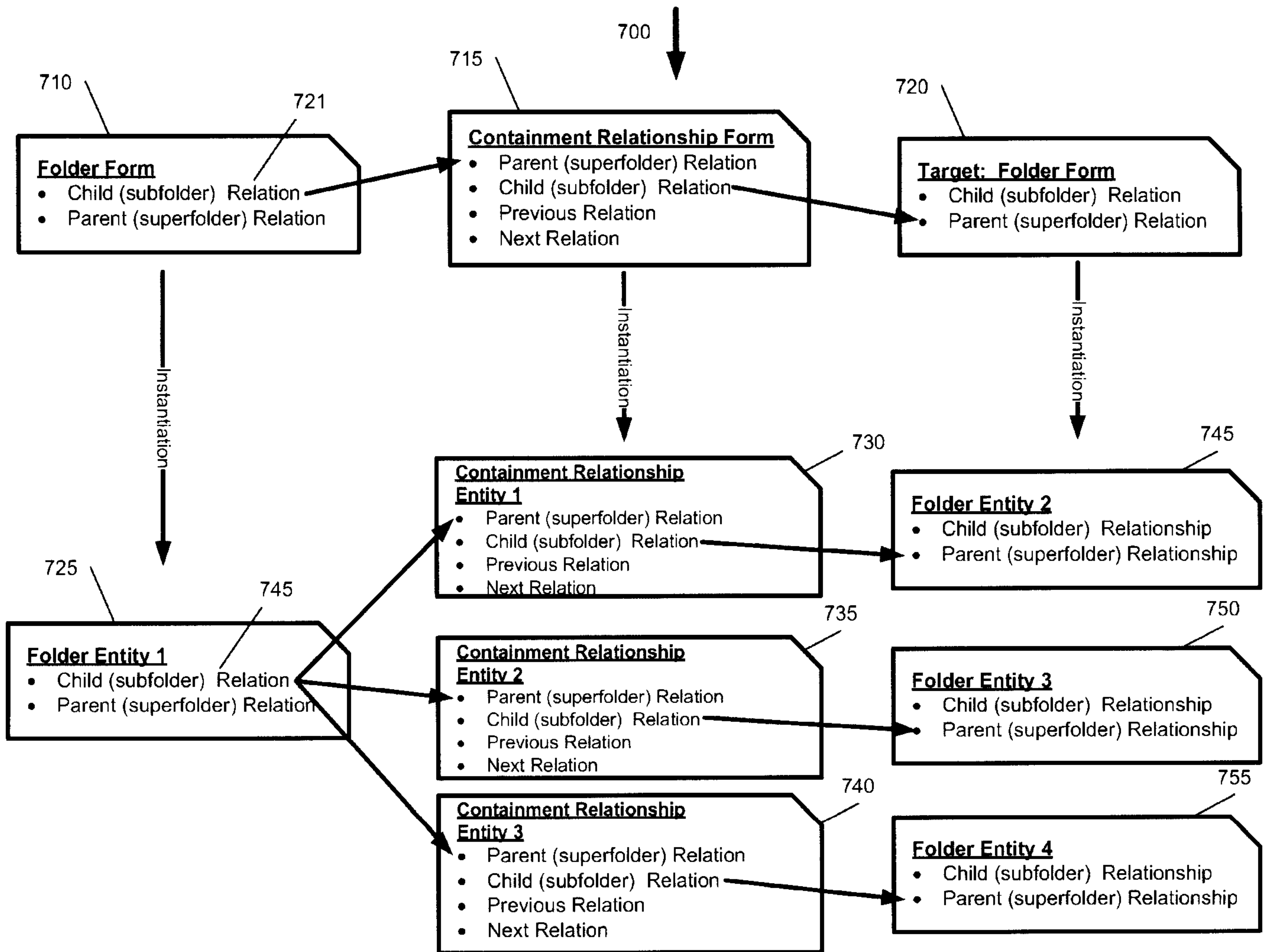
Figure 7. Example Variant Child (Subfolder) Relation
