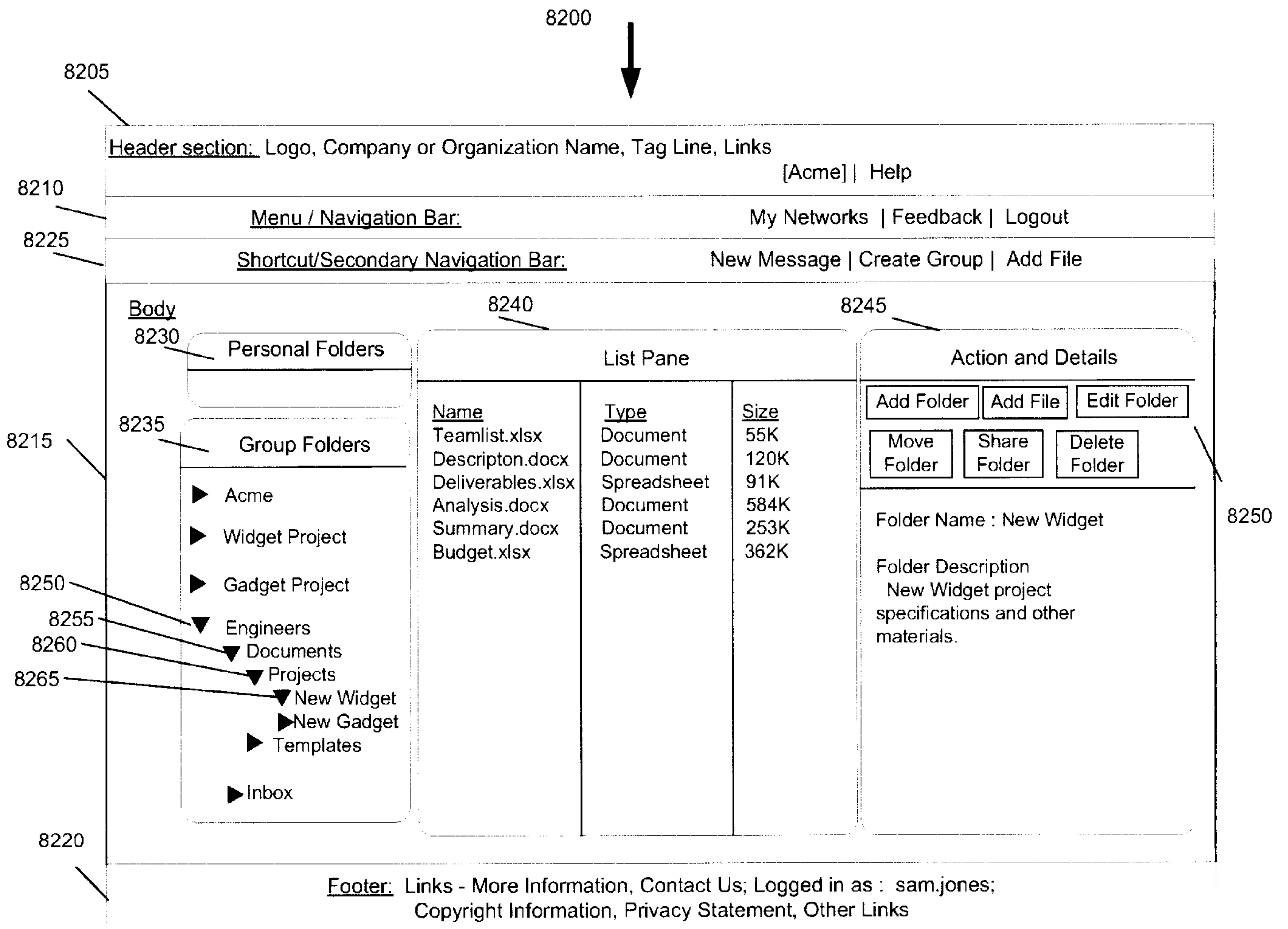
Figure 82. Group Folders Expanded View
