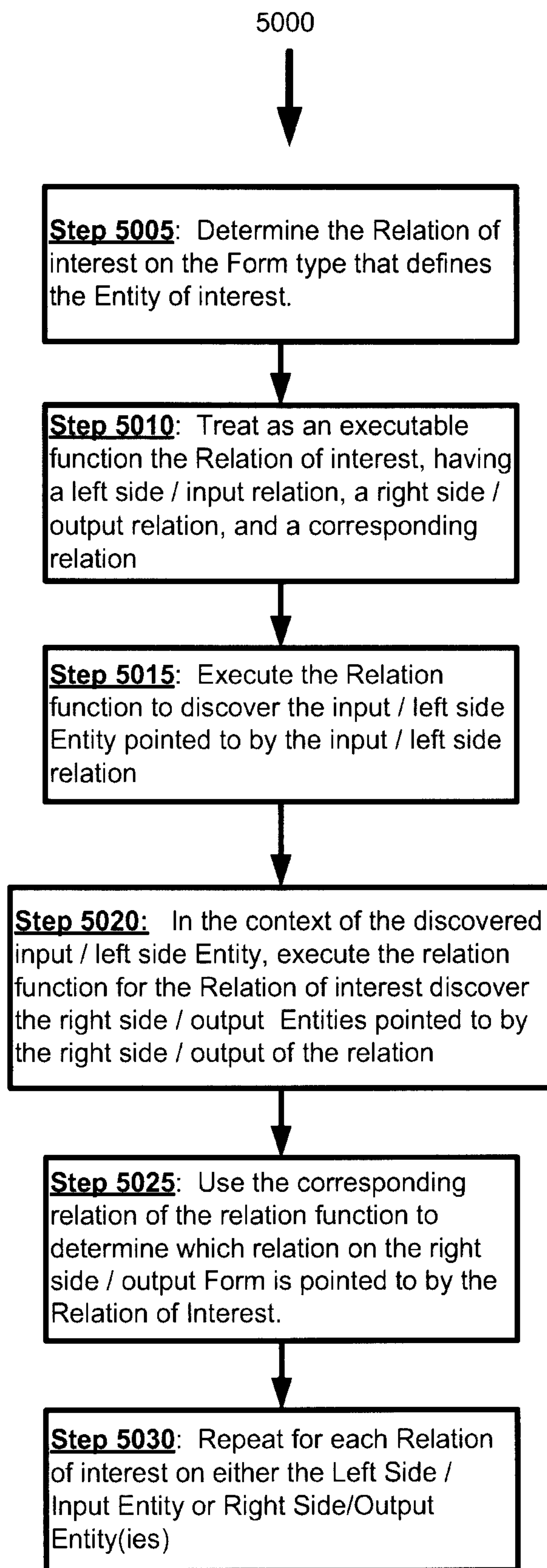
Figure 50. Conceptual Overview of the Process Flow For Traversing Relations
