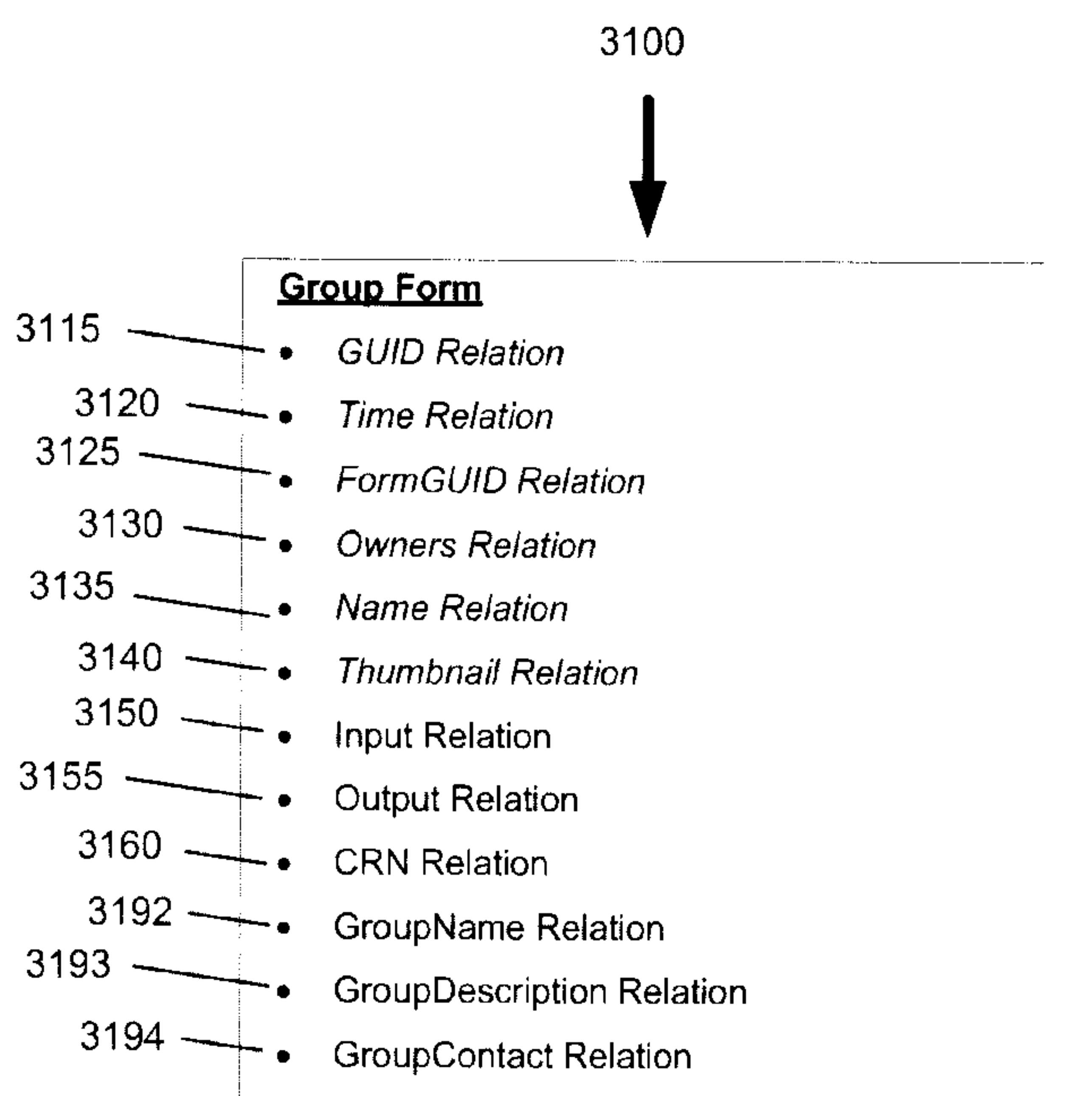
Figure 31. Example Group Form
