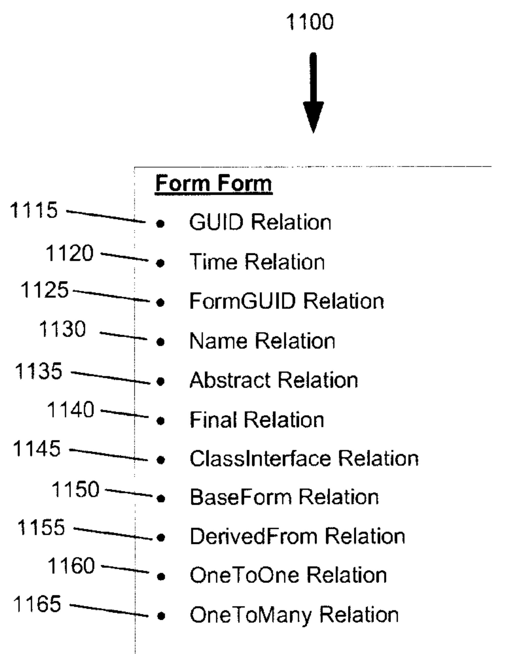
Figure 11. Example Form Form
