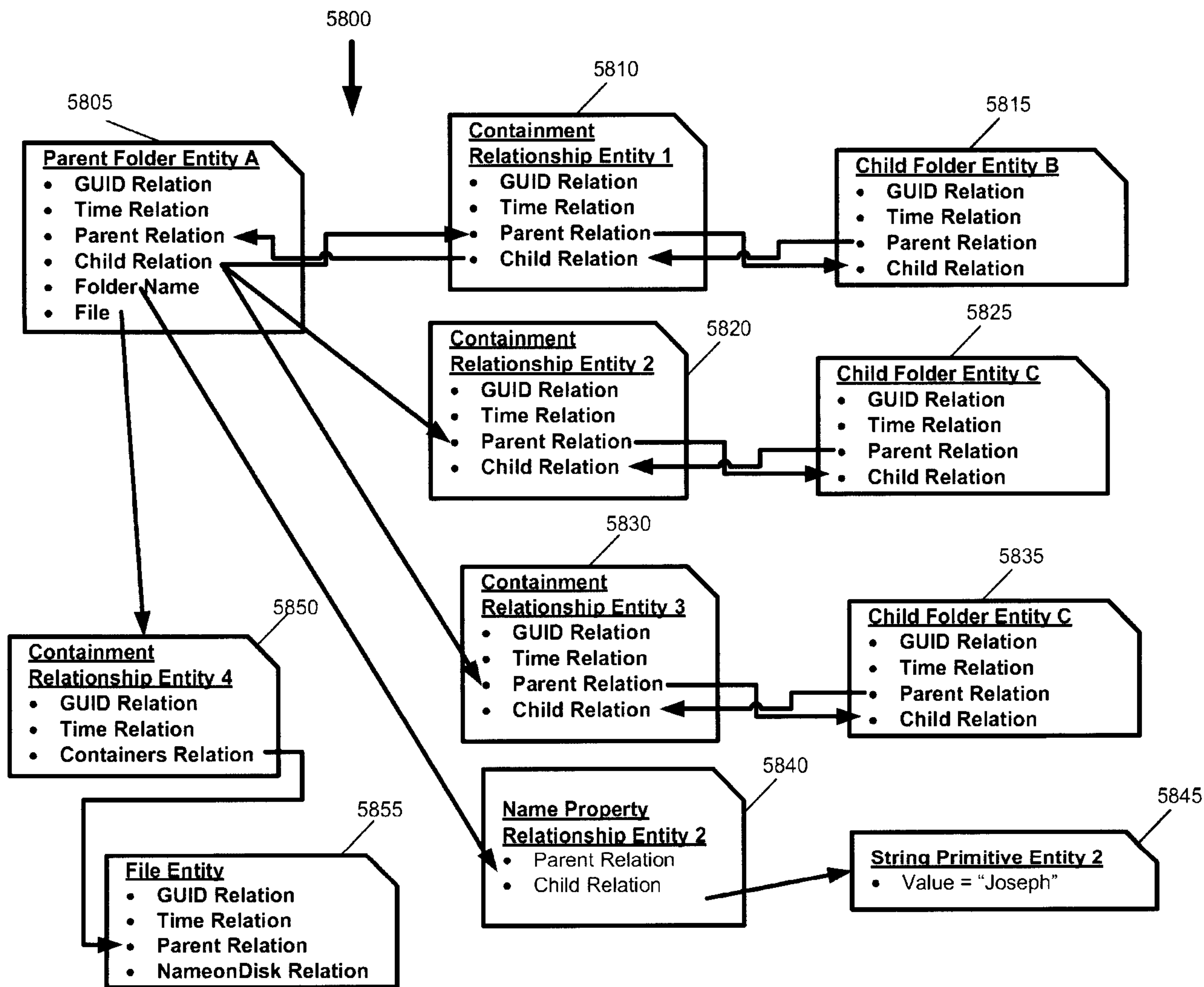
Figure 58. Example of Writing Streams for Multiple Containment and Other Relationships
