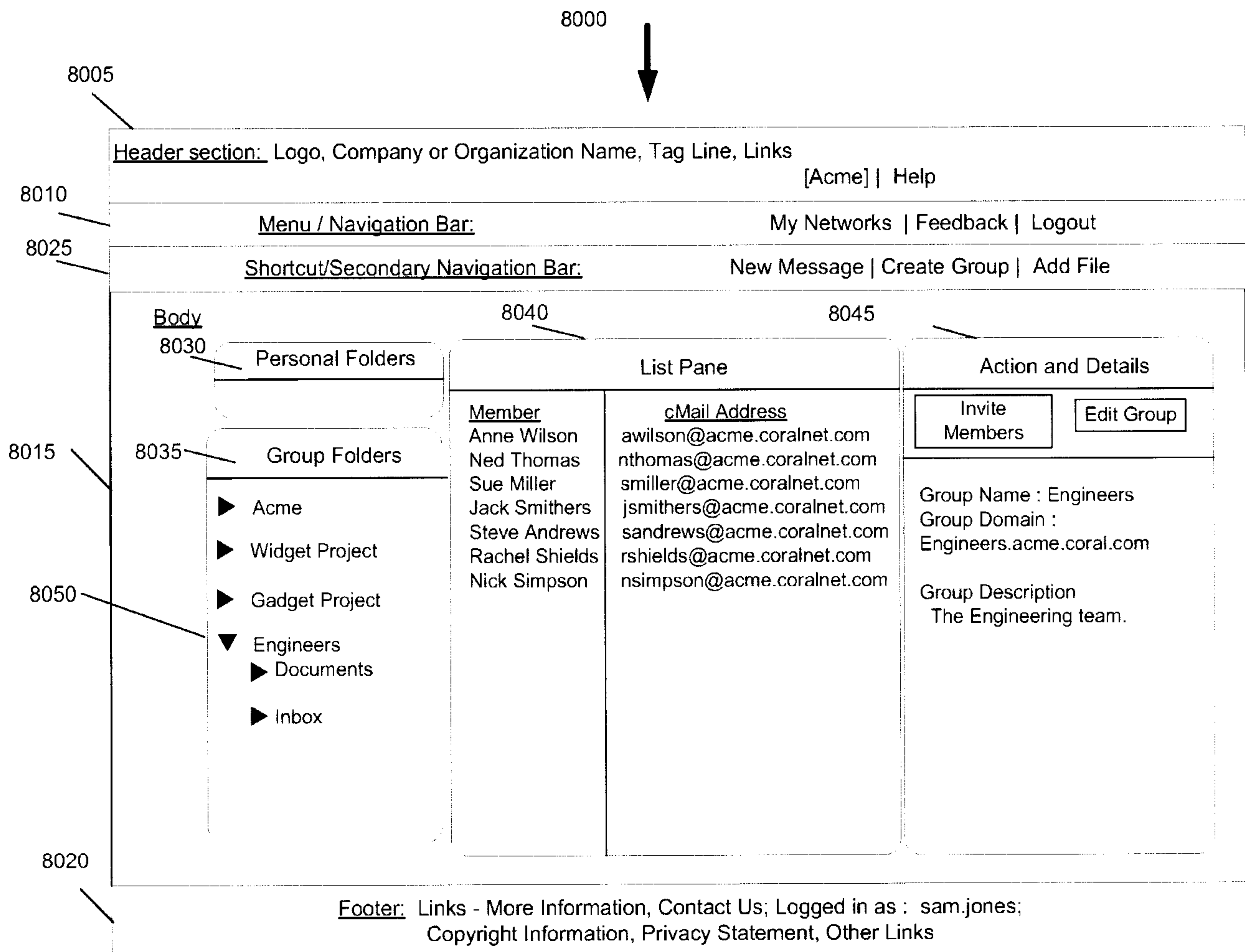
Figure 80. Group and Group Members View
