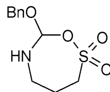
Compound D4
