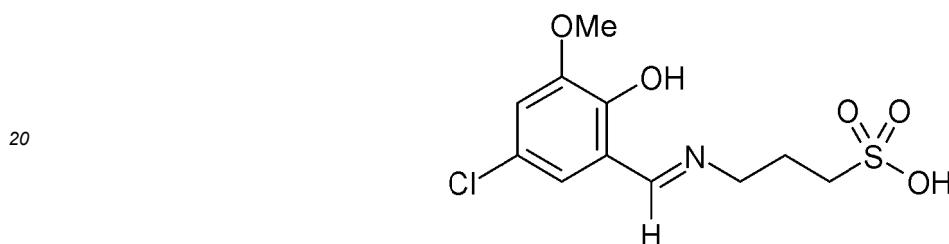
Compound M9
