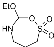
Compound D3
