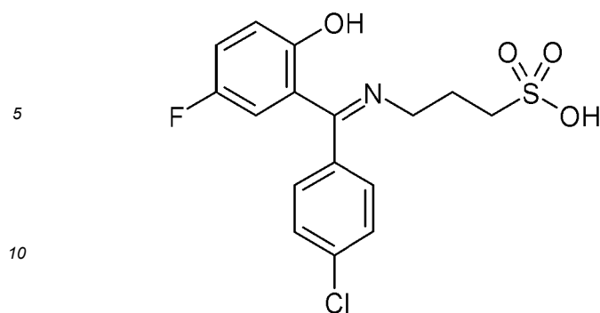
Compound M7
