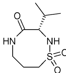
Compound D8*
