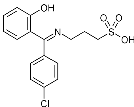
Compound M8
