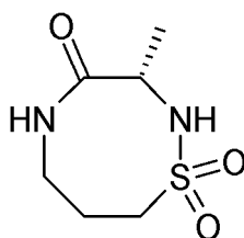
Compound D7*
