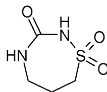
Compound D5*
