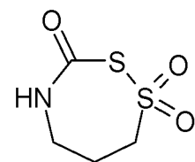
Compound D6*
