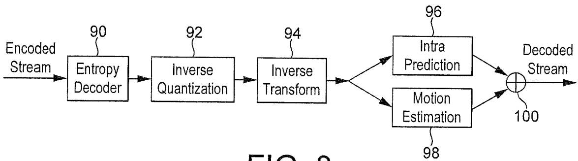
FIG. 8 (Prior Art)
