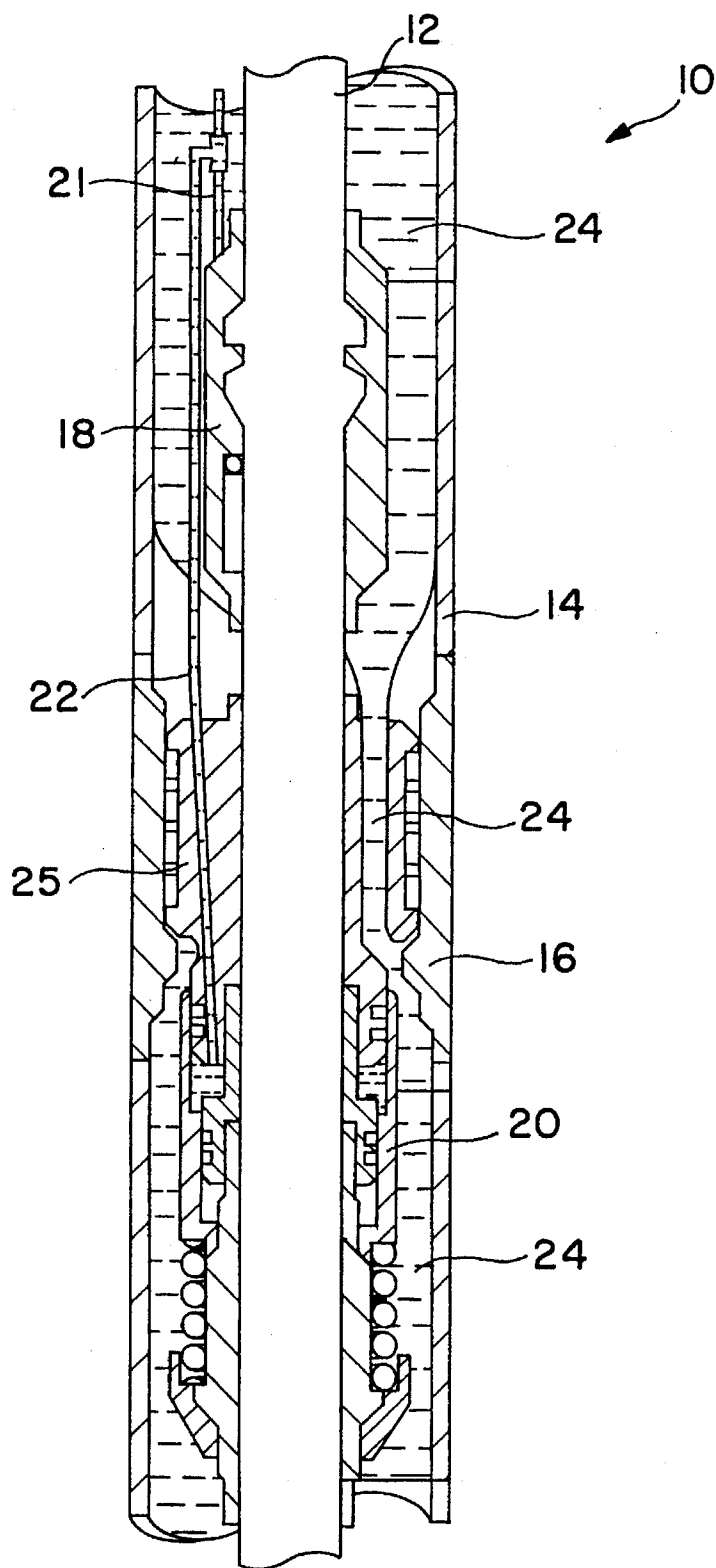
FIG. 1 PRIOR ART
