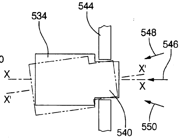
PRIOR ART FIG. 45
