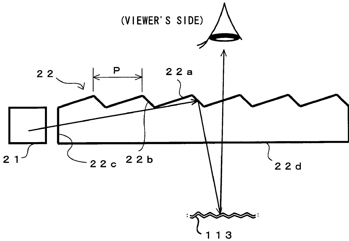
FIG. 3 PRIOR ART
