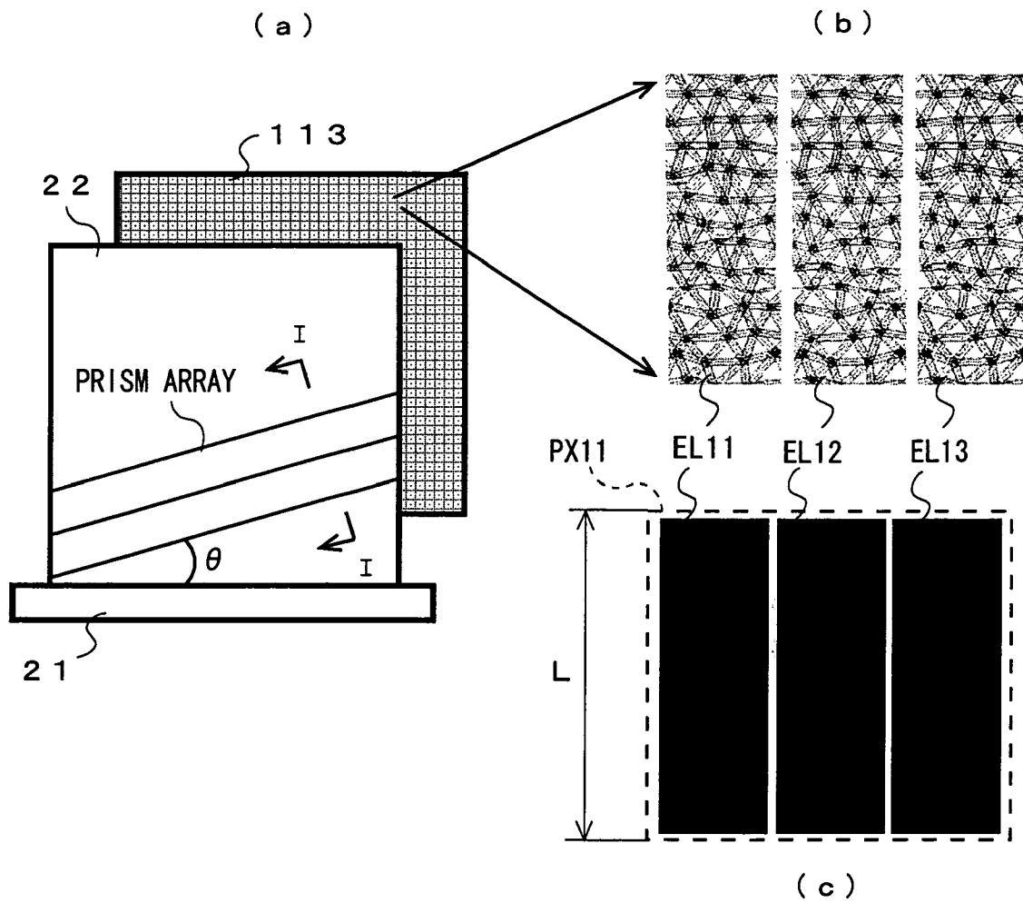
FIG. 2 PRIOR ART
