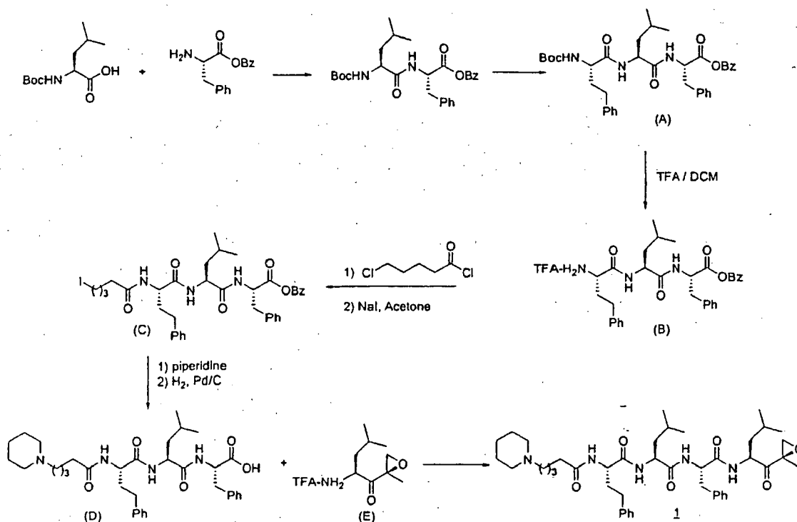
Scheme 1: Synthesis of Example 1
