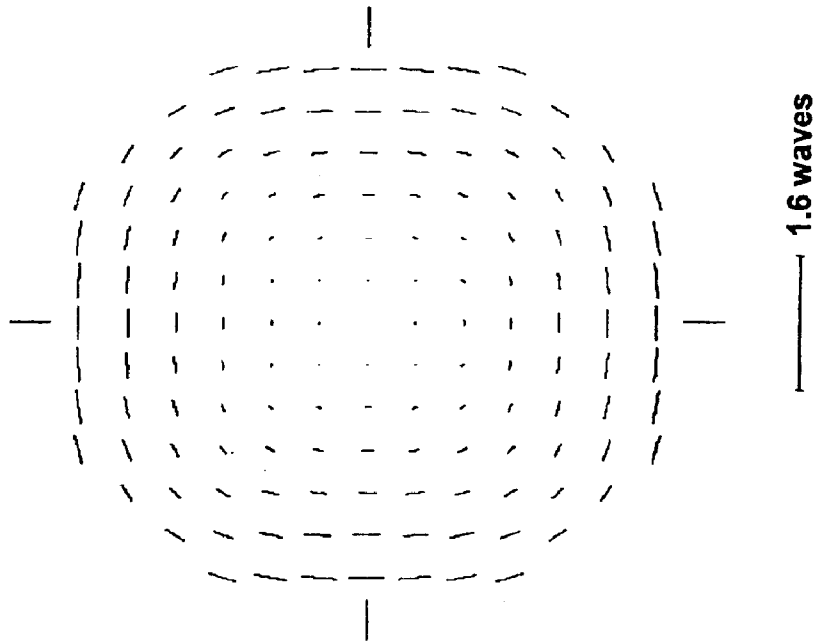
Net Retardance of Elements Between Rotators, On-Axis Field
