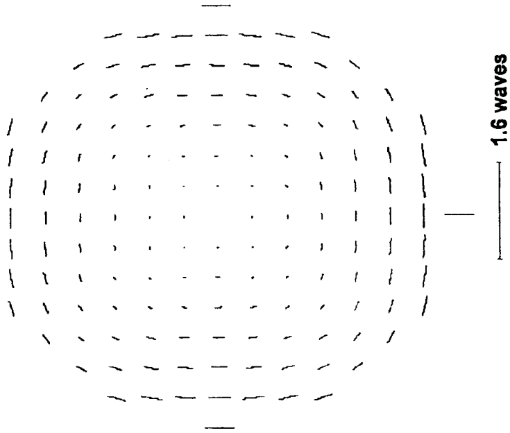
Net Retardance of Elements Following Rotators, Extreme Field
