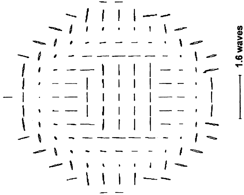
Retardance, Extreme Field
