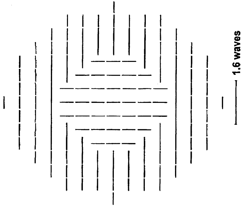
Net Retardance without Rotator, On-Axis Field
