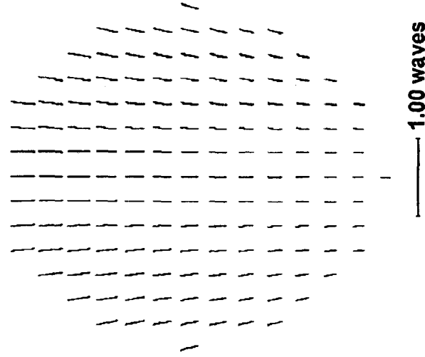
Retardance from Stress Induced Birefringence, Extreme Field
