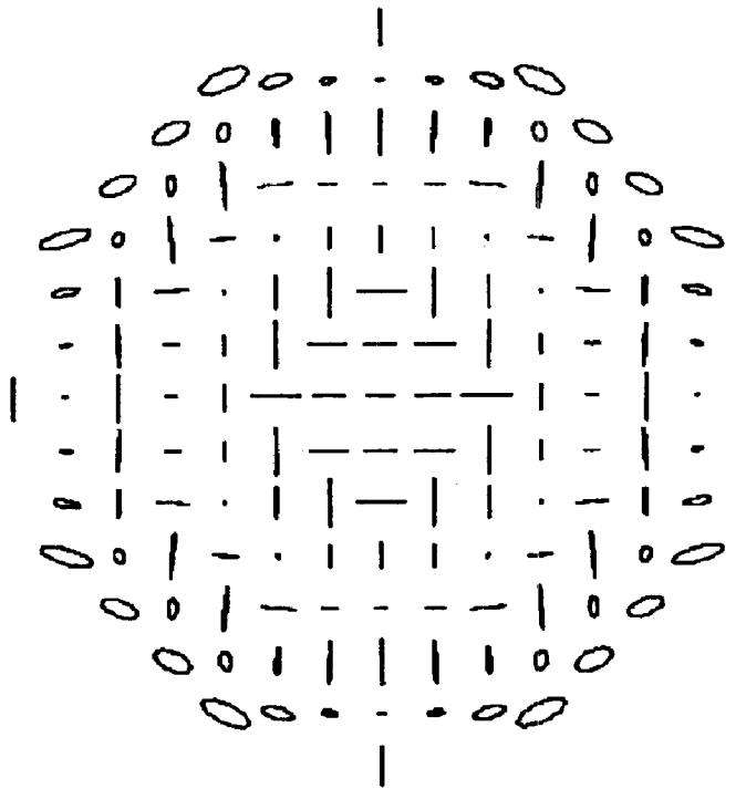
Retardance, On-Axis Field
