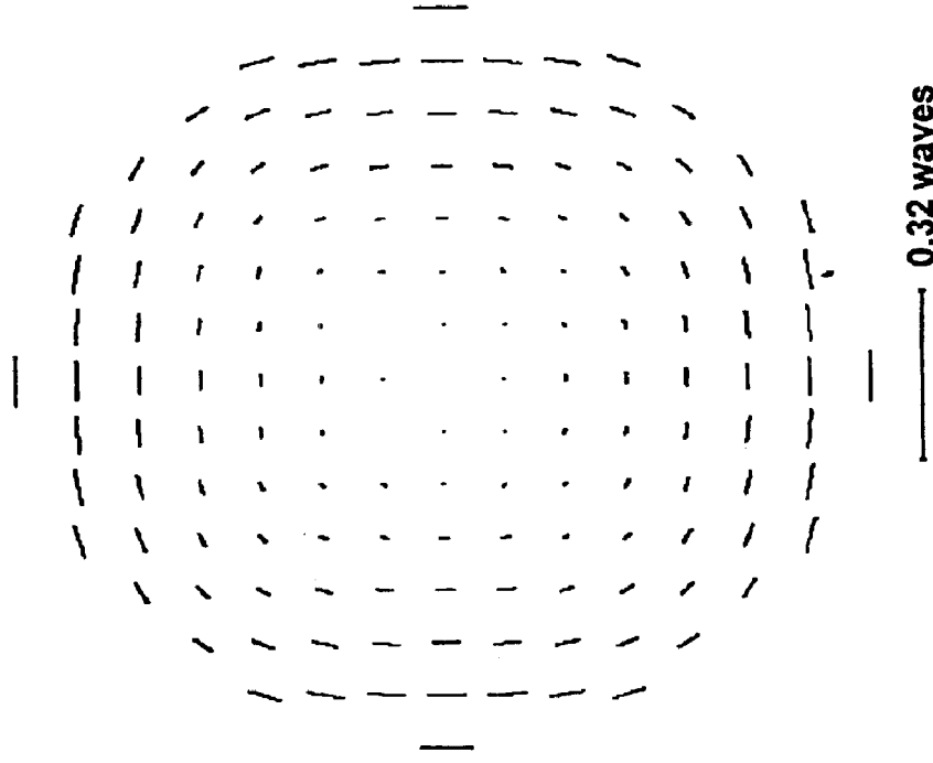
Net Retardance without Rotator, Extreme Field
