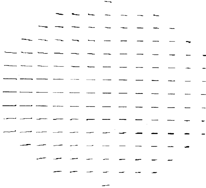
Net Retardance All Elements Plus Rotators 1 and 2, Extreme Field
