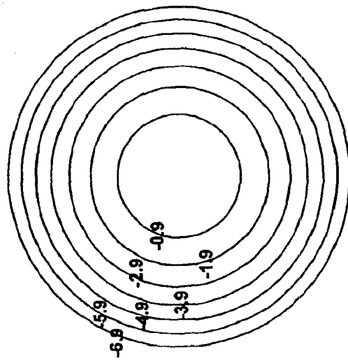
Stress Induced Birefringence Magnitude (nm/cm)
