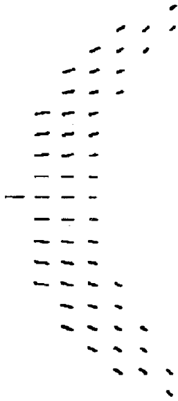
Net Retardance with rotator and [111] Element, Extreme Field
