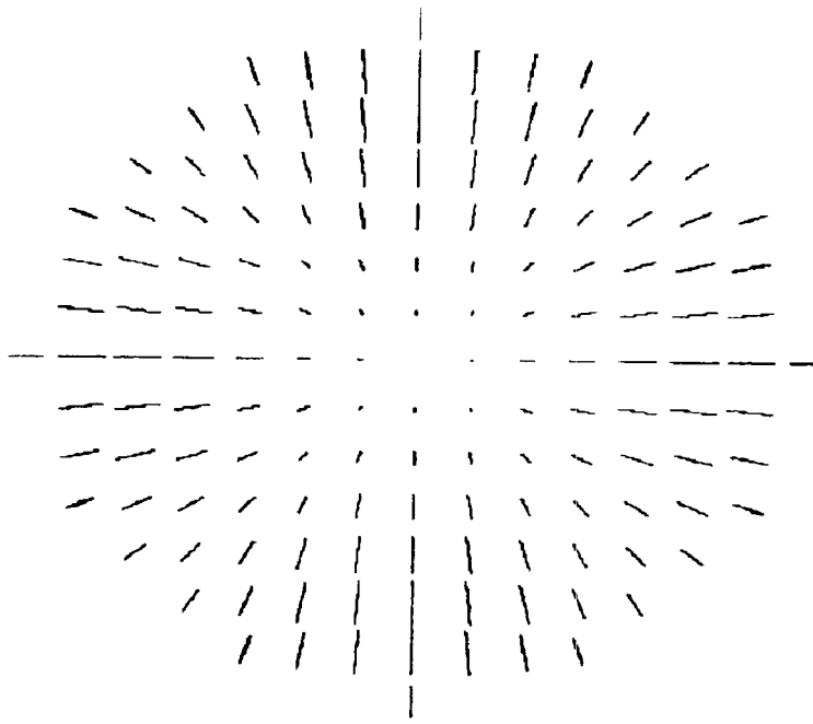
Net Refardance All Elements Plus Rotators 1 and 2, On-Axis
