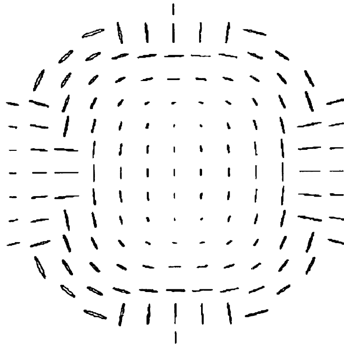
Retardance, On-Axis Field
