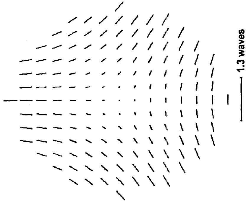
Net Retardance without Rotator, On-Axis Field
