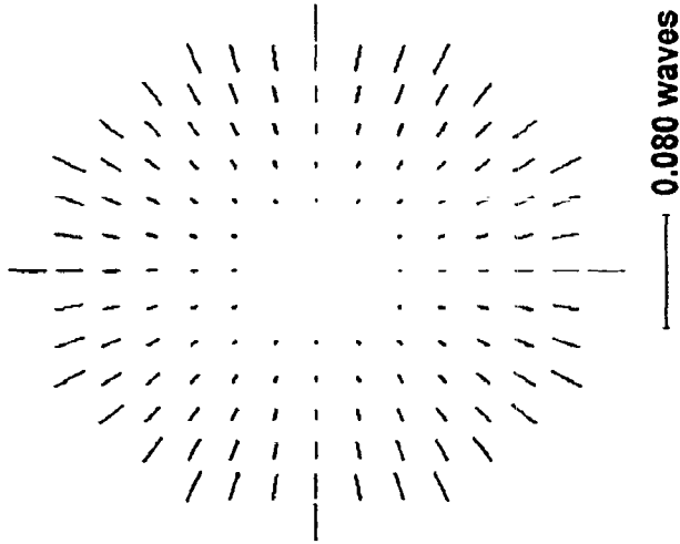
Retardance from Stress Induced Birefringence, On-Axis Field
