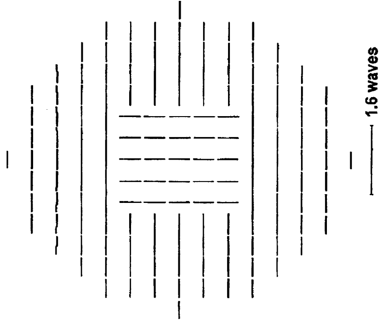
Net Retardance without Rotator, Extreme Field
