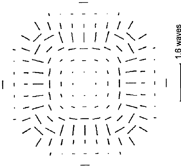
Retardance, On-Axis Field
