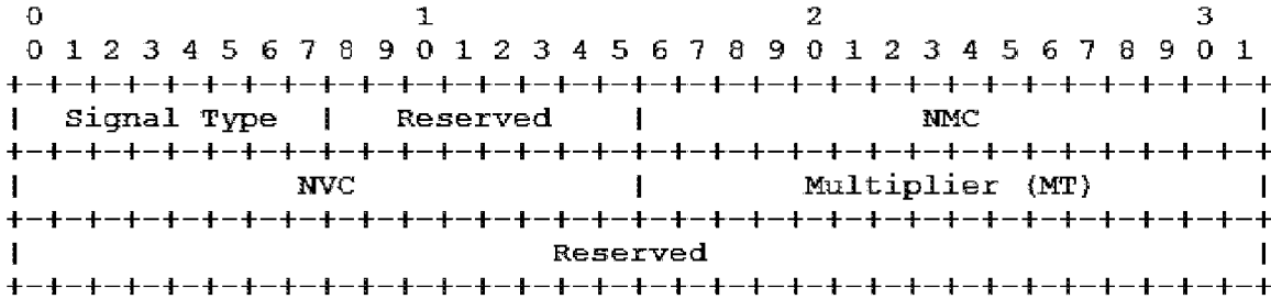
Generalized label request and traffic parameters
