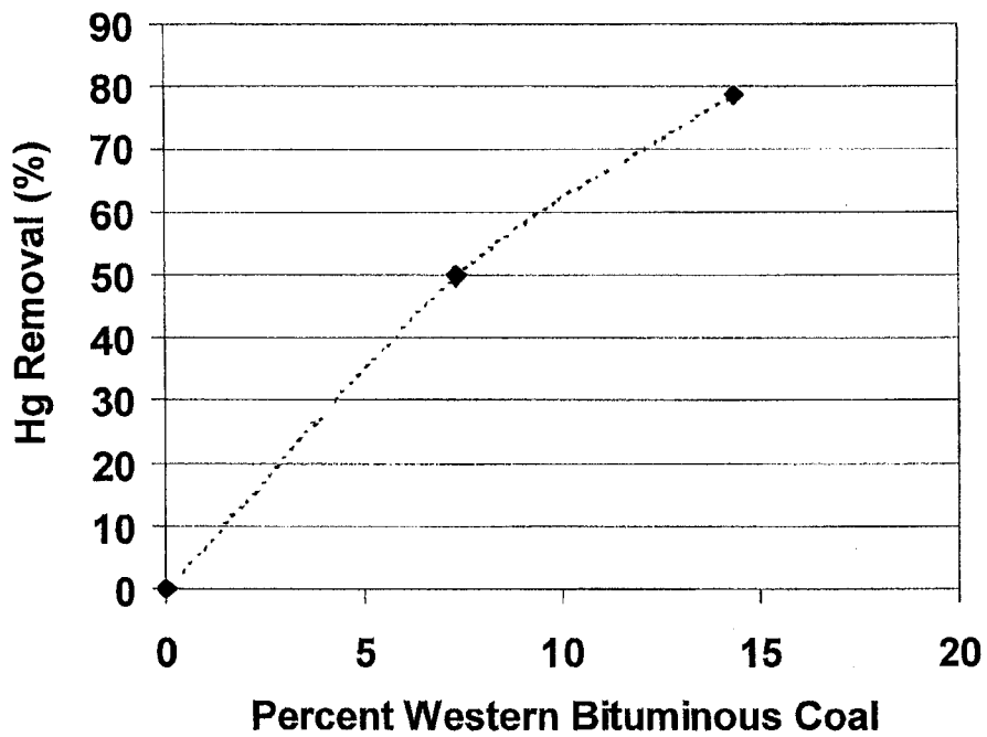
Figure 7. Results of Coal Blending Tests, Experiment #3
