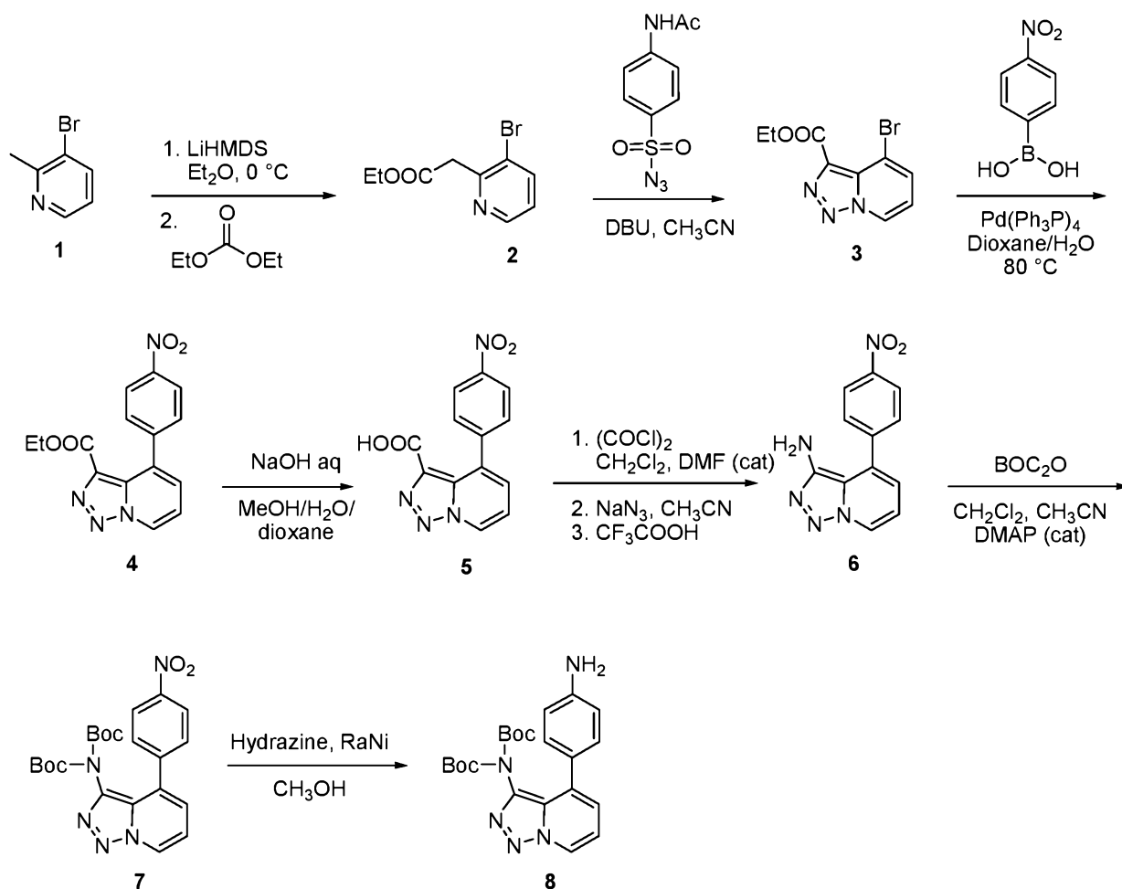
Scheme 1: Synthesis of Intermediate Compound 8.
