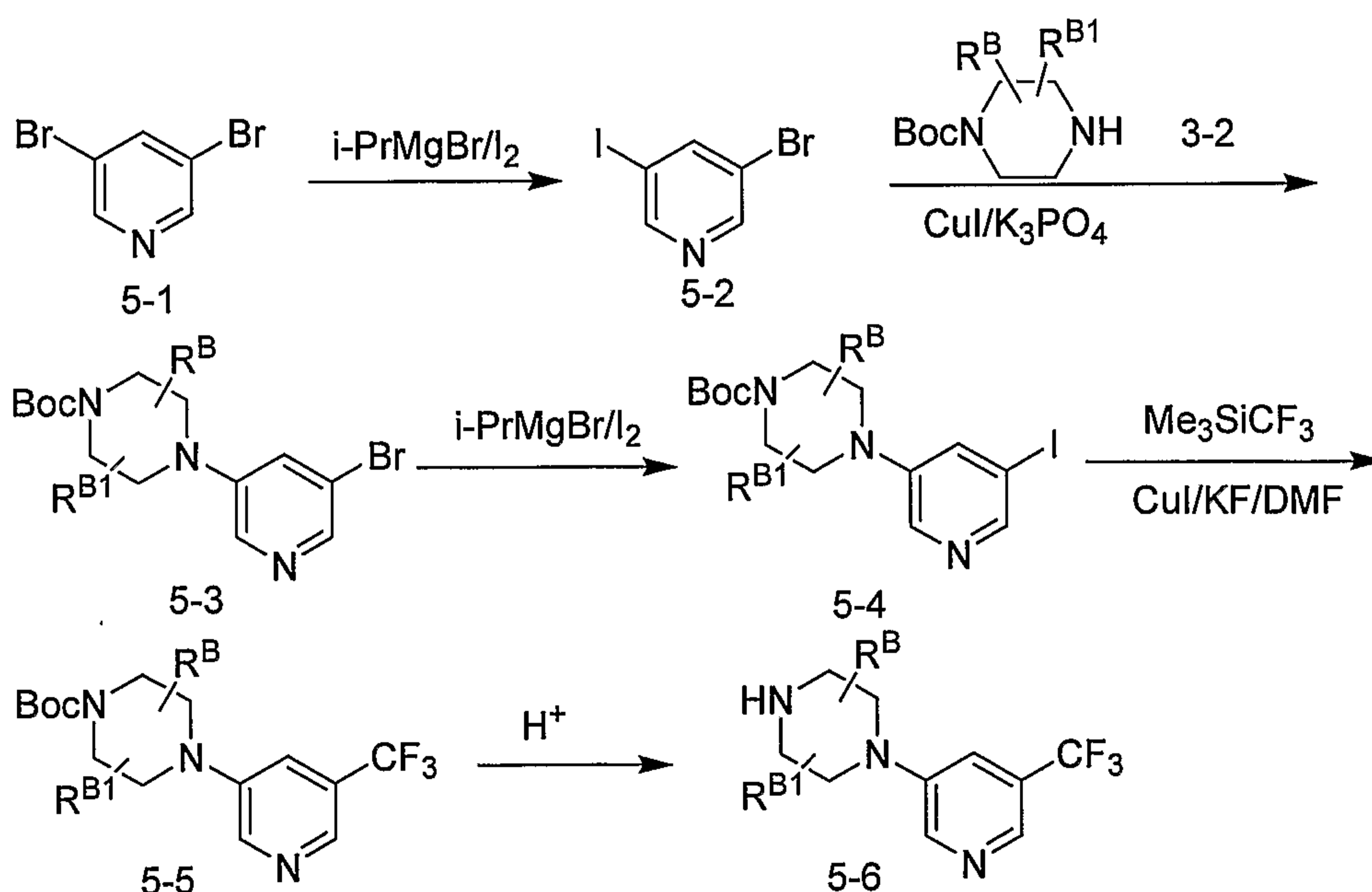
Scheme 5
