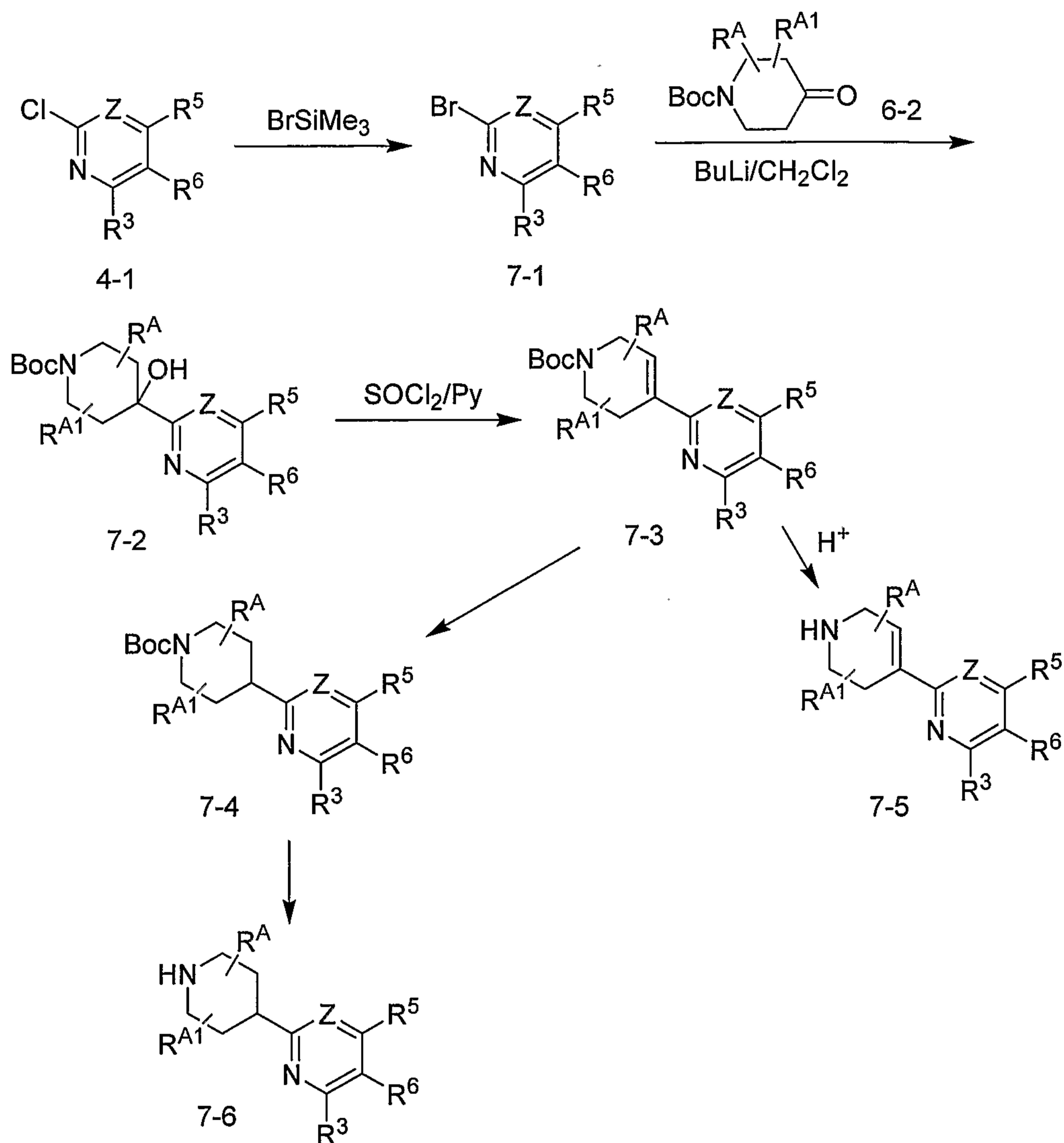
Scheme 7
