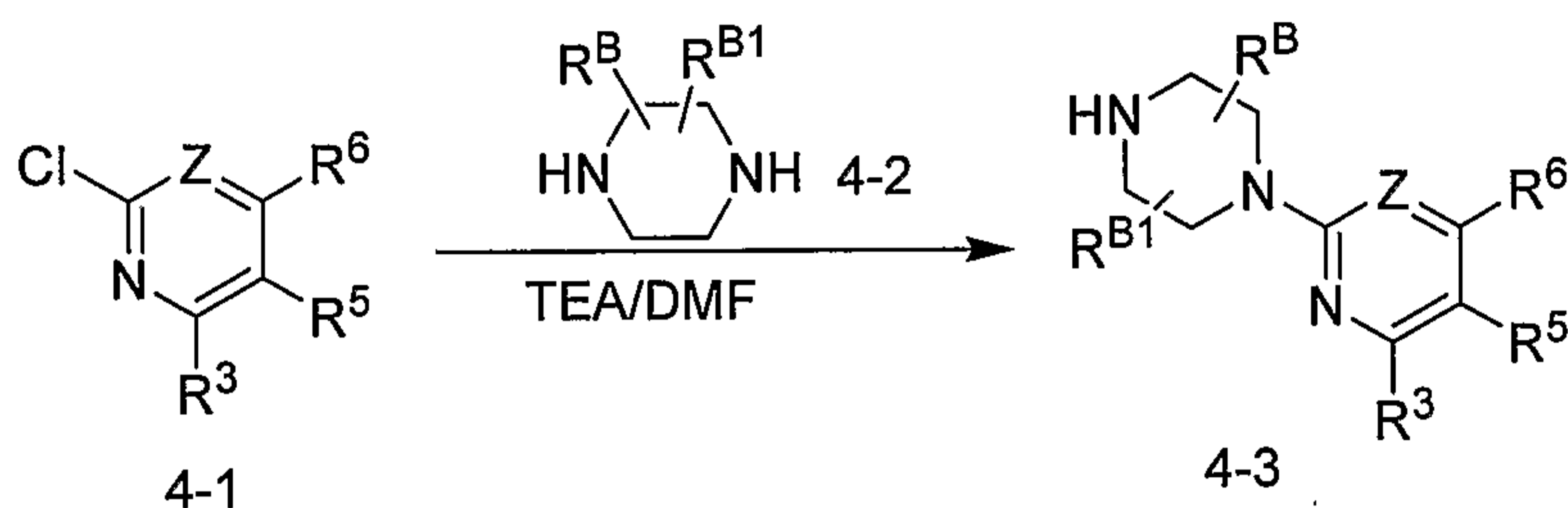
Scheme 4
