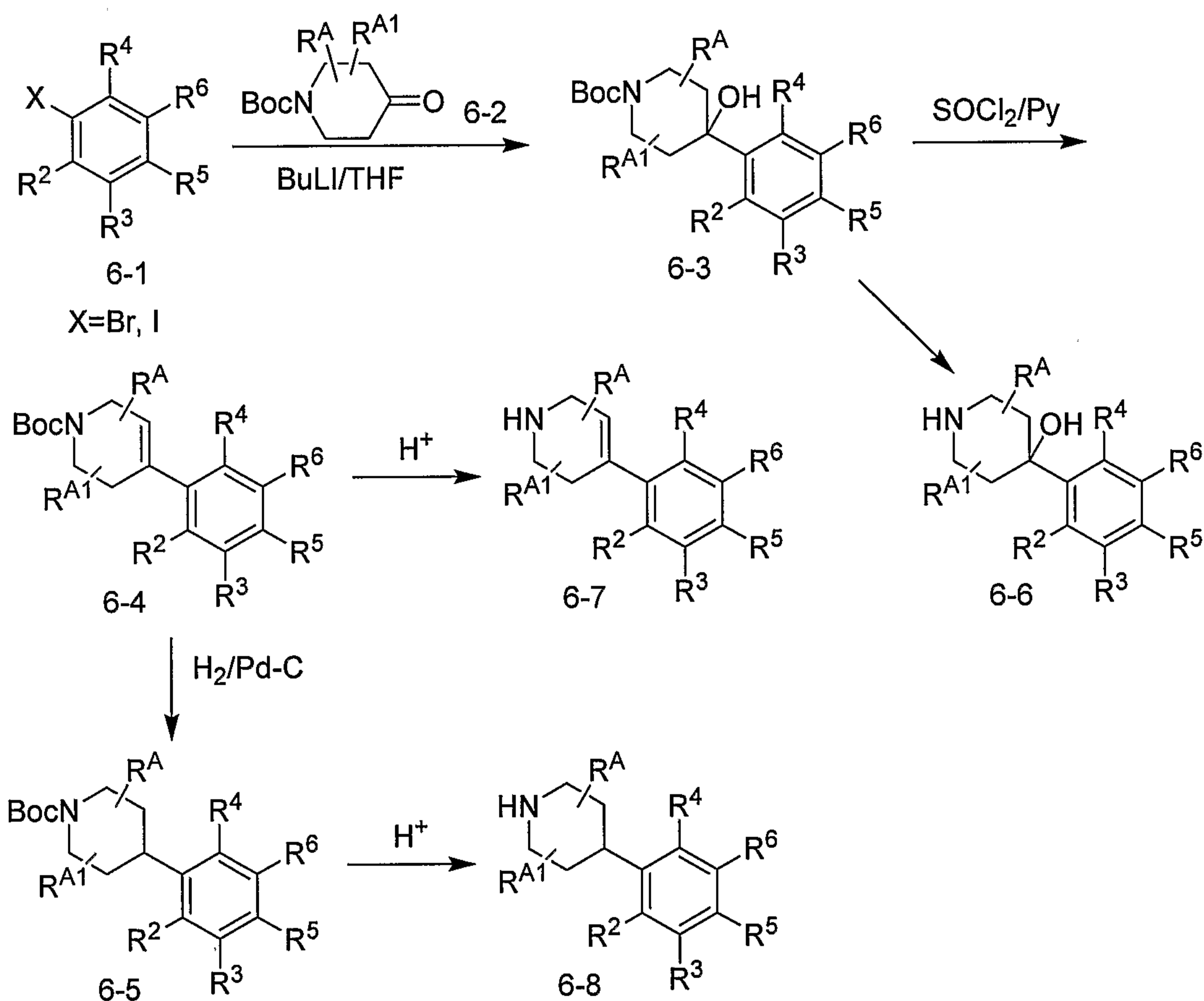
Scheme 6
