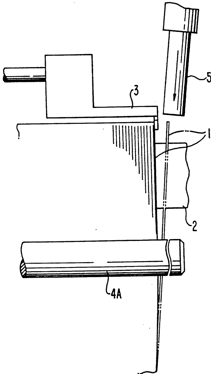
FIG. 16 (PRIOR ART)
