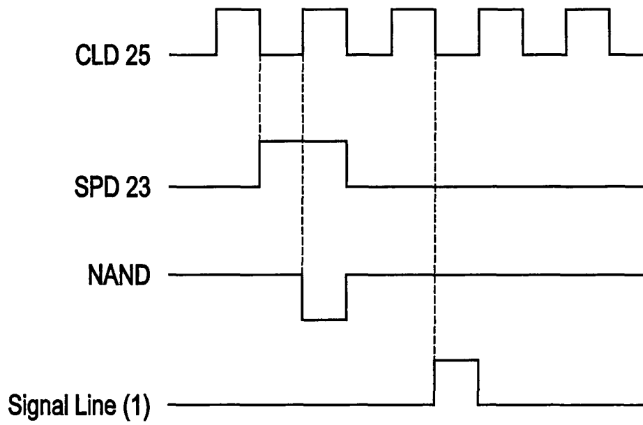
Timing Chart of Source Driver Circuit
