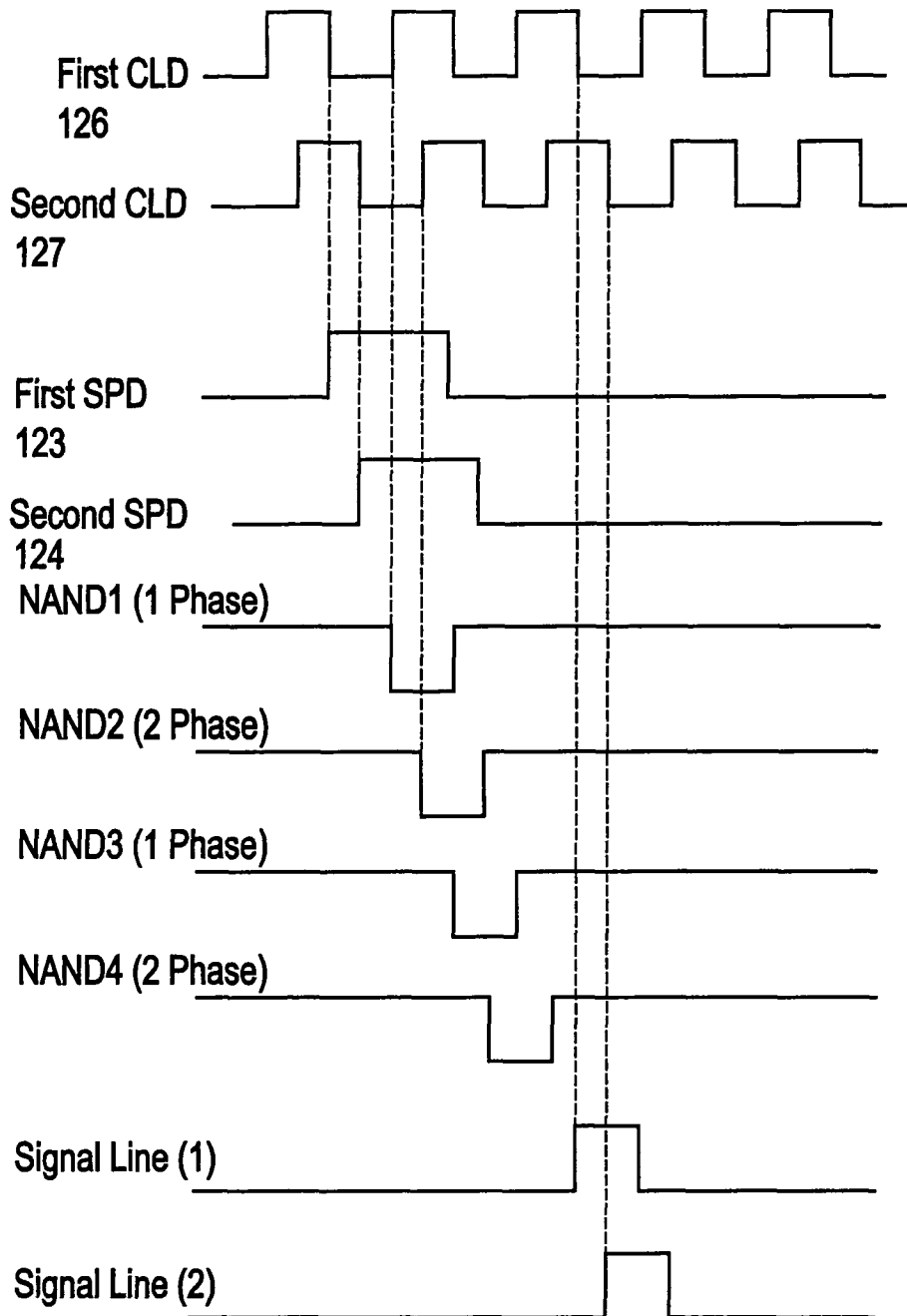
Timing Chart of Source Driver Circuit
