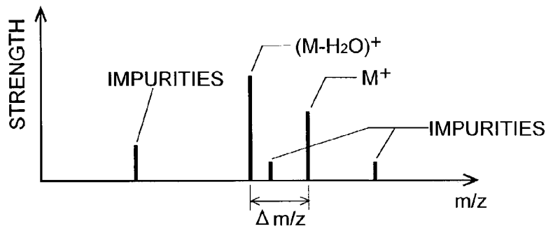
Fig. 3A MASS SPECTRUM BEFORE SELECT
