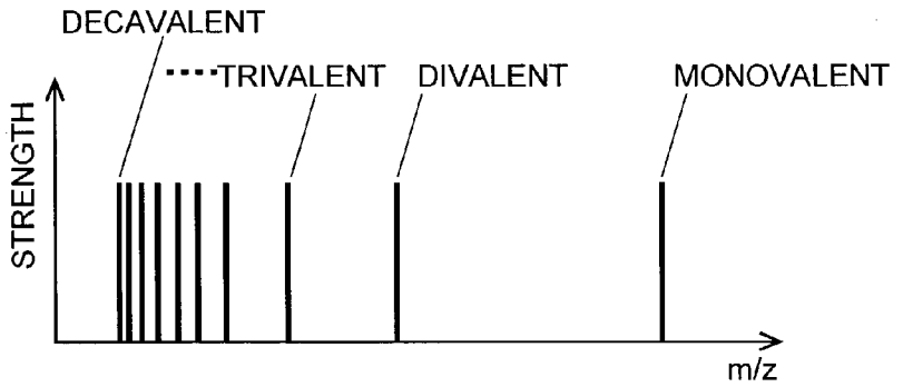
Fig. 4C MASS SPECTRUM AFTER SELECT
