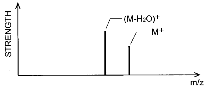
Fig. 3C MASS SPECTRUM AFTER SELECT
