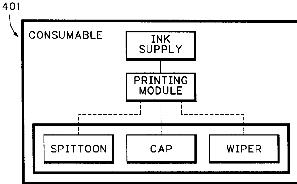
FLUIDIC BLOCK DIAGRAM
