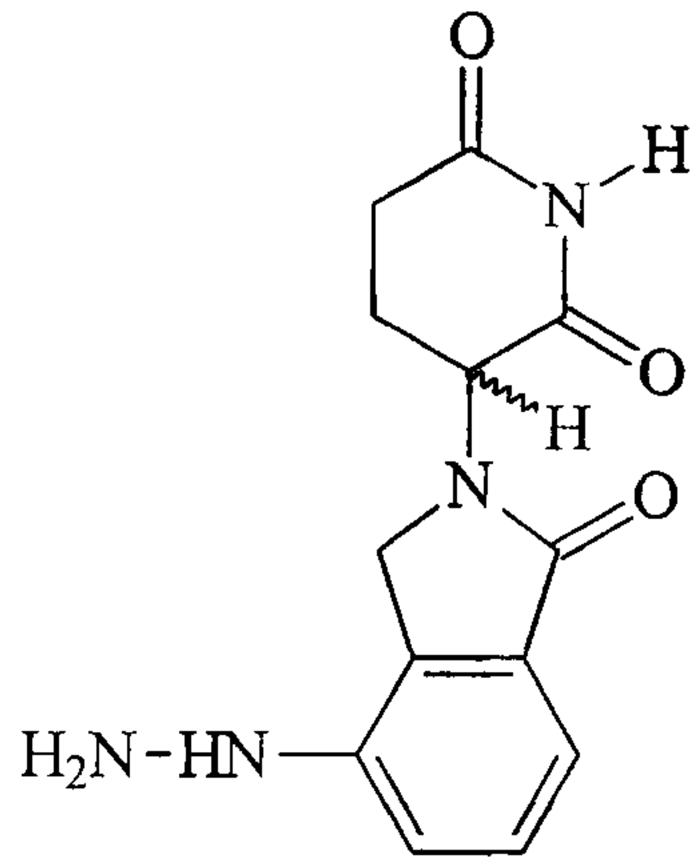
6-Hydrazino-EM-12
