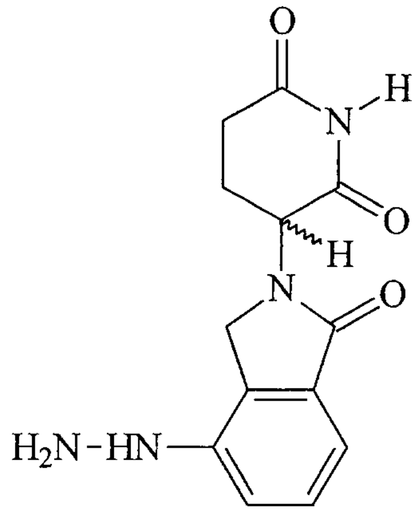
6-Hydrazino-EM-12
