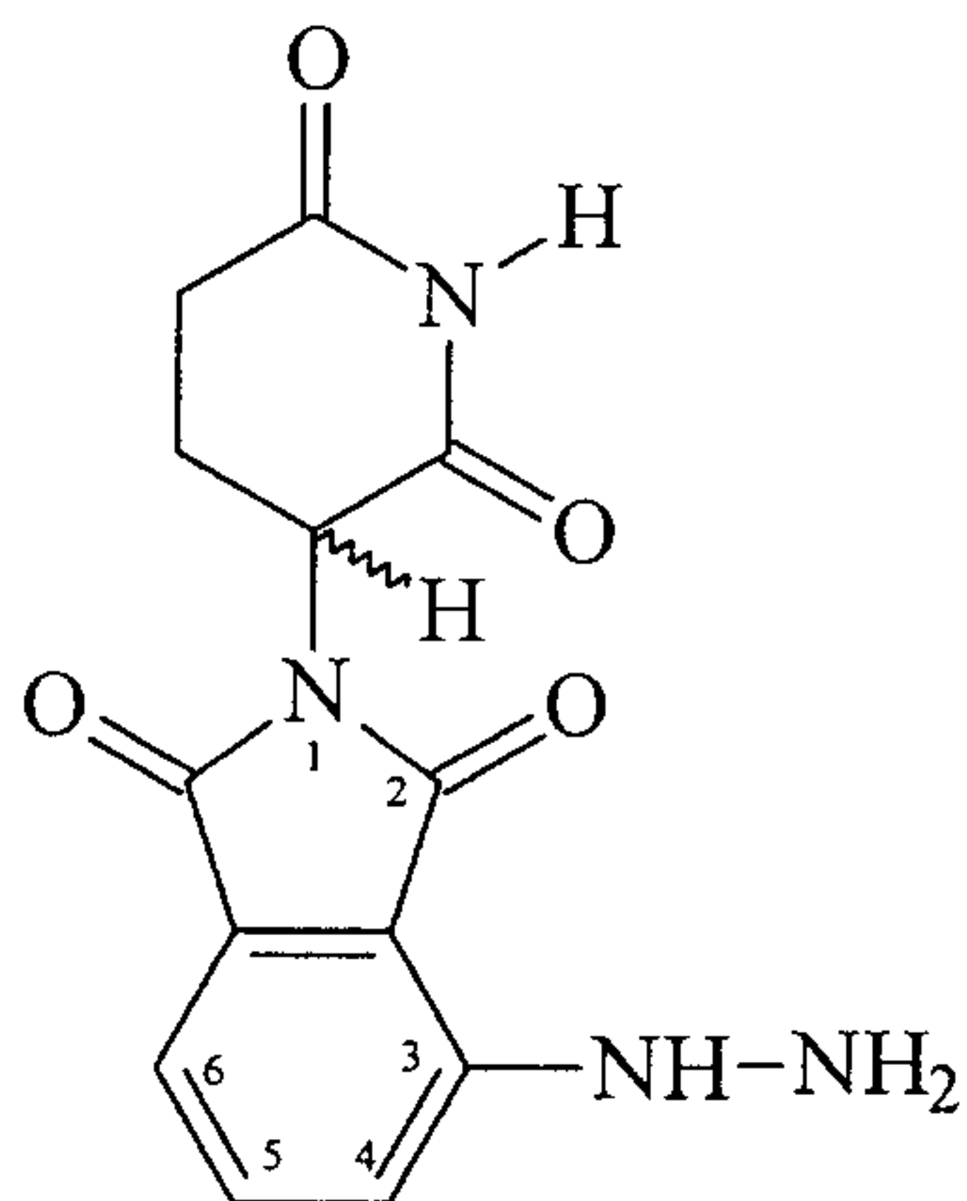
3-Hydrazino-Thalidomide
