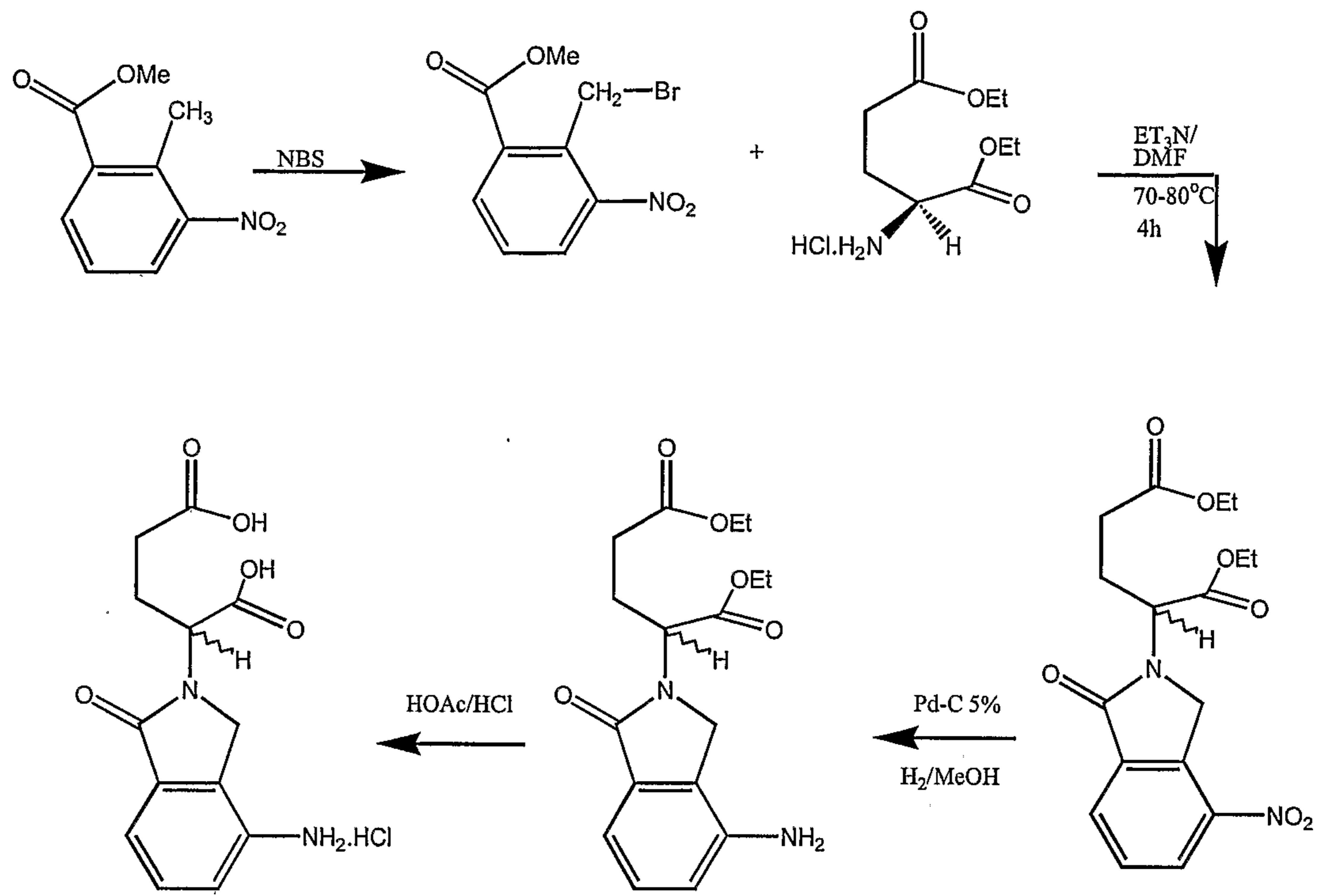
3-(4-aminophthalimidino)-glutaric acid.HCl
