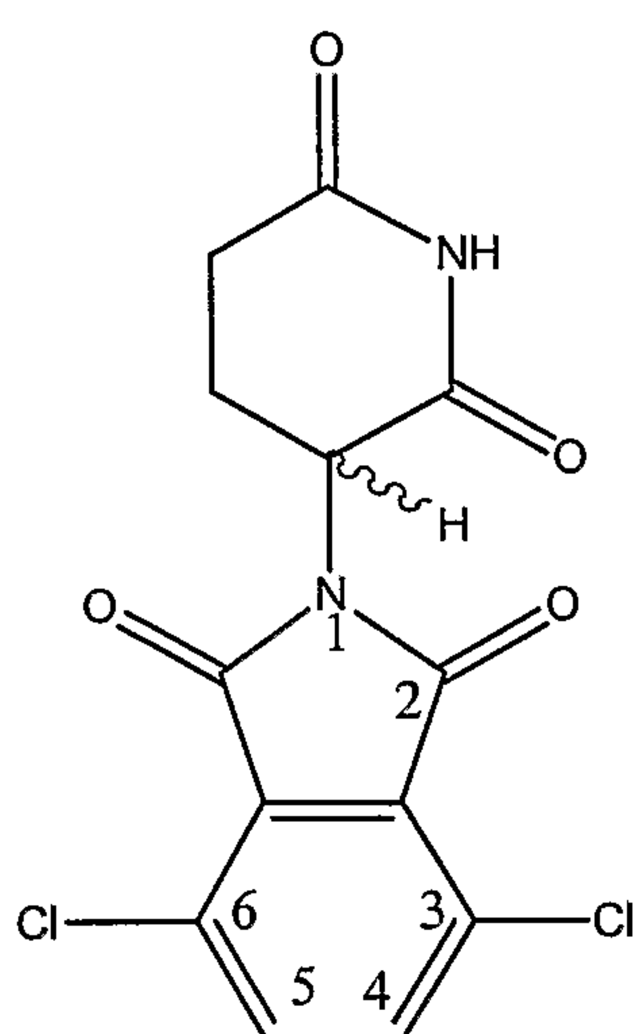
3, 6-Dichloro-thalidomide
