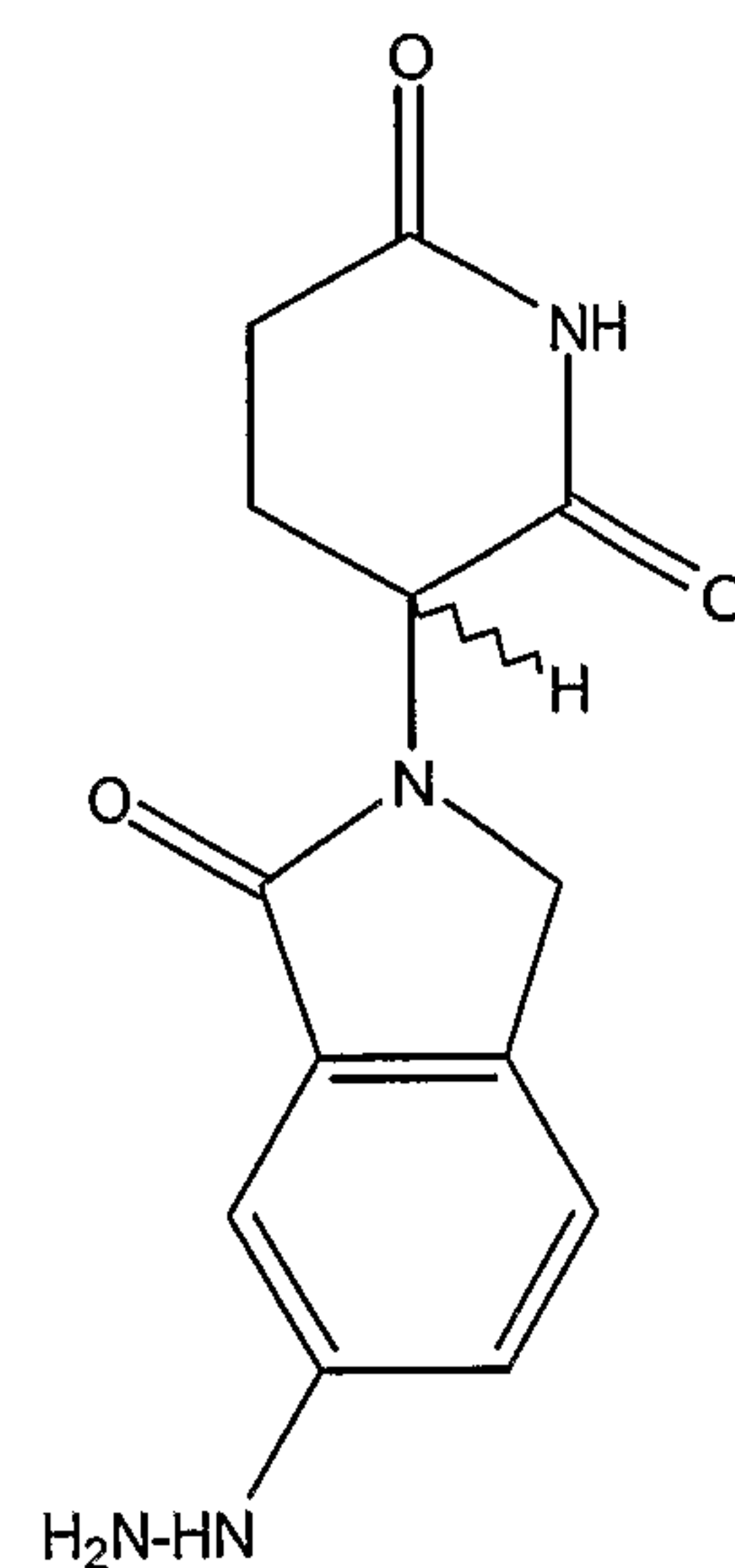
3-(6-hydradizephthalimidino)- glutarimide
