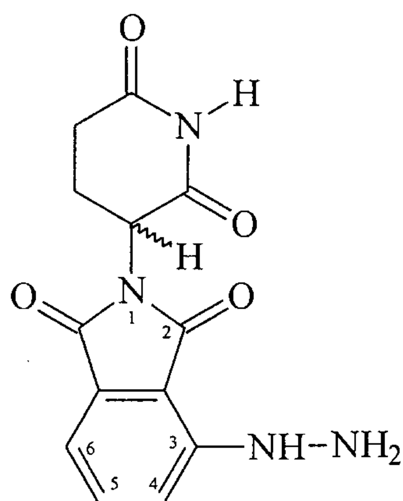
3-Hydrazino-Thalidomide
