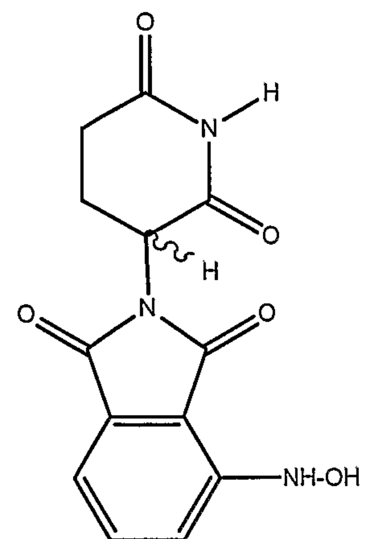
3-Hydroxylamino-Thalidomide
