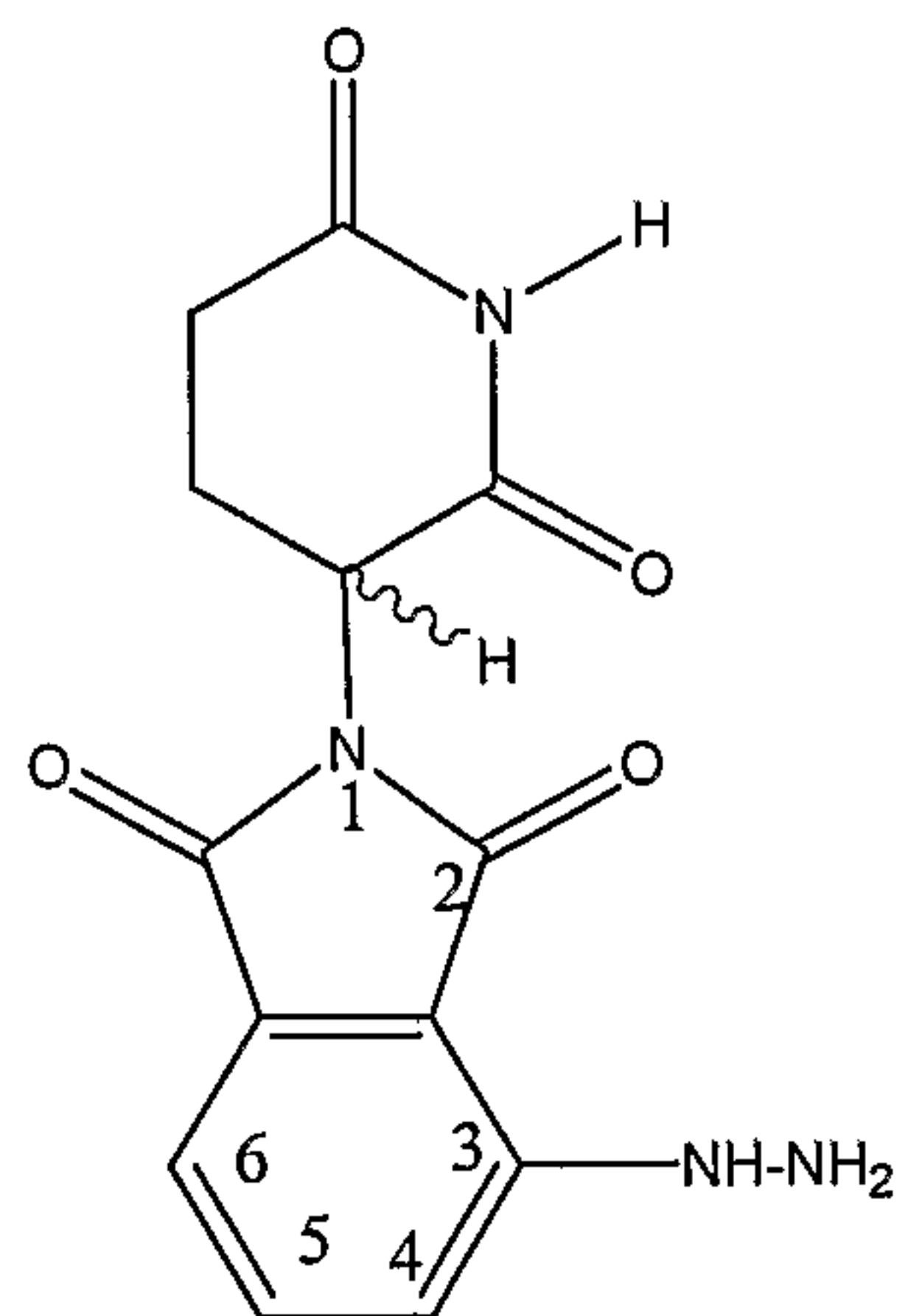
3-Hydrazino-Thalidomide
