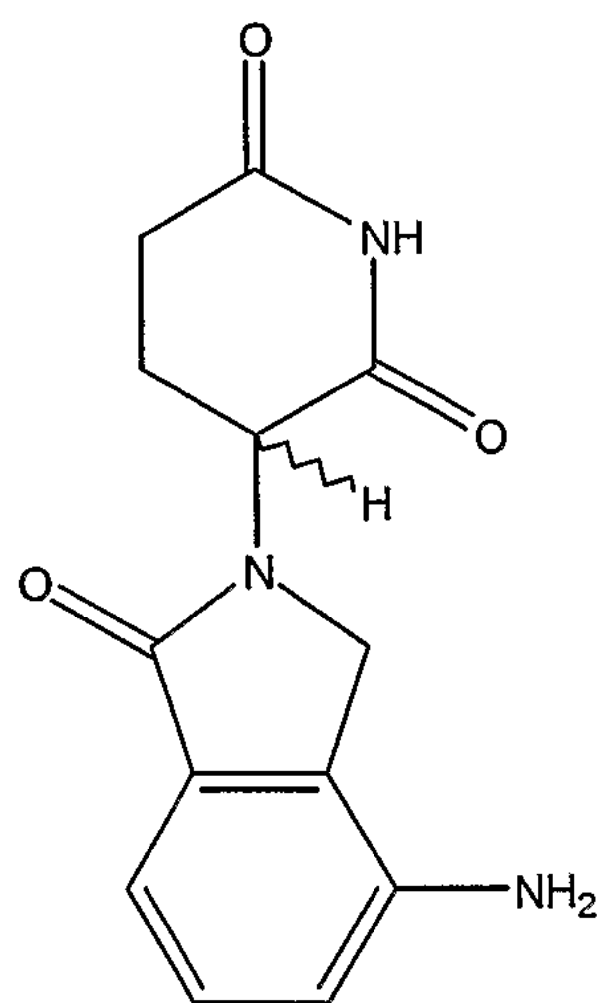
3-(4-amino-phthalimidino)- glutarimide
