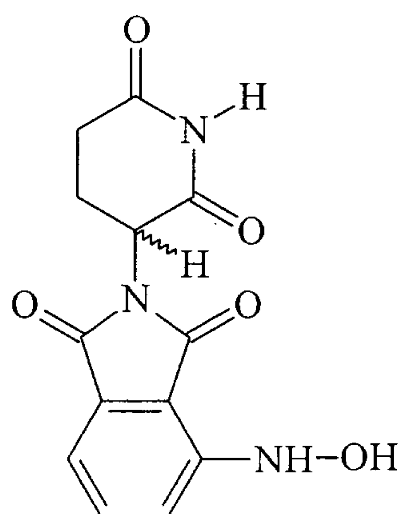
3-Hydroxylamino-Thalidomide
