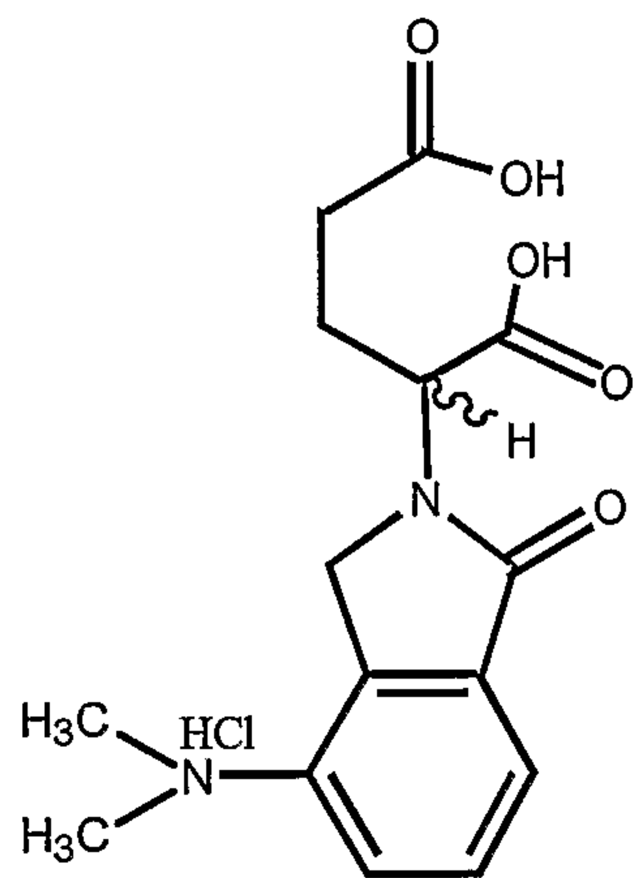
2-(6-dimethylamino-phthalimidino)-glutaric acid
