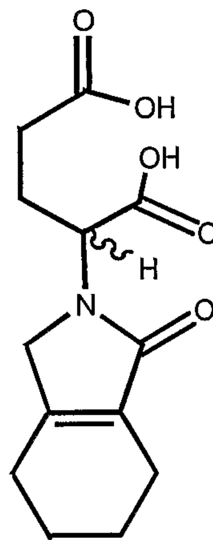
2-3,4,5,6-Tetrahydro-phthalimidino)-glutaric acid
