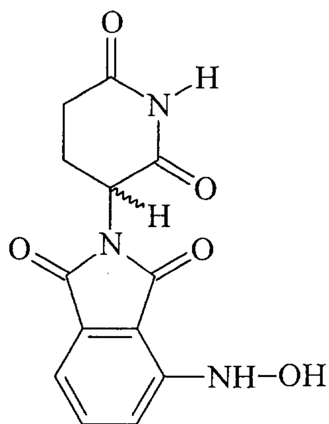
3-Hydroxylamino-Thalidomide
