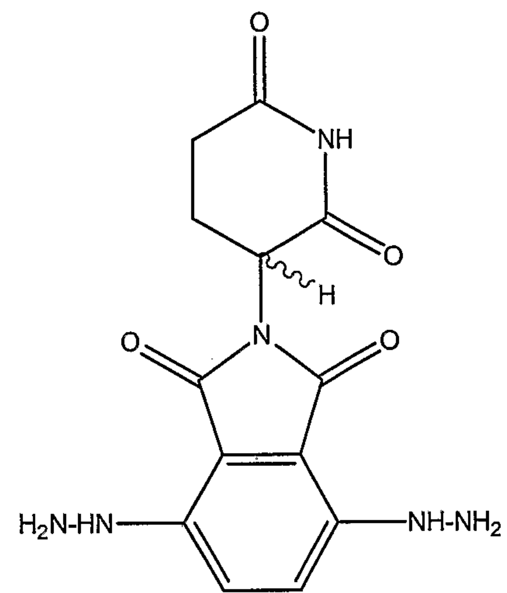
3, 6-Dihydrzino-thalidomide
