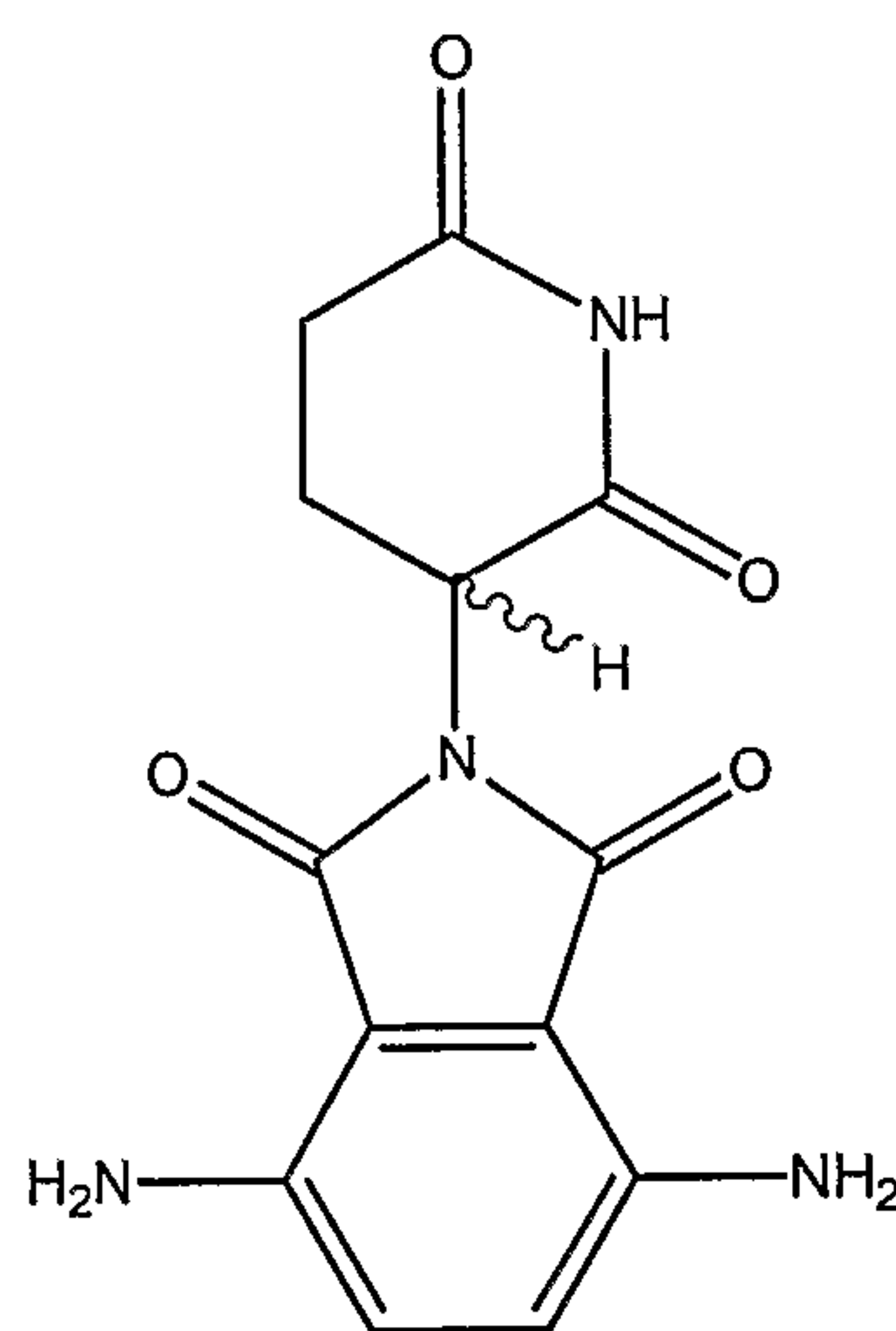
3, 6-Diamino-thalidomide
