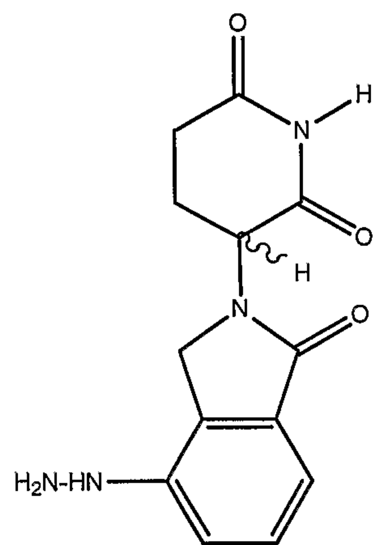
3-(4-Hydrazino-phthalimidino)-gluteramide
