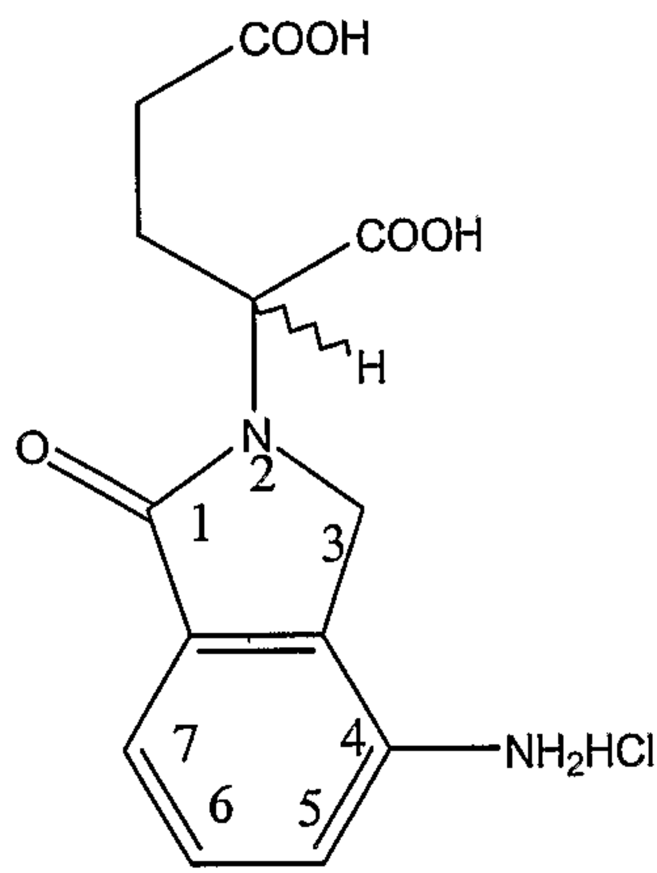
2-(4-amino-phthalimidino)- glutaric acid HCl
