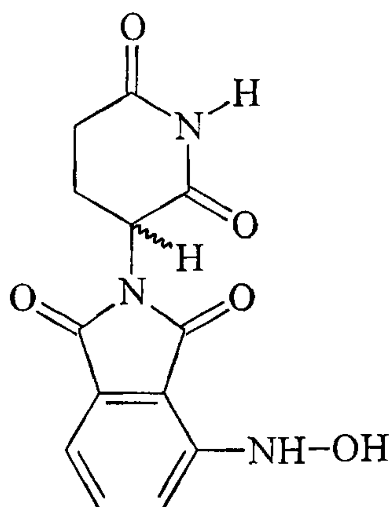
3-Hydroxylamino-Thalidomide
