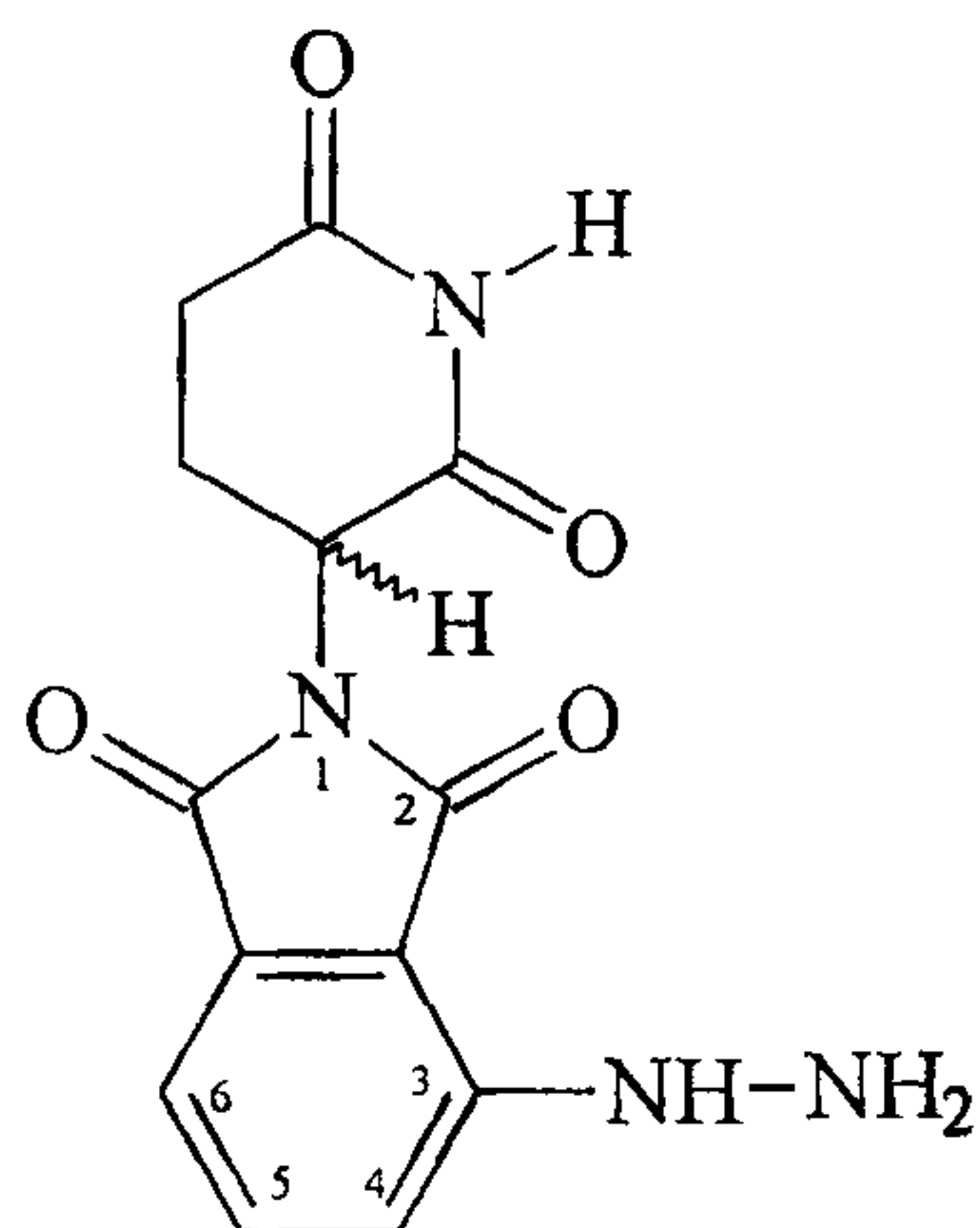
3-Hydrazino-Thalidomide
