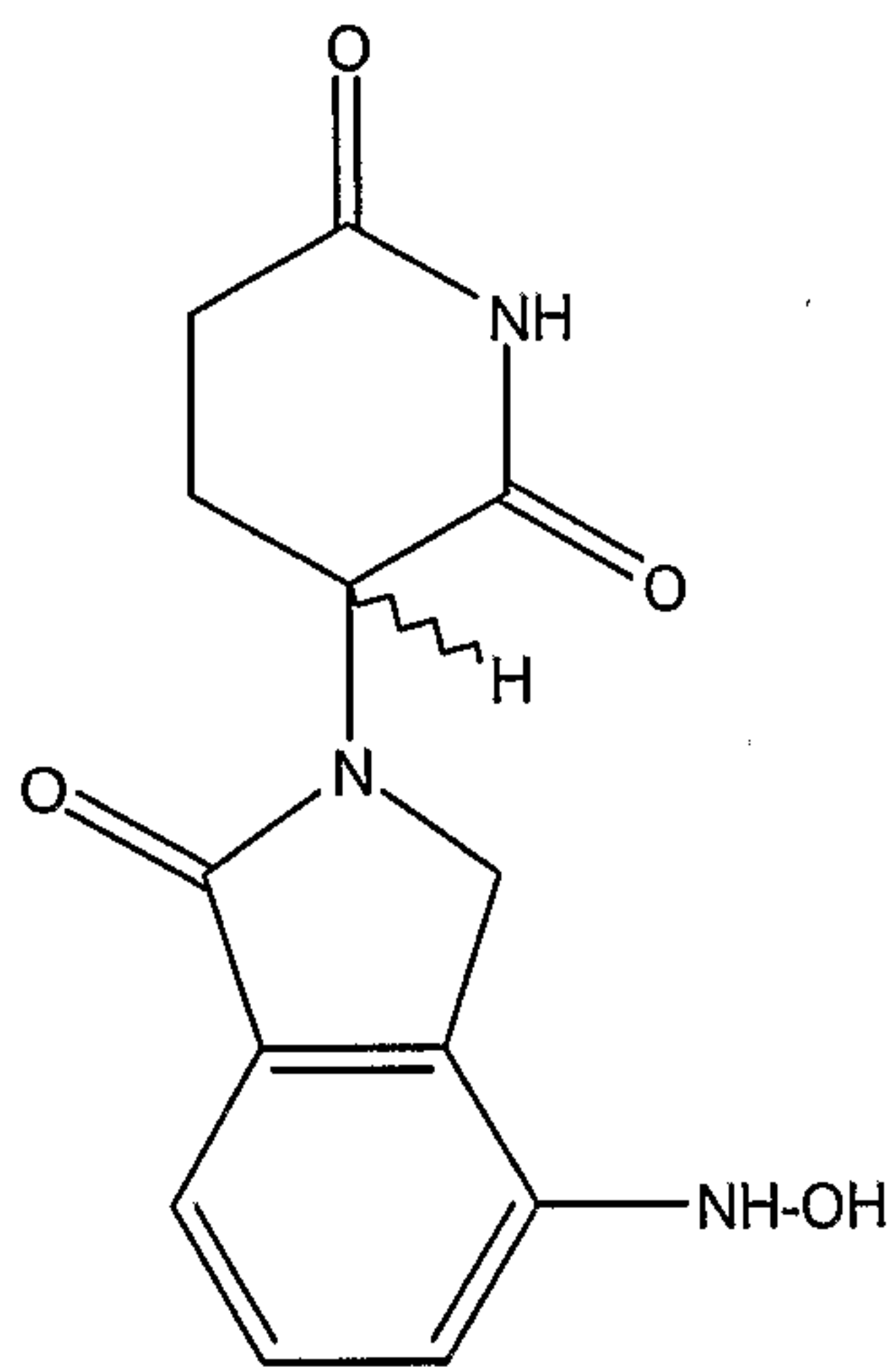
3-(4-Hydroxyaminephthalimidino)- glutarimide
