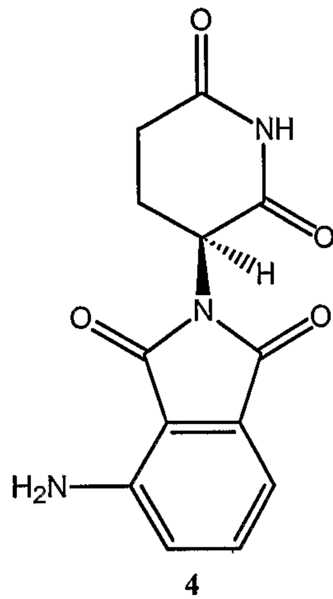
S(-)-3-amino-thalidomide
