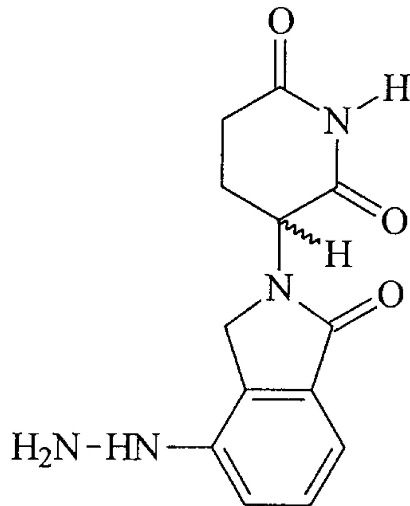
6-Hydrazino-EM-12
