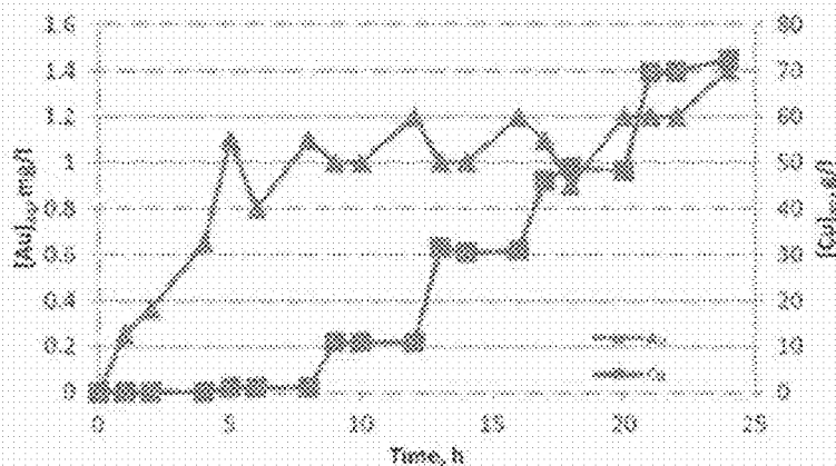
Figure 5. Gold concentration of the solution vs. copper concentration in test 3 of Example 2: [Cu] aq,0 =0-75 g/l, [NaBr] aq =100 g/l, [CaCl 2 ] aq,0 =177 g/l, pH=1.7, T=98°C, oxygen feed 2 l/min, and solid concentration 400 g/l.
