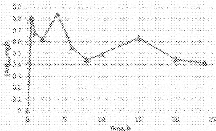
Figure 4. Gold concentration of the solution vs. leaching time in test 1 of Example 2: [Cu] aq,0 =100 g/l, [NaBr] aq =10-100 g/l, [CaCl 2 ] aq,0 =177 g/l, pH=1.7, T=98°C, oxygen feed 2 l/min, and solid concentration 200 g/l.
