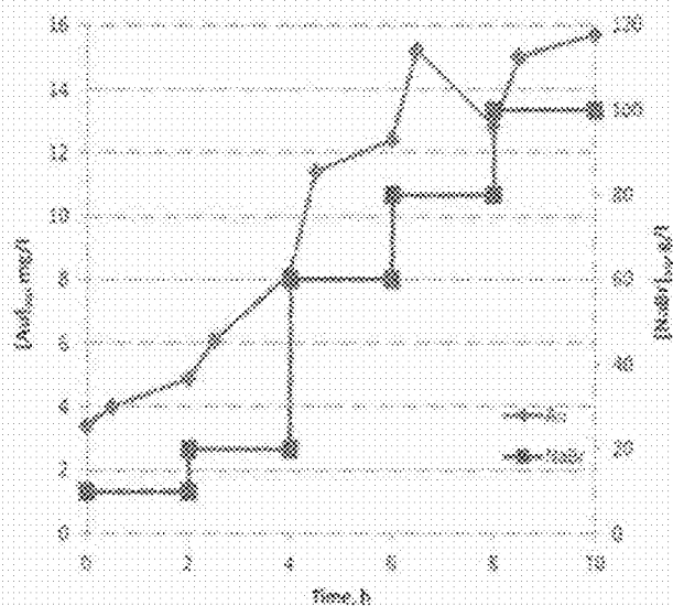
Figure 3. Gold concentration of the solution vs. bromide concentration in test 4 of Example 1: [Cu]_{sol,0}=100 g/l, [NaBr]_{sol,0}=10-100 g/l, [CaCl_2]_{sol,0}=177 g/l, acid concentration >10 g/l (HCl), T=98^\circ C , oxygen feed 220 ml/min, and solid concentration 200 g/l.
